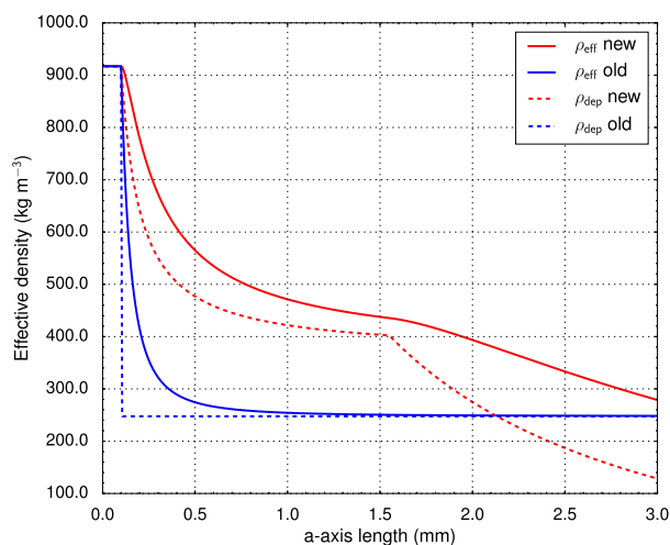
FIG. 1. Plot of deposition density (dashed lines) and effective density (solid lines) for a crystal at sizes from a = 0.01 to a = 3.0 using the deposition density model developed herein (red) and the deposition density model of Jensen and Harrington (2015), with a_c = 0.1 \text{ mm} and \rho_{dep} \approx 250 \text{ kg m}^{-3} (blue). The crystal structure quantities for the deposition density shown here are a_c = 0.1 \text{ mm} , f_b = 0.4 , f_i = 0.5 , and f_t = 0.3 .
