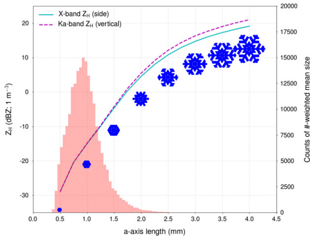
FIG. 8. Comparison of Z given 1 \text{ m}^{-3} crystals growing from a = 0.5 \text{ mm} to a = 4.0 \text{ mm} for X band at side incidence (solid cyan line; corresponding to X-SAPR) and Ka band at vertical incidence (dashed magenta line; corresponding to KAZR). The 2D ice crystal structures used in the Amsterdam discrete dipole approximation (ADDA; Yurkin and Hoekstra 2011) calculations are plotted in blue. An overlay of the histogram of number-weighted mean a -axis lengths from the MCMC simulations is plotted in red.
