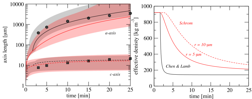
FIG. 3. Particle a - and c -axis lengths as a function of time for dendrites grown in a wind tunnel at liquid saturation and at -15^\circ\text{C} (black solid circles; Fukuta and Takahashi 1999). Simulated a - and c -axis lengths are shown with the solid and dashed lines, respectively. The black curves use the deposition density from Chen and Lamb (1994) whereas the red curves use the deposition densities from Fig. 1 above and an initial particle radius of 5 \mu\text{m} . The black and red shaded regions show the range of solutions for initial particle radius from 1 to 10 \mu\text{m} . (left) The effective particle density as a function of time for Chen and Lamb (1994) (black lines) and using our density functions (red lines) with two initial radii shown. The parameters we use here for our deposition density function are a_c = 0.01 , f_b = 0.2 , f_i = 0.2 , and f_t = 0.2 .
