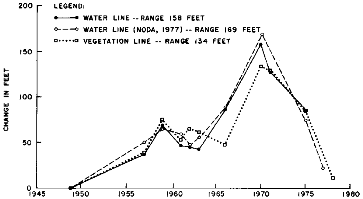
FIG. 7 Historic changes in the water line and vegetation line for Kailua Beach Park.
