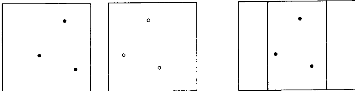
FIG. 1 Selecting photographs with a minimum of tilt. Case 1: Either or both of the photographs are tilted. Case 2: Photographs of different scale-no tilt. Case 3: Photographs of the same scale-neither are tilted.
