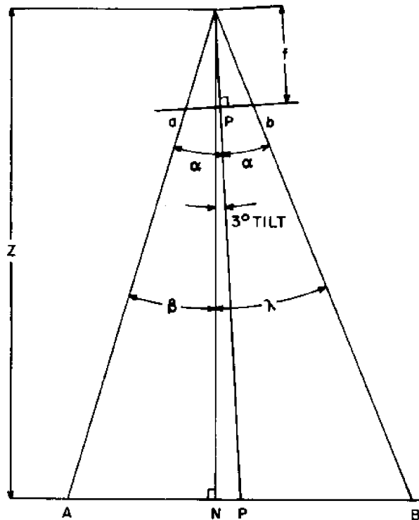
FIG. 5 Tilt on a photograph. For the vertical photograph, the computed distance between AB is 4036.2 feet. On a photograph with a 3^\circ tilt, this distance is computed as 4,049.0 feet. The error is (12.8/4,036.2)(100) = .3\% (Adapted from Scherz, 1974).
