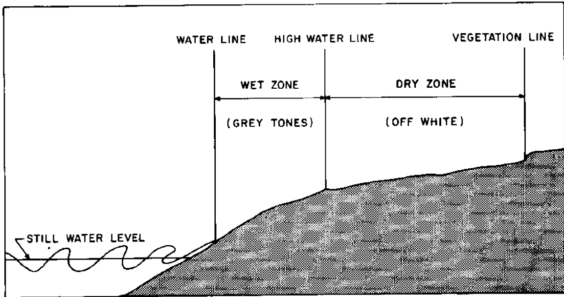
FIG. 3 Beach index lines, (Weber, 1969).
