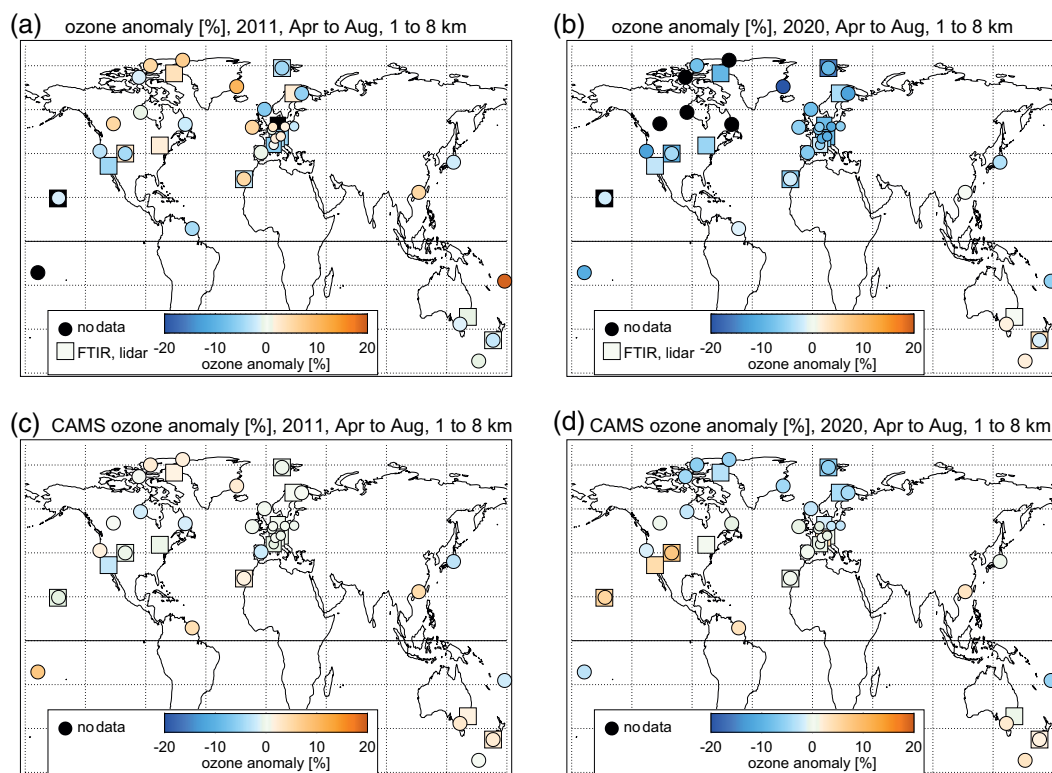
Figure 5. Geographic distribution of observed tropospheric ozone anomalies (averaged over the months April to August, and over altitudes from 1 to 8 km) for the years (a) 2011 and (b) 2020. Panels (c) and (d): same, but for CAMS results at the station locations. Colored circles give the anomaly at the ozonesonde stations. Squares are for FTIR and lidar stations. Black filling indicates insufficient data in the given year. CAMS, Copernicus Atmosphere Monitoring Service; FTIR, Fourier Transform Infrared Spectrometers.
