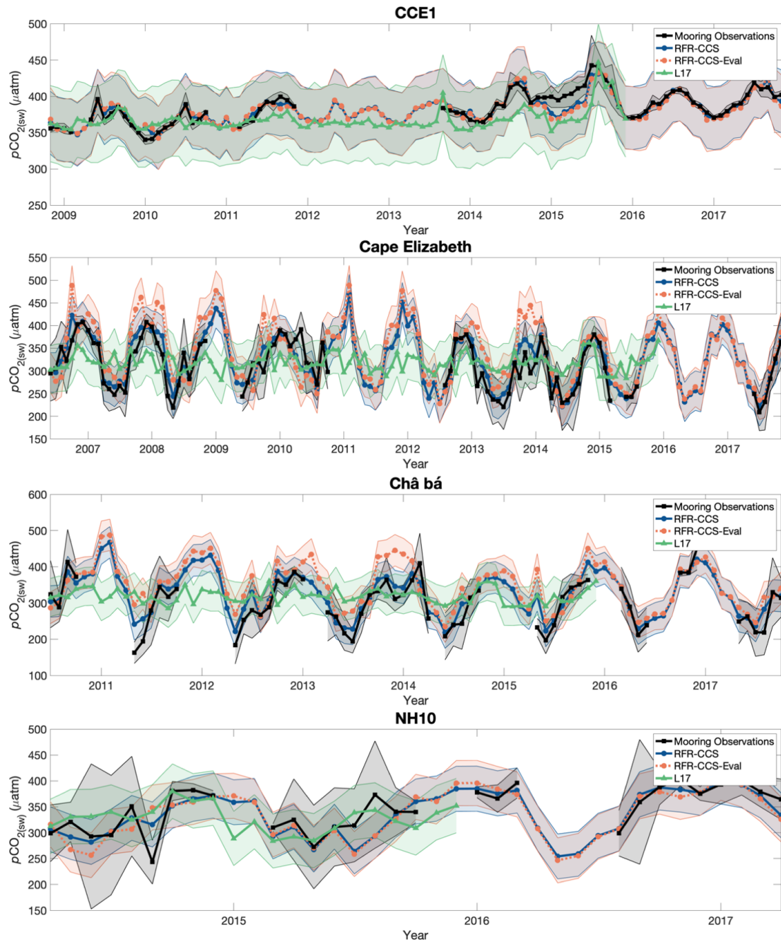
Figure B3. Like Fig. 2 in the main text, showing monthly values of p\text{CO}_{2(\text{sw})} from mooring observations (black), RFR-CCS (blue), the mooring-excluded RFR-CCS-Eval model (orange), and L17 (green). The envelopes around the black lines equal the standard deviations of all mooring observations within each month, representing the natural variability of the 3-hourly mooring measurements; the envelopes around the blue and orange lines represent the RFR-CCS and RFR-CCS-Eval results plus 1 standard uncertainty (43.6 \mu\text{atm} ; Sect. 3.5); the envelopes around the green lines represents the L17 data product plus the RMSE of an independent data evaluation in the province most closely associated with the mooring locations (52.5 \mu\text{atm} ; Table 3 of Laruelle et al., 2017; Province P7).
