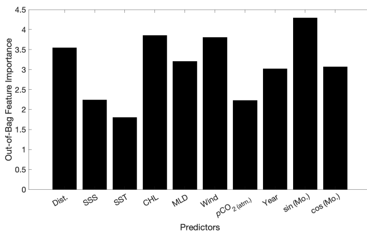
Figure B2. Predictor variable feature importances calculated for the random forest regression model fit used to produce RFR-CCS (Sharp et al., 2022; https://doi.org/10.5281/zenodo.5523389 ).
