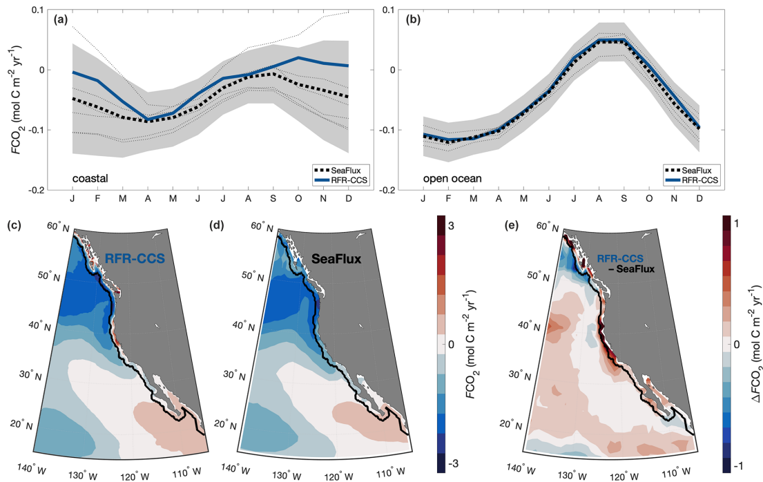
Figure 8. Monthly \text{CO}_2 flux per unit area for the nearshore coastal (a) and open-ocean (b) portions of the RFR-CCS domain calculated from the SeaFlux ensemble average (dotted black line; individual products in thin dotted lines) and from RFR-CCS (solid blue line). The grey shaded area represents variability in SeaFlux p\text{CO}_{2(\text{sw})} products calculated as plus and minus 1 standard deviation. Also shown is the spatially distributed \text{CO}_2 flux per unit area calculated from RFR-CCS (c) and from SeaFlux (d), as well as the difference between them (e). Red in panels (c) and (d) indicates net release of \text{CO}_2 to the atmosphere, whereas blue indicates net uptake of \text{CO}_2 ; in panel (e), red indicates where the RFR-CCS \text{CO}_2 flux per unit area is greater and blue where the SeaFlux \text{CO}_2 flux per unit area is greater. The solid black line denotes the boundary between the nearshore coastal (a) and open ocean (b) calculated as 100 km from the coast. All calculations are performed using ERA5 winds and an identical gas exchange coefficient ( \Gamma_{660} = 0.276 ).
