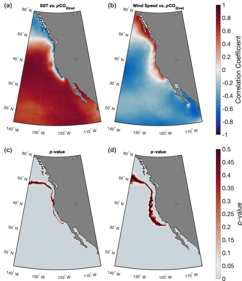
Figure B5. Correlations (a, b) and the p values of those correlations (c, d) in each grid cell of RFR-CCS between p\text{CO}_2 (sw) and SST (a, c) and between p\text{CO}_2 (sw) and wind speed (b, d).
