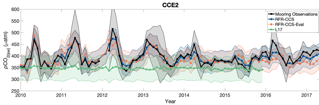
Figure 2. Monthly values of p\text{CO}_2(\text{sw}) from mooring observations (black), RFR-CCS (blue), the mooring-excluded RFR-CCS-Eval model (orange), and L17 (green). The envelope around the black line equals the standard deviation of all mooring observations within each month, representing the natural variability of the 3-hourly mooring measurements; the envelopes around the blue and orange lines represent the RFR-CCS and RFR-CCS-Eval results plus 1 standard uncertainty (43.6 \mu\text{atm} ; Sect. 3.5); the envelope around the green line represents the L17 data product plus the RMSE of an independent data evaluation in the province associated with CCE2 (52.5 \mu\text{atm} ; Table 3 of Laruelle et al., 2017; Province P7).
