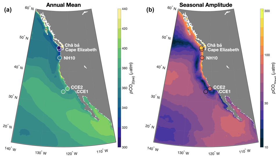
Figure 6. Annual mean p\text{CO}_2(\text{sw}) (a) and the seasonal amplitude of p\text{CO}_2(\text{sw}) (b) from RFR-CCS. Also shown are annual mean p\text{CO}_2(\text{sw}) and the seasonal amplitude of p\text{CO}_2(\text{sw}) measured at ocean mooring locations.
