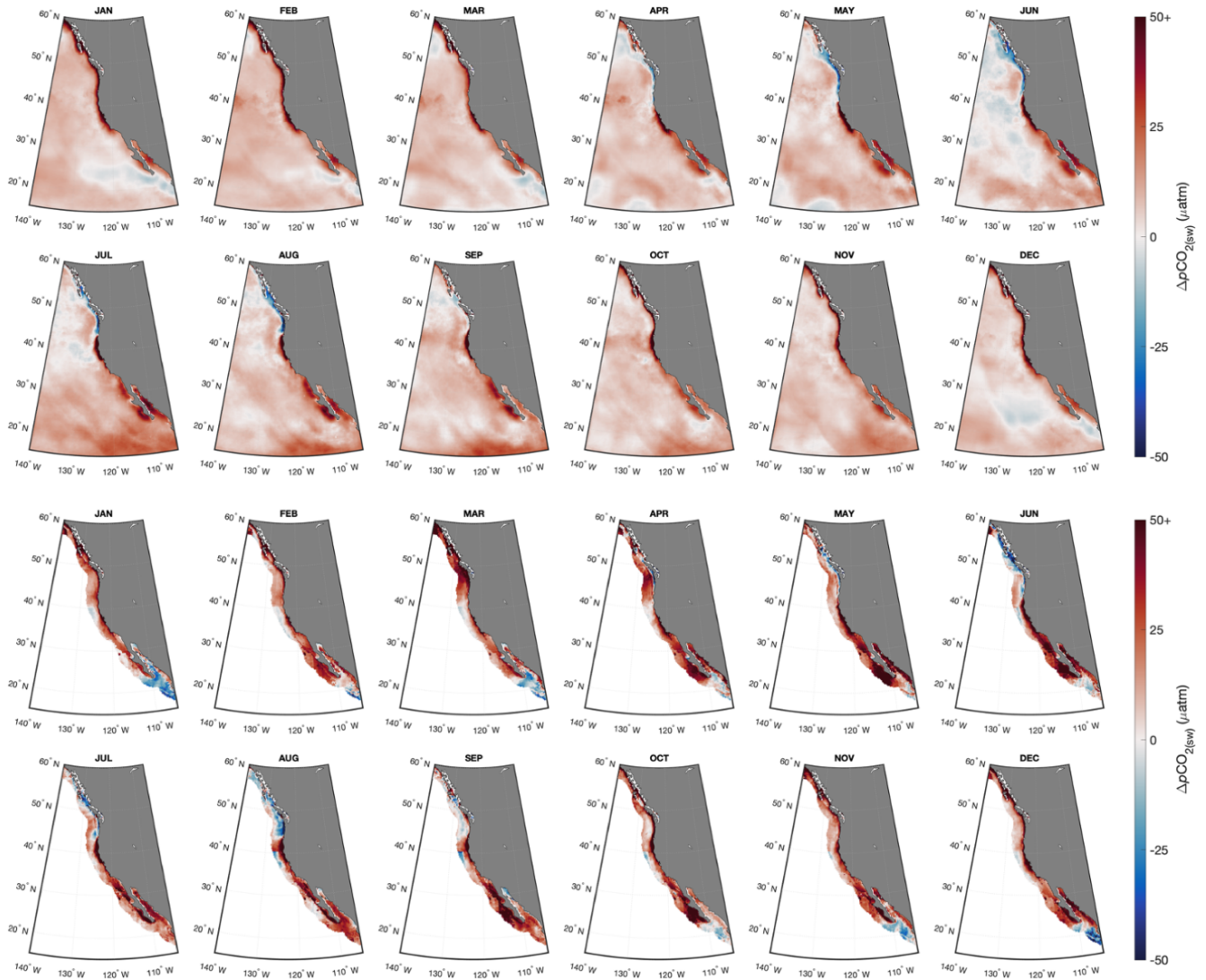
Figure B4. Monthly mean differences in p\text{CO}_2(\text{sw}) values between RFR-CCS-clim and L20 (top) and between RFR-CCS-clim and L17 (bottom).
