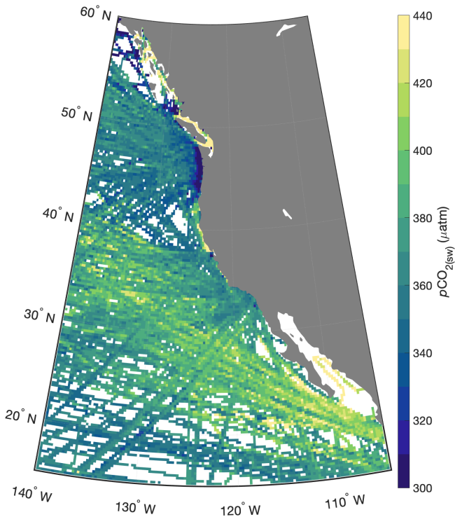
Figure 1. Annual mean p\text{CO}_2(\text{sw}) from the 0.25^\circ resolution gridded dataset computed as an average over the monthly climatology from 1998 to 2020 for each grid cell. The two extremes of the color bar can represent p\text{CO}_2(\text{sw}) values less than or greater than the color bar limits; the chosen range represents most of the values and emphasizes regional contrast.
