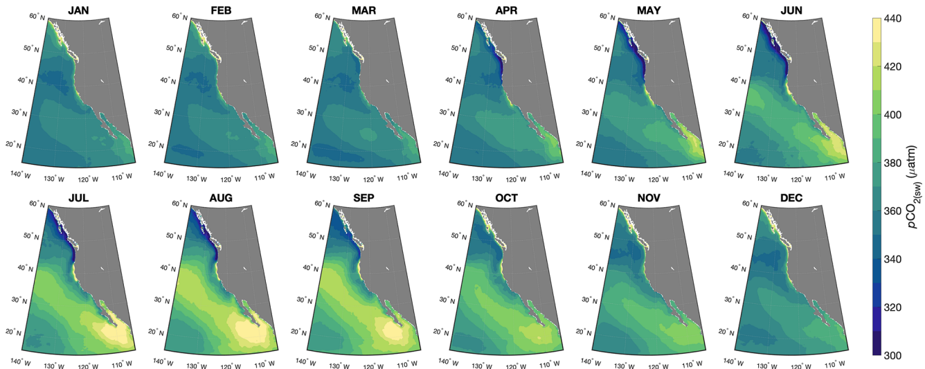
Figure 7. Monthly mean p\text{CO}_2(\text{sw}) fields from RFR-CCS.
