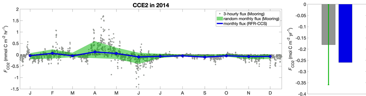
Figure 9. Hourly flux of \text{CO}_2 across the air-sea interface ( F_{\text{CO}_2} ) calculated from 3-hourly mooring observations (grey), monthly values from RFR-CCS (blue), and the 1-standard-deviation envelope of a Monte Carlo analysis ( n = 100\,000 ) whereby one randomly selected 3-hourly mooring observation from each month is selected to represent that month (green). The bar chart on the right gives annual F_{\text{CO}_2} based on 3-hourly mooring observations ( -0.18 \text{ mol C m}^{-2} \text{ yr}^{-1} ) and RFR-CCS ( -0.26 \text{ mol C m}^{-2} \text{ yr}^{-1} ), along with the uncertainty in annual F_{\text{CO}_2} from mooring measurements based on the Monte Carlo analysis ( -0.00 to -0.36 \text{ mol C m}^{-2} \text{ yr}^{-1} ).
