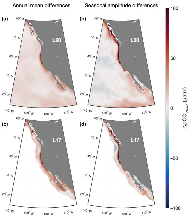
Figure 3. Differences between annual means (a, c) and seasonal amplitudes (b, d) of p\text{CO}_2(\text{sw}) from RFR-CCS-clim versus the L20 climatology (a, b; RFR-CCS-clim – L20) and versus a climatological average of the L17 product (c, d; RFR-CCS-clim – L17).
