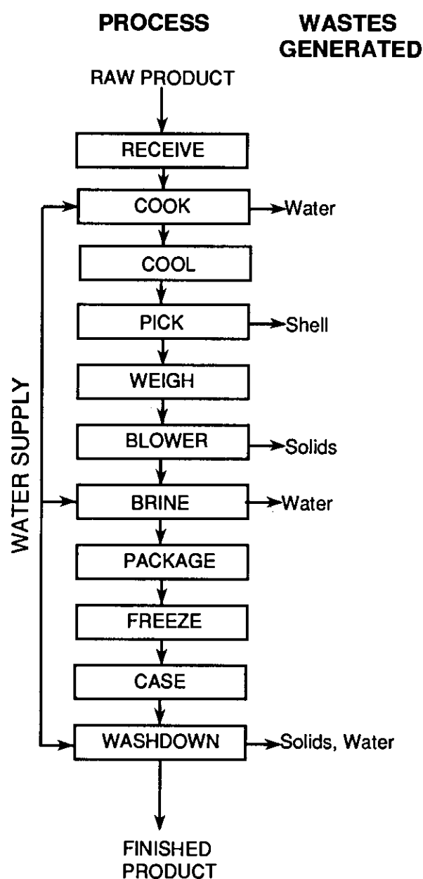
Figure 5.2 Process Flow of Waste Generated from a Hand Pick Shrimp Processing Plant (19).
