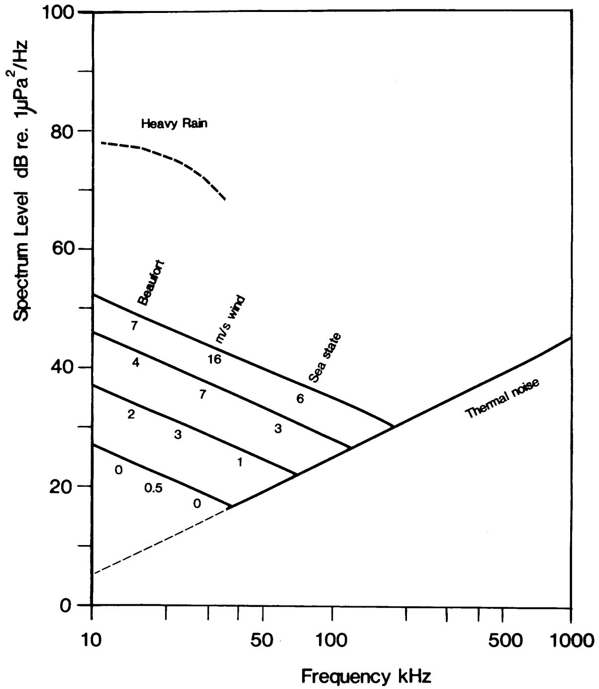
Figure 5. Ambient sea noise spectra.
