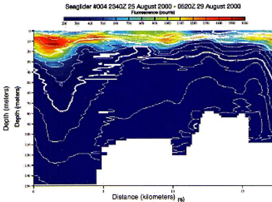
Figure 15. (A) Autonomous instrument-equipped Seaglider deployed by Erikson and Perry. (B) Track occupied by Seaglider superimposed on bathymetric map of Monterey Bay, California. (C) Horizontal and vertical distribution of chlorophyll from fluorometer mounted on Seaglider.
