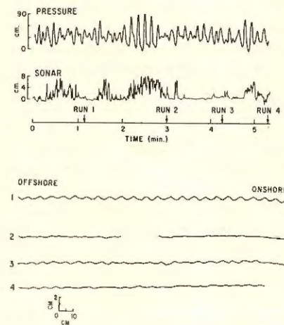
Figure 3. Field measurements of the generation and disappearance of sand ripples by wave action in water 3.4 meters deep off Scripps Pier.
