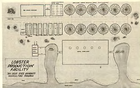
Figure 2.—Diagrammatic representation of a 100-foot diameter "care-O-cell" capable of rearing 8,000 lobsters to market size.
