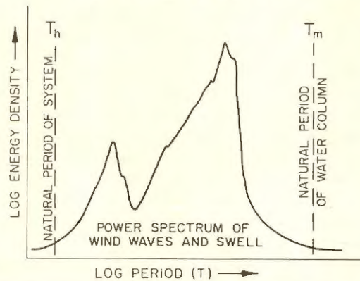
Figure 3. Response of a wave-powered generator to a random sea.
