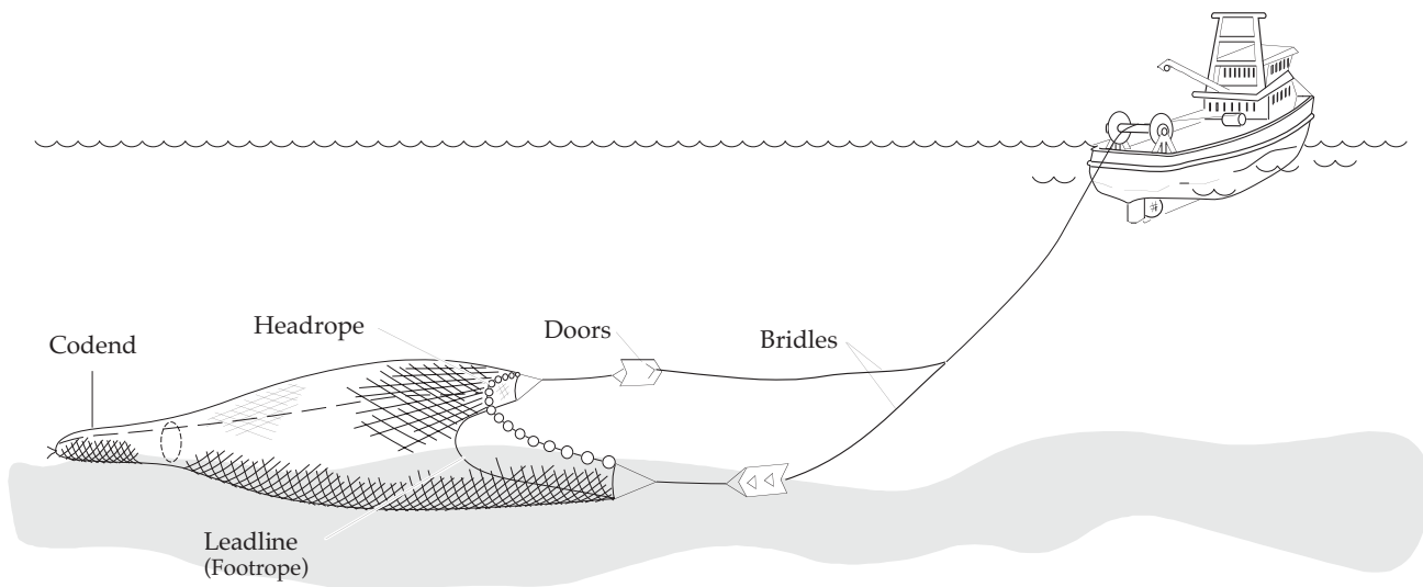
Figure 11. Example of trawl net configuration.
