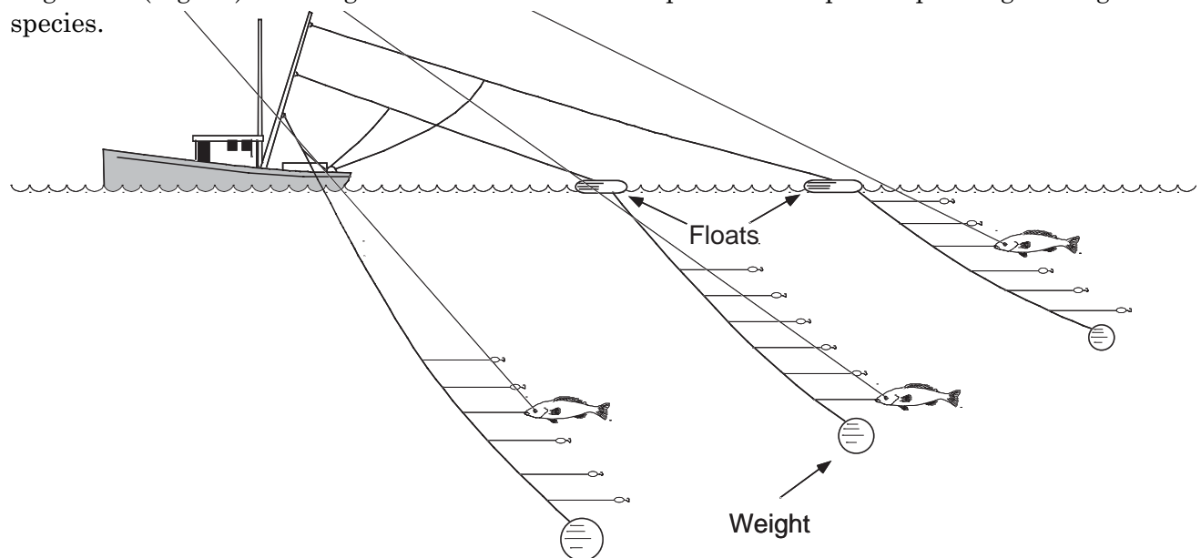
Figure 12. Example of troll fishing gear configuration.
