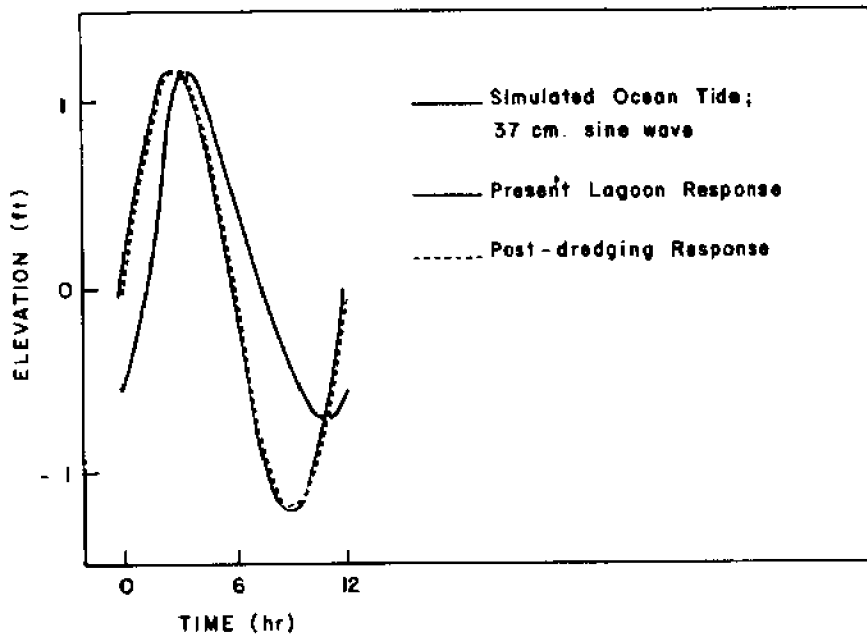
Figure 7. The response of a mathematical model developed to predict tidal fluctuations in Pala Lagoon
