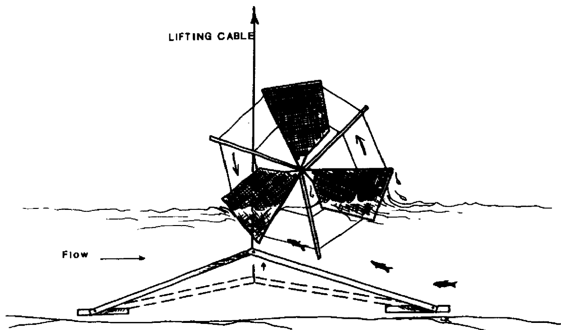
Inclined Fish Wheel
