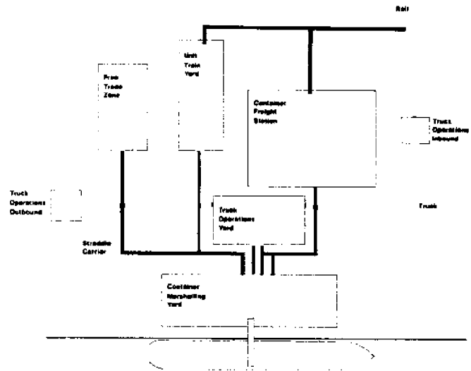
Flow diagram of a typical container facility Source: Container Services of the Atlantic
