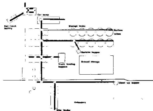
Product flow pattern of a typical grain terminal
