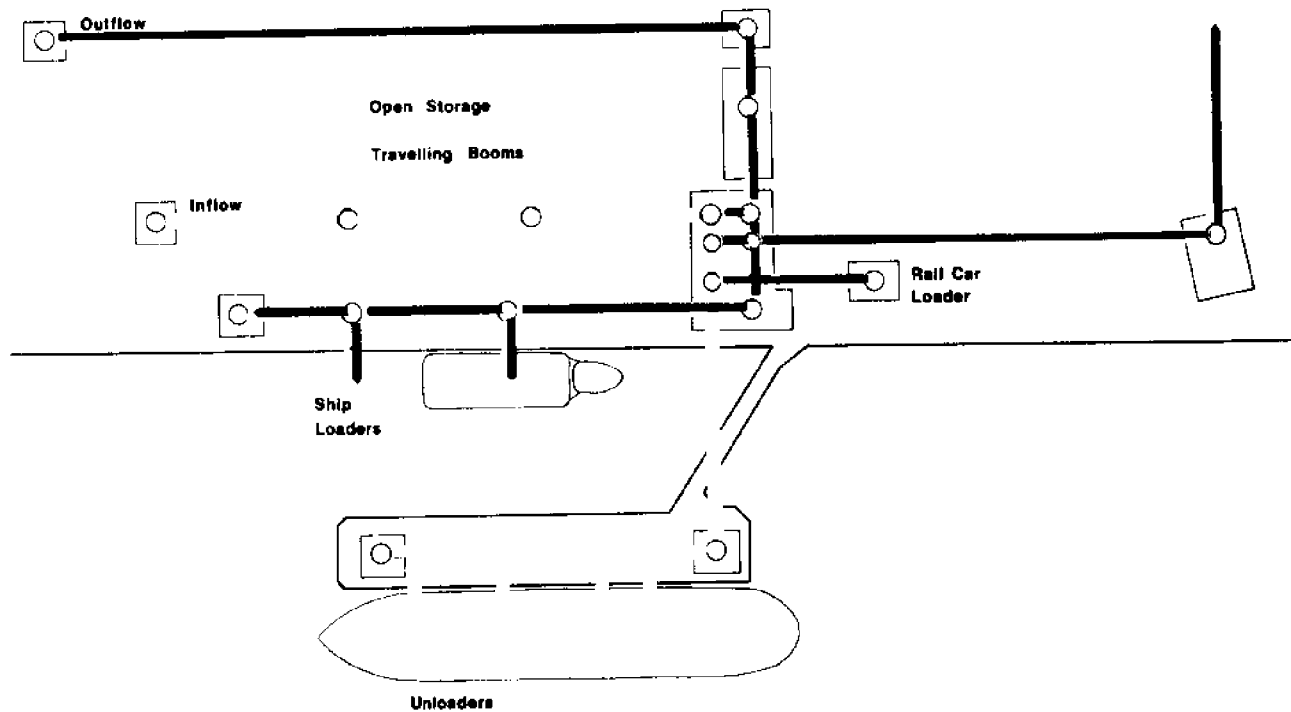
Product flow pattern of a typical ore terminal
