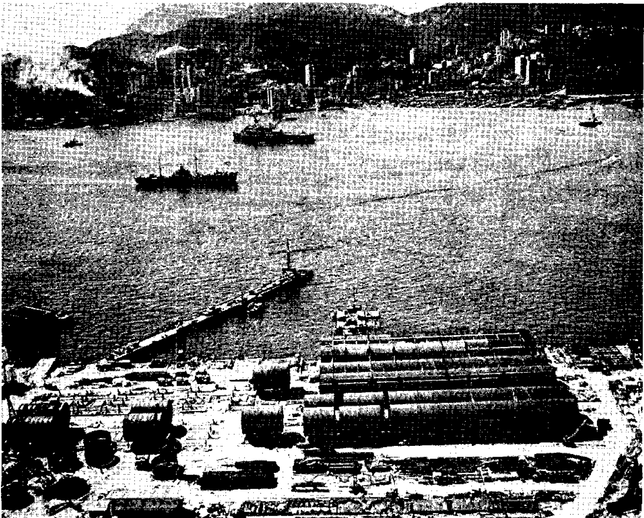
Assembly process for an underwater tunnel to connect Kowloon with Hong Kong Island Source: Part of Hong Kong
