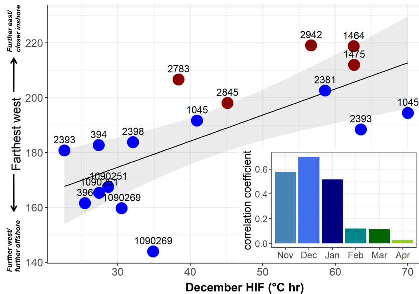
FIGURE 6 | Mean December HIF versus farthest westward location (degrees east, reached between January and June) for the 15 fish which moved offshore of the California Current in fall, and returned during spring, with tag number also shown. Blue circles show fish which departed the California Current in fall north of 40°N, red circles show fish which departed the California Current south of 40°N. Inset shows linear correlation coefficient between mean HIF and farthest west (degrees east) by month.
