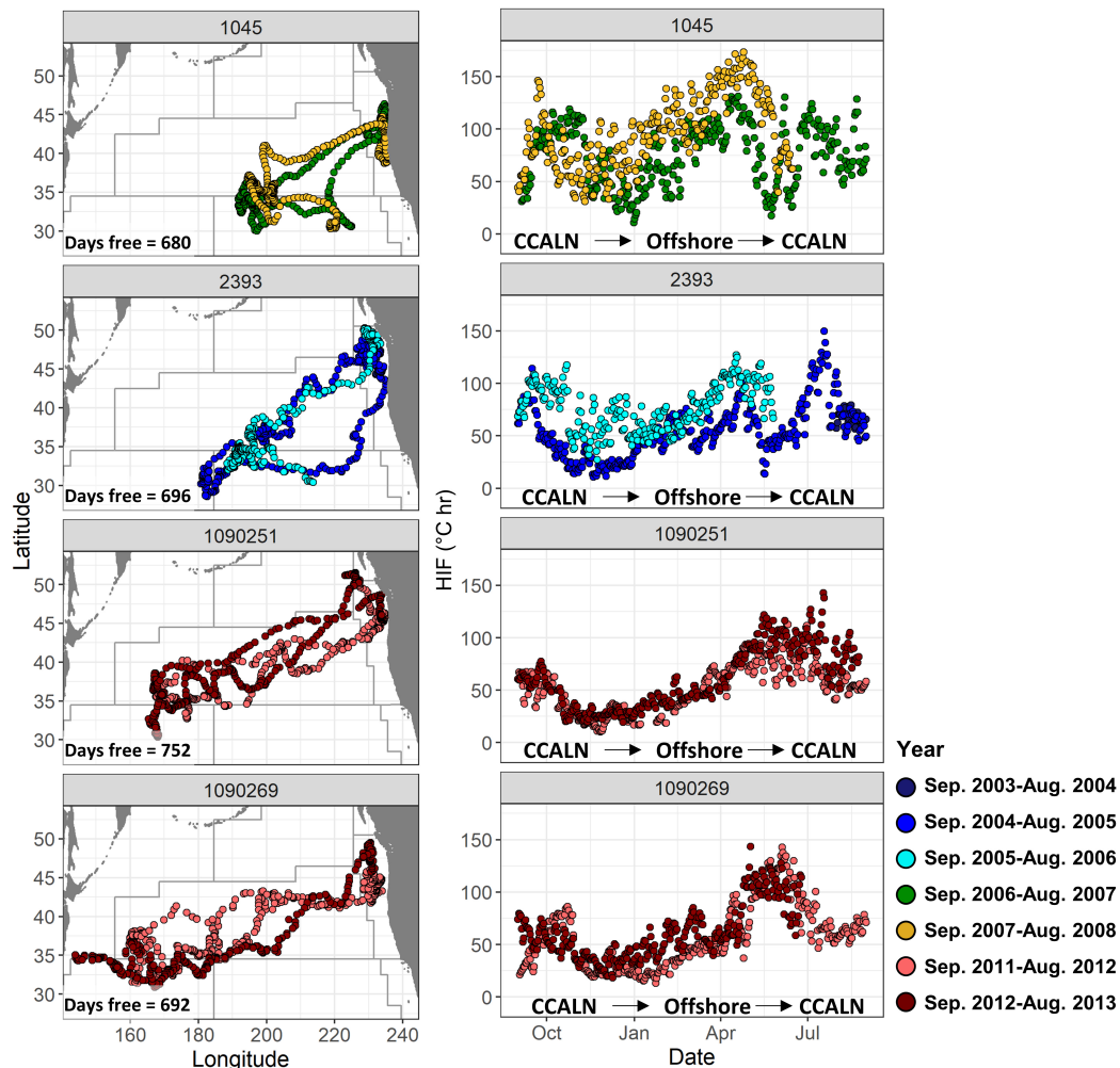
FIGURE 5 | Left: daily locations, and right: daily mean HIF for the 4 fish which were at large the longest, during both years at liberty. Years were defined from September 1st through August 31st, to coincide with typical migration timing leaving and returning to the West Coast. Boundaries of modified Longhurst regions from Figure 1 are also shown. “CCALN” denotes the northern California Current.
