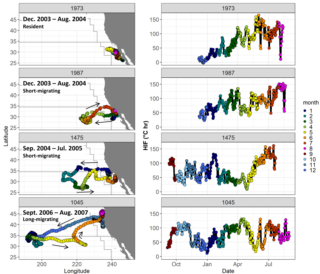
FIGURE 4 | Daily locations ( left ), and daily mean HIF ( right ) for four example fish showing different migration patterns (see Table 1 ). Colors denote month, arrows show migration directions. Boundaries of modified Longhurst regions from Figure 1 are also shown.
