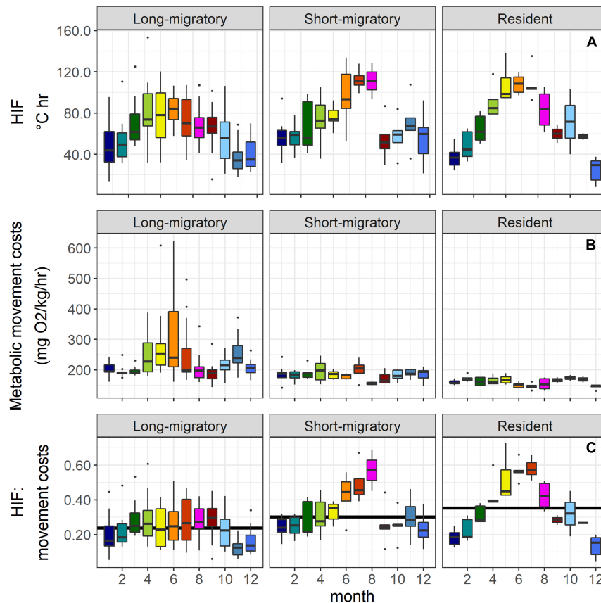
FIGURE 7 | (A) Mean monthly HIF, (B) mean monthly movement costs based on water temperature and swimming speed, and (C) HIF-cost ratio, normalized against the maximum value. Annual mean values of (C) are shown as solid black lines. Tagged fish are split into “long-migratory” fish, “short-migratory” fish, and “resident” fish (see Table 1 and Figure 1 ). Note that fish at large for more than one migration year always showed the same migratory pattern.
