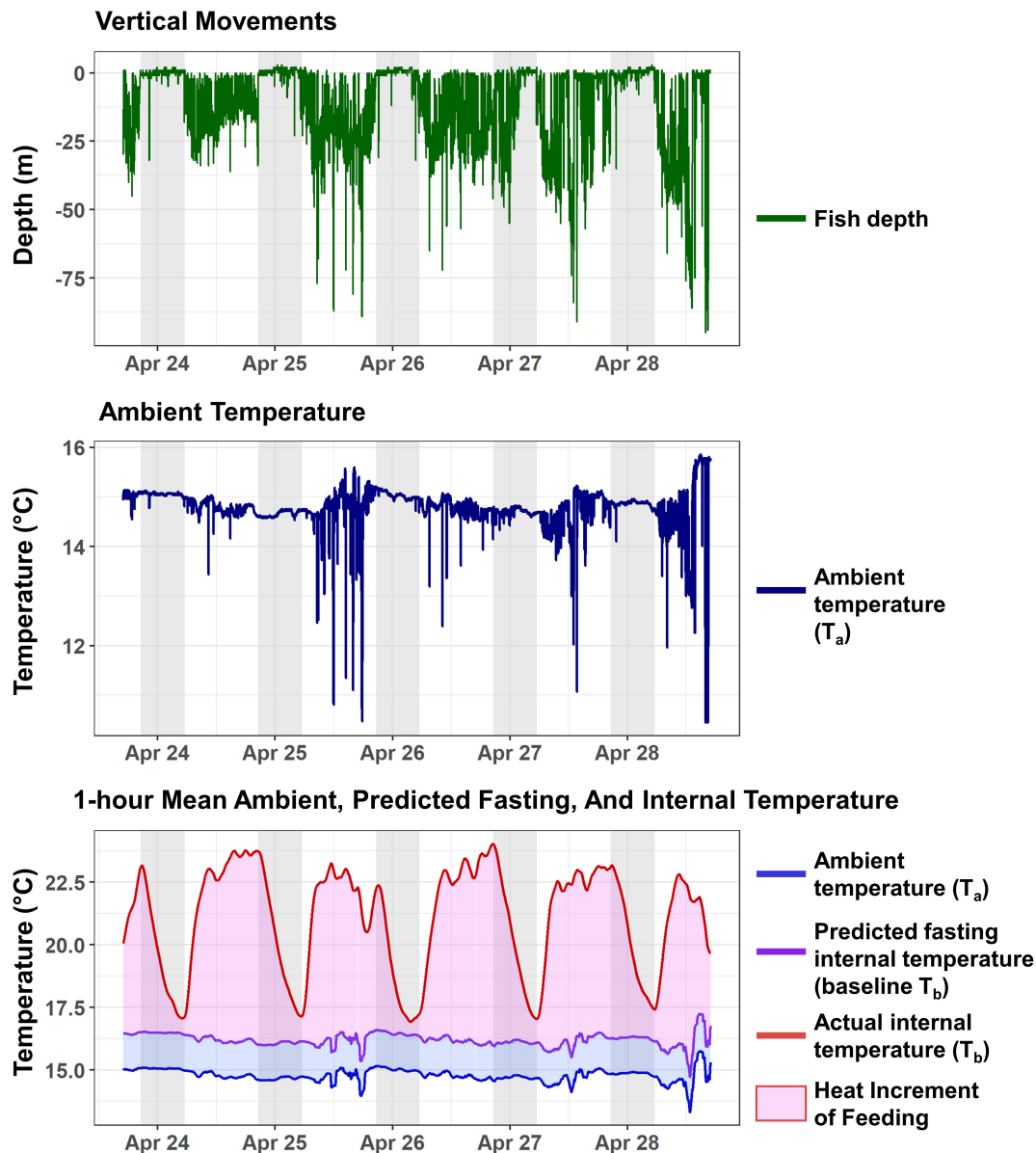
FIGURE 2 | Five days of HIF events for tag 1973 in the CCALS, April 24–28, 2004. Top: depth occupied at 1-min intervals. Middle: ambient water temperature recorded by the tag at 1-min intervals. Bottom: 1-h moving mean of ambient temperature, estimated baseline (fasting) internal temperature, and measured internal temperature. The light pink area denotes the internal temperature increase due to HIF, while the purple area is the estimated thermal excess maintained by the fish under fasting conditions. Gray shading denotes nighttime, defined as time between nautical dusk and nautical dawn.
