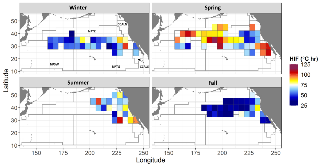
FIGURE 3 | Mean daily HIF by season at 5 \times 5 degree resolution, 2003–2013. Only grid cells with data from at least two fish are plotted. Boundaries of modified Longhurst regions from Figure 1 are also shown.
