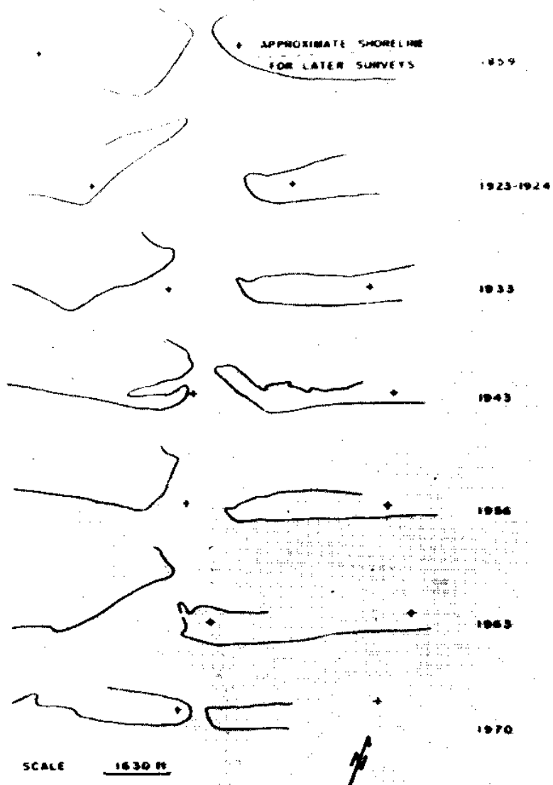
FIG 1 SURVEYED SHORELINE OF TUBBS INLET, N.C. FOR INDICATED YEARS. NOTE INCONSISTENCY OF SHORELINE IN 1859 SURVEY WITH MORE RECENT SURVEYS. THE X'S ARE IN THE SAME POSITIONS ON ALL DRAWINGS. (ADAPTED FROM DATA COMPILED BY U.S. ARMY CORPS OF ENGINEERS)
