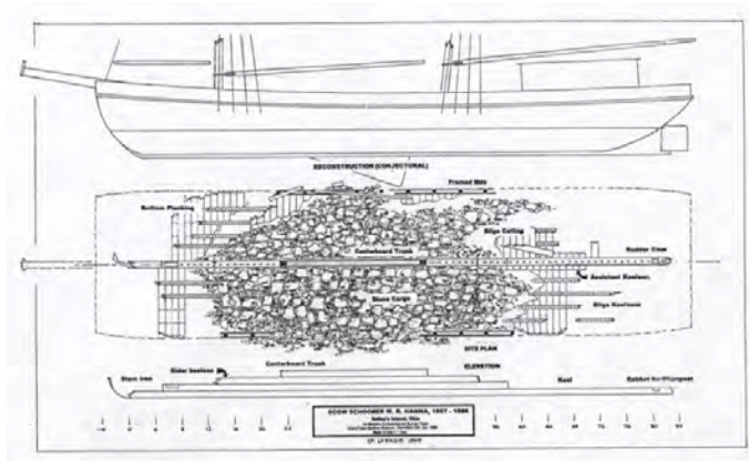
Figure 38. Site plan of W.R. Hanna (National Museum of the Great Lakes).
