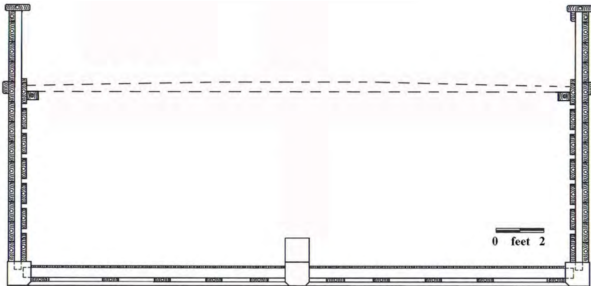
Figure 3. Cross section of a “perfectly flat” scow hull bottom (Wisconsin Historical Society).
