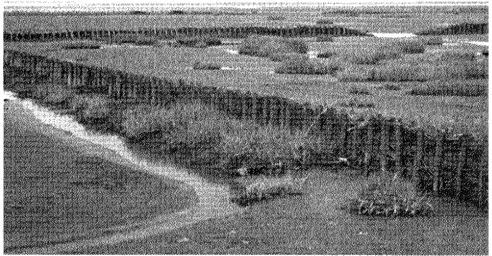
Fig 11. Soft structures for sediment control along the North Sea
