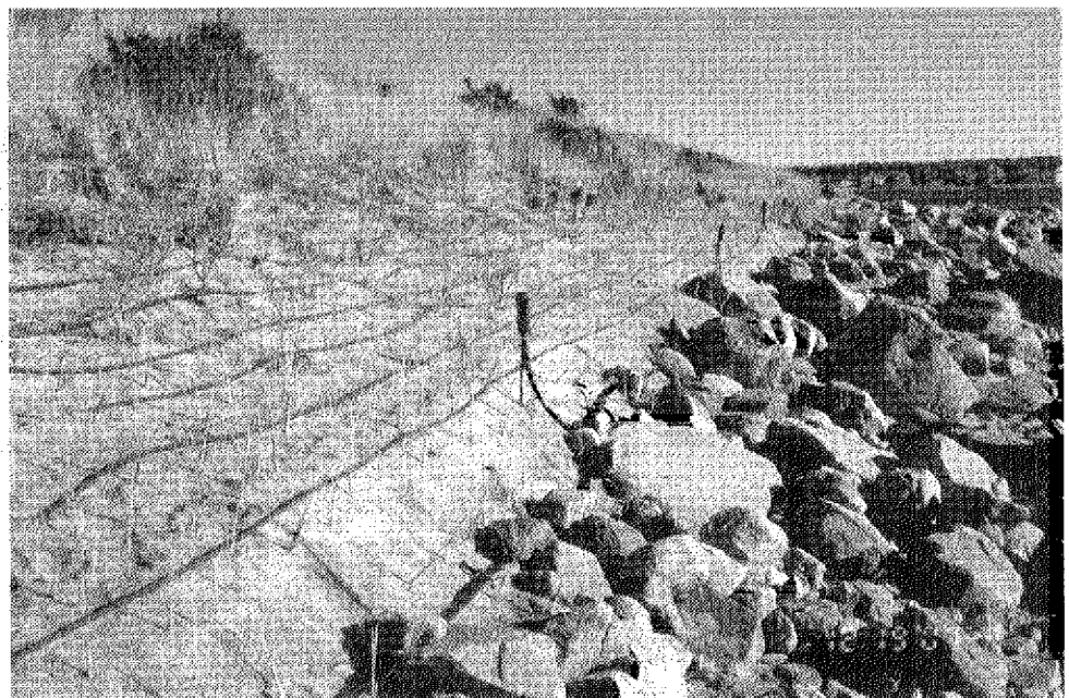
Fig 7. Coastal bank erosion control using bioengineering (bio-logs, jute netting, plants) and a system for watering and fertilizing
