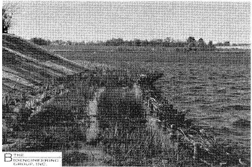
Fig 12. Sediment control using soft breakwaters & sills
