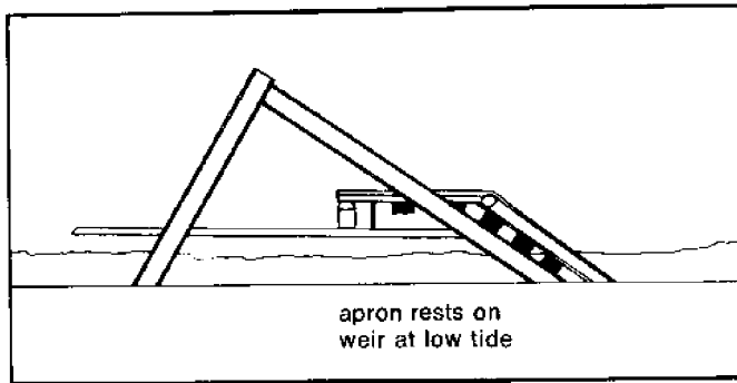
Fig. 13. Operation of the weir apron.
