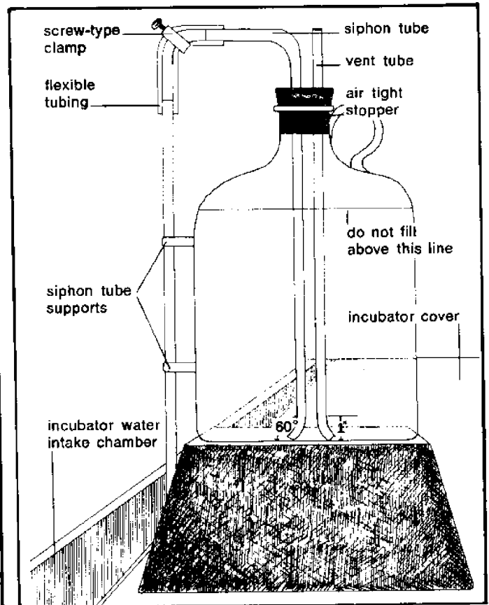
Fig. 22. Construction of drip bottle used in Malachite Green treatment.
