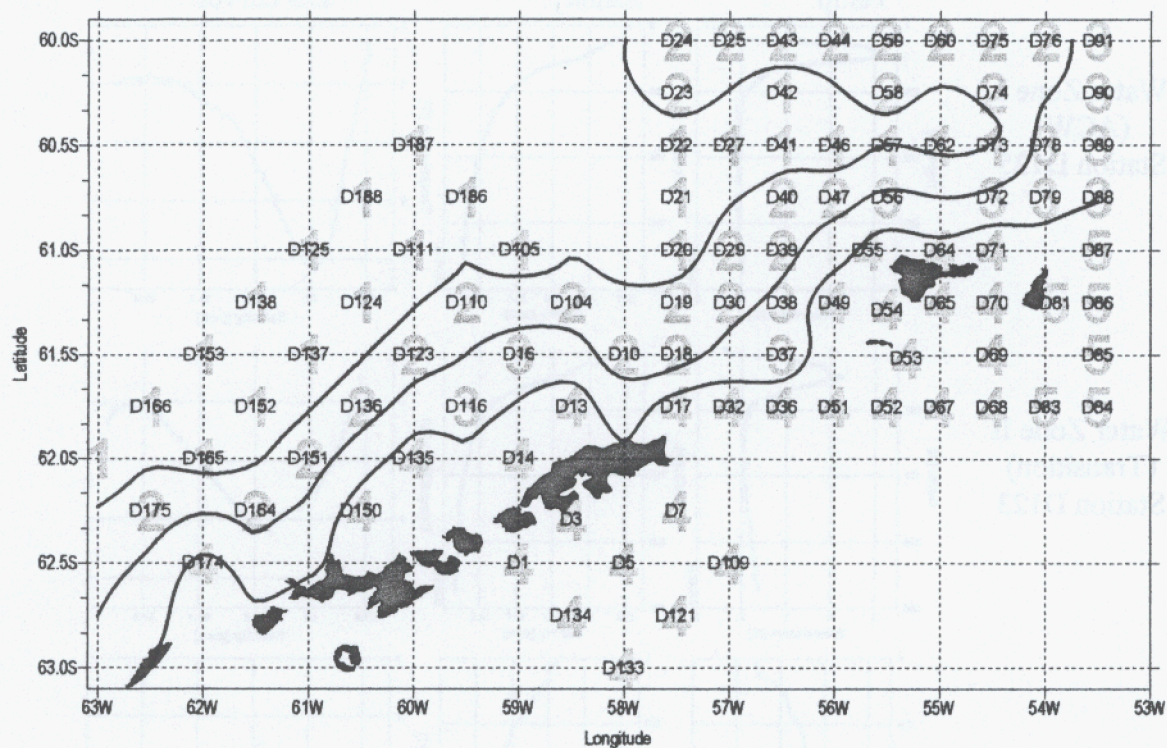
Figure 1.3 Geographic distribution of water zone types in during the AMLR survey (Leg II).
