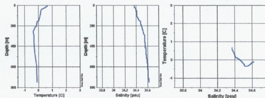
Figure 1.2 T/S curves for selected stations designated as Water Zones I through V during the AMLR survey (Leg II).
