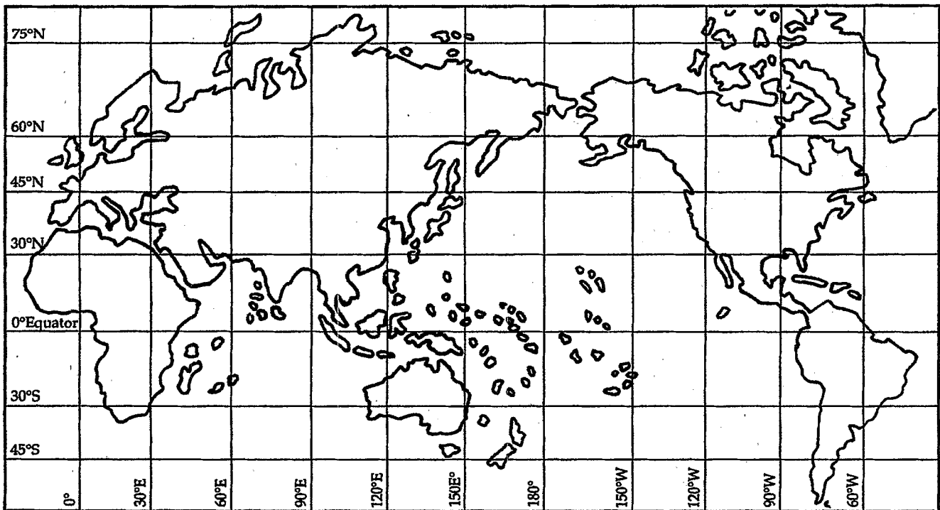
Coral distribution map
