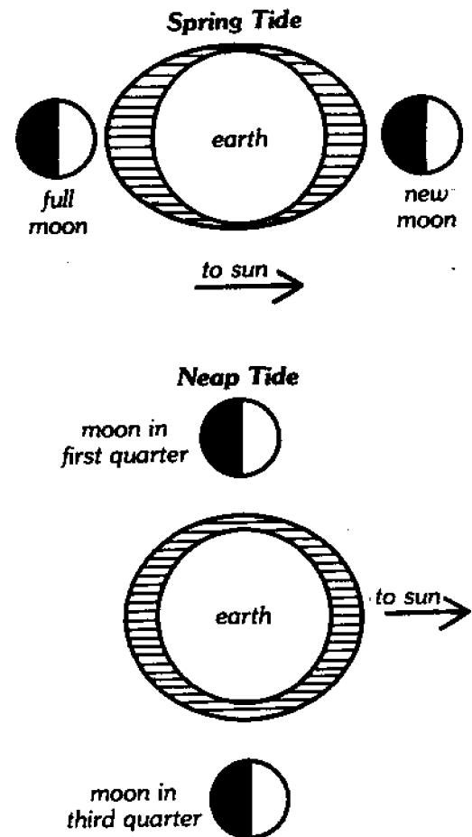
Positions of the sun and moon relative to the earth during the spring and neap tides
