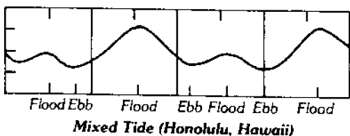
Tidal graphs and corresponding data of the three general types of tides.
