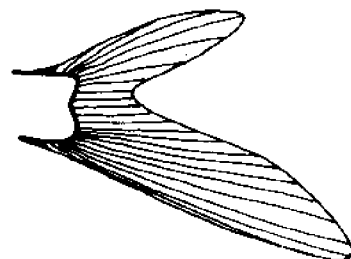
Hypocercal tail
