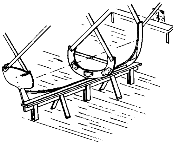
Midship Station Mold braced in place. Typical Strongback Setup.
