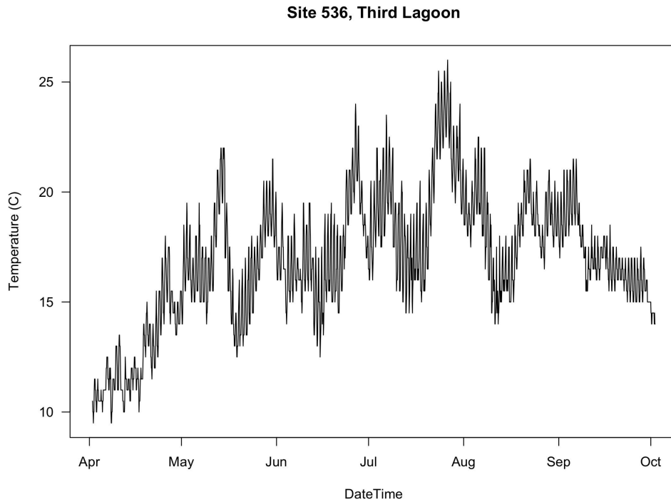
Figure 28. Sample temperature profile from a lagoon site, 536, Third Lagoon, on San Juan Island.
