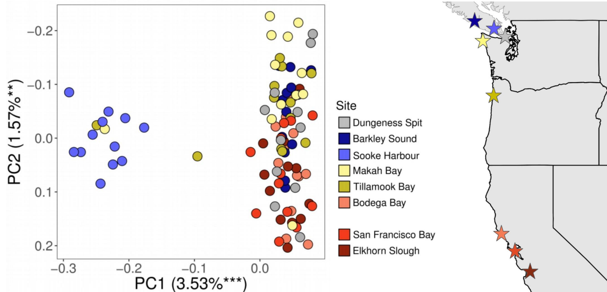
Figure 31. Genomic characterization of individual green crabs collected from sites along the US West Coast. Of particular note is the unique signature of Sooke Basin - indicated by the spatially separated cluster of dots in the plot - and that a few individuals originating from Sooke Basin were likely among those analyzed for Makah and Tillamook Bays. (Carolyn Tepolt, in prep)
