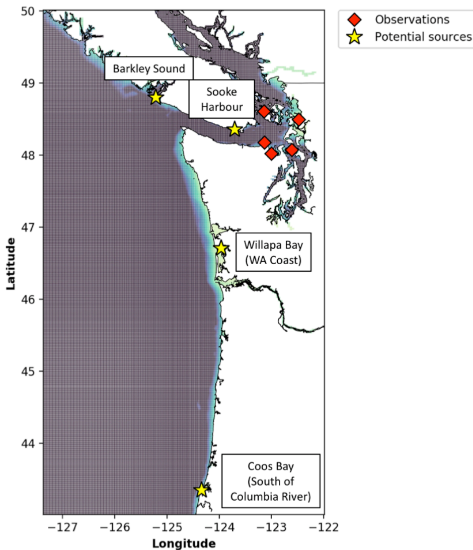
Figure 22. Map of simulated larval release locations (yellow stars). The map represents the geographic extent of the ocean model used in the experiments. Red diamonds indicate green
