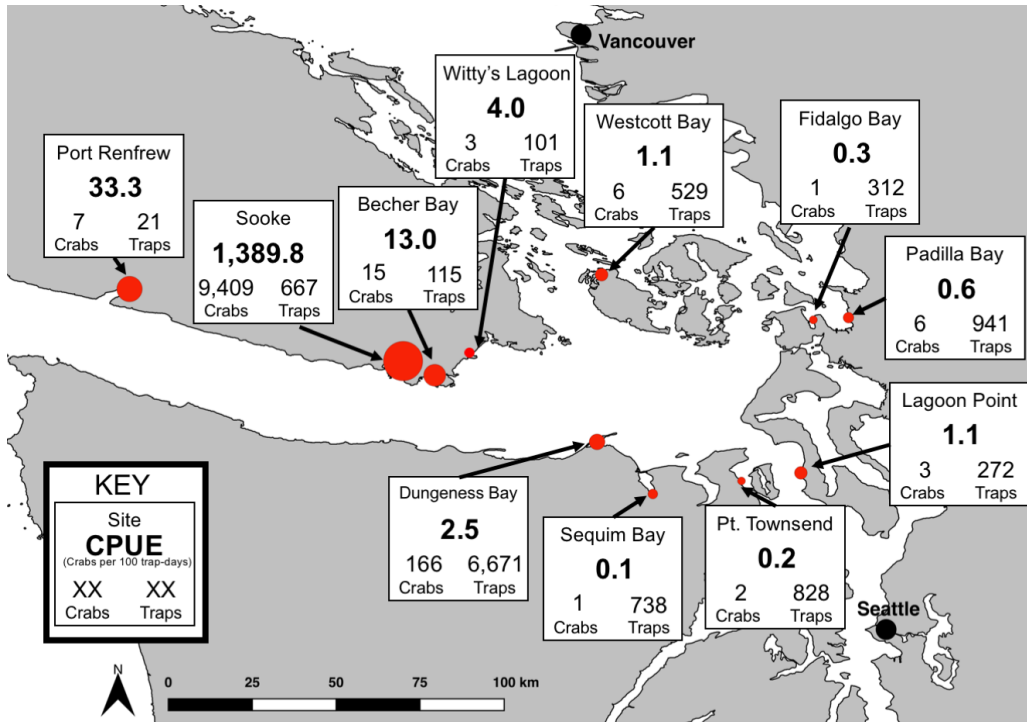
Figure 3. Summary of European green crab captures in the Salish Sea as of December 2018. Catch Per Unit Effort (CPUE) represents number of green crab captured per 100 trap days. In Washington, traps were set for approximately 24 hours, so a trap and trap day are equal. In British Columbia, the soak time was more variable so the number of traps and number of trap days are slightly different. Previous published work multiplied CPUE by 100 as convention because catches in Washington and Oregon were extremely low.
