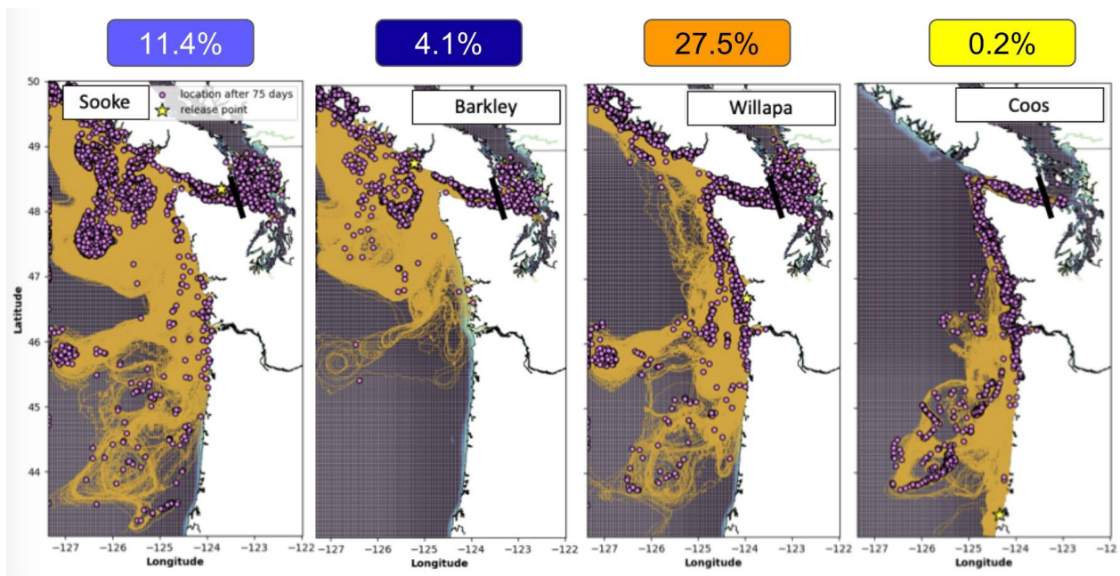
Figure 29. Examples of particle tracking experiments in which simulated larvae, released 10 August 2014, were successful reaching the Salish Sea after a 75 day period in the water column. (reproduced from Brasseale et al. 2018 in review )
