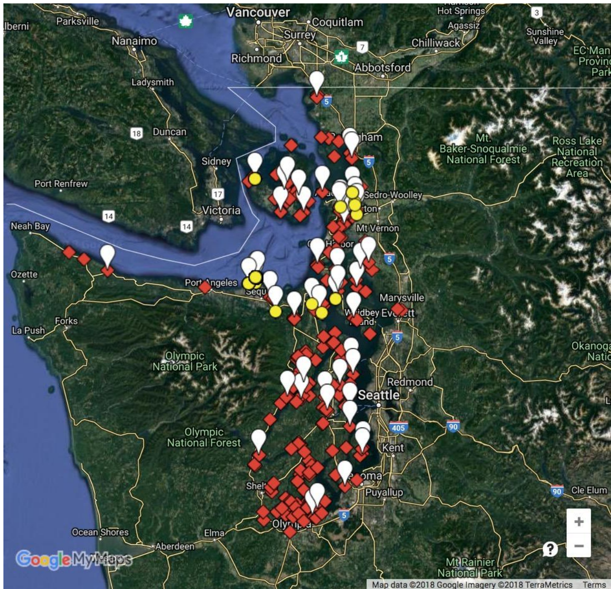
Figure 15. December 1, 2018 screenshot of the Crab Team map with most suitable habitat locations flagged as red diamonds; Crab Team monitoring sites as white bubbles and locations where green crab have been found as yellow dots. The map also includes a layer of sites previously monitored for green crab by other entities (e.g. USFWS). Data current as of December 2018. The interactive map is available at www.tinyurl.com/wagreencrab .
