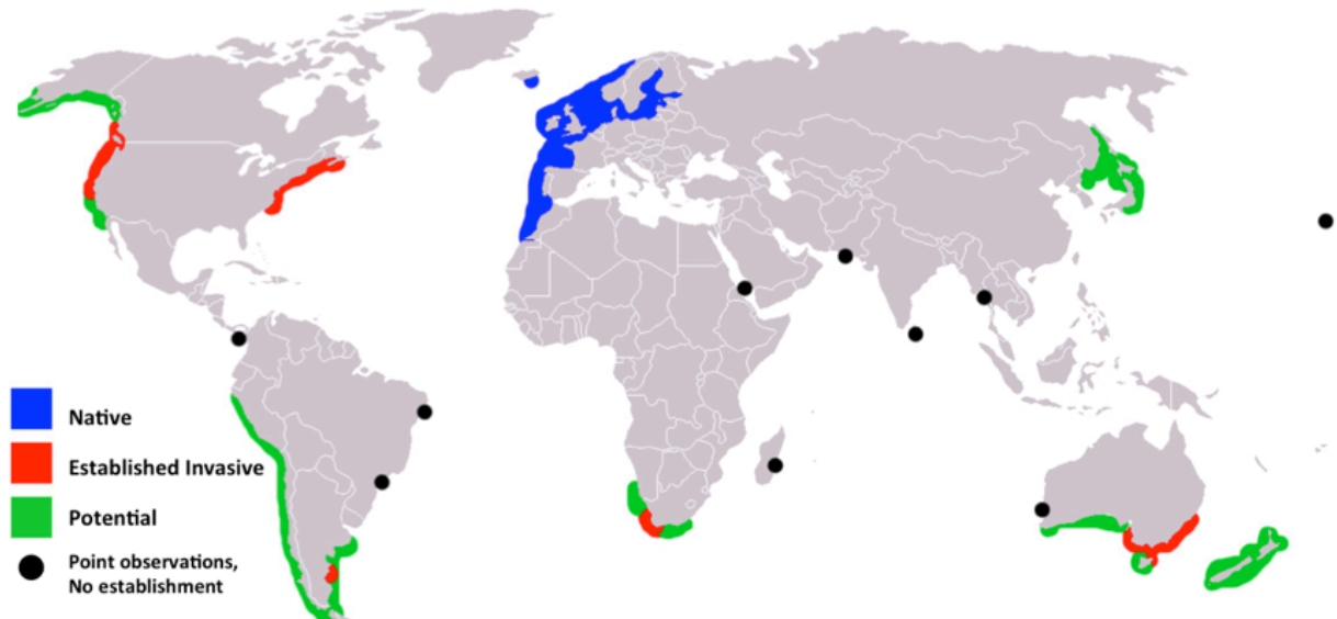
Figure 1. Realized and potential global distribution map of European green crab ( Carcinus maenas ). As of 2018, green crab are found north to Newfoundland on the Atlantic Coast of North America. Map prepared by Stemonitis (2006), English-language Wikipedia, based on a blank world map and data from Commonwealth Scientific and Industrial Research Organization (CSIRO).
