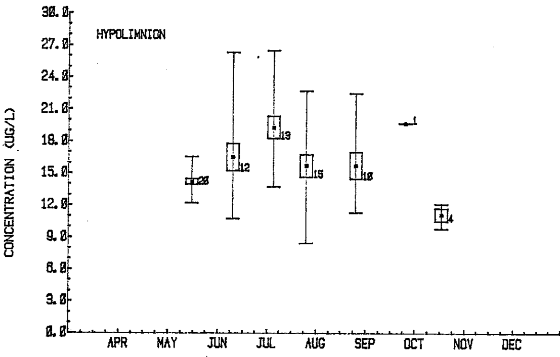
FIGURE 25. THE MEAN CENTRAL BASIN EPILIMNION AND HYPOLIMNION TOTAL PHOSPHORUS CONCENTRATIONS FOR 1979 (CCIW-NWRI).
