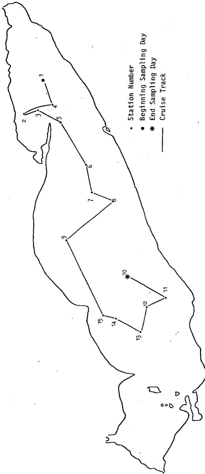
FIGURE 6. REPRESENTATIVE CRUISE TRACK USED BY CCIW-NWRI DURING 1979 (TAKEN FROM CRUISE 103, MAY 15 - MAY 18).
