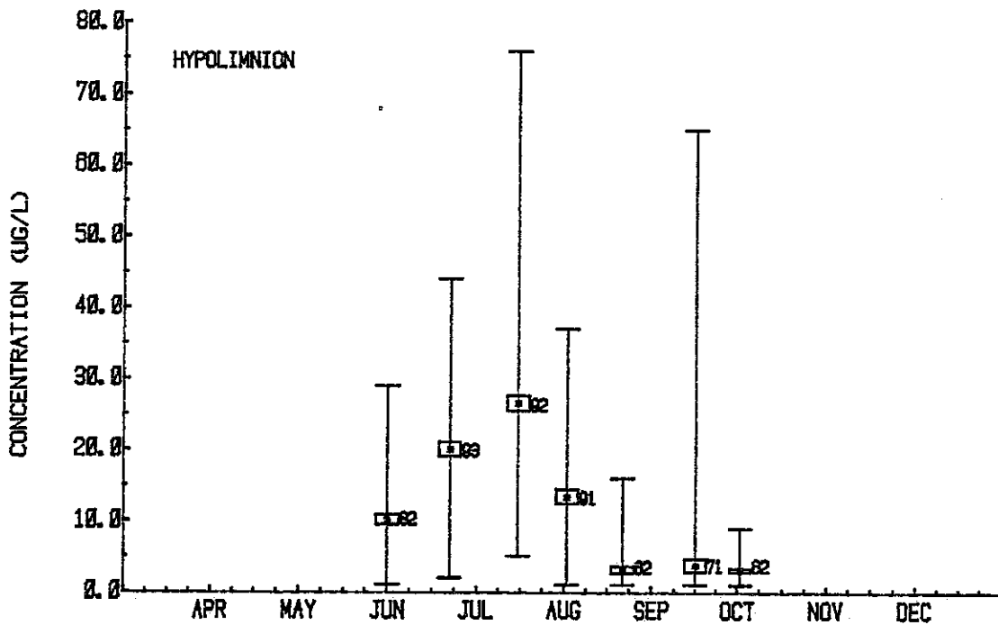
FIGURE 32. THE MEAN EASTERN BASIN EPILIMNION AND HYPOLIMNION AMMONIA CONCENTRATIONS FOR 1978 (CCIW-NWRI).
