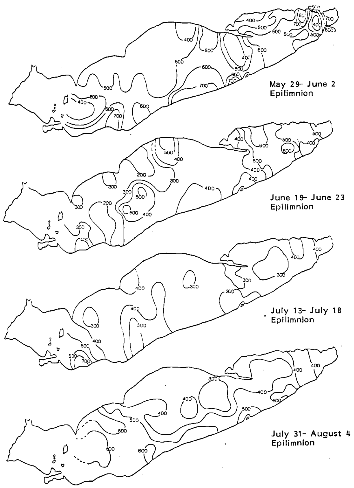
FIGURE 42. THE SEASONAL EPIILMNION PARTICULATE ORGANIC CARBON ( \mu\text{g}/\text{l} ) DISTRIBUTION PATTERNS FOR THE CENTRAL AND EASTERN BASINS OF LAKE ERIE FOR 1978 (CCIW-NWRI).
