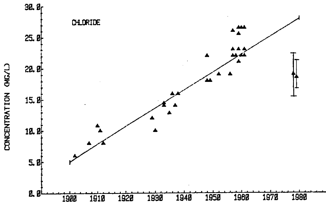
FIGURE 119. SPECIFIC CONDUCTANCE AND CHLORIDE TREND ANALYSIS FOR THE CLEVELAND AREA AS REPORTED BY BEETON (1961) AND RICHARDS (1981).
