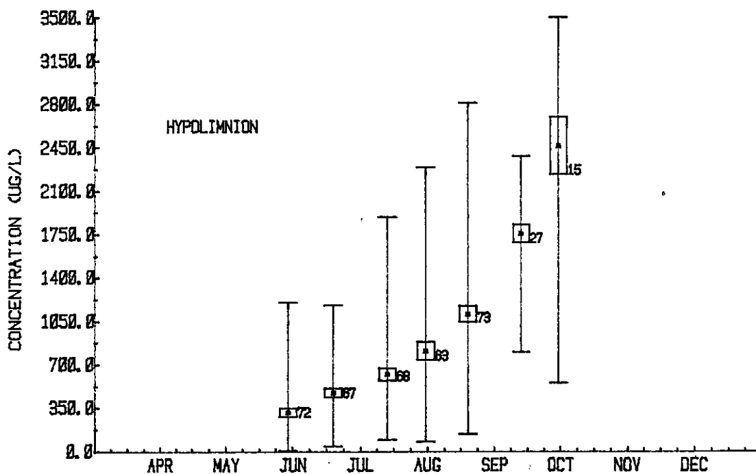
FIGURE 39. THE MEAN CENTRAL BASIN EPILIMNION AND HYPOLIMNION CONCENTRATIONS OF DISSOLVED SILICA FOR 1978 (CCIW-NWRI).
