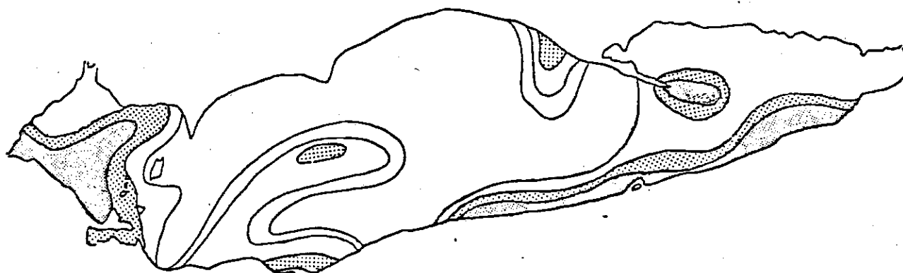
FIGURE 66b. THE DISTRIBUTION PATTERN OF MERCURY CONCENTRATIONS (mg/kg) IN THE SURFICIAL SEDIMENTS OF LAKE ERIE DURING 1979.
