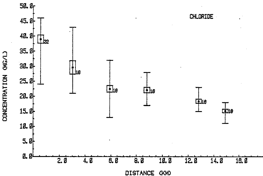
FIGURE 96. MEAN TOTAL PHOSPHORUS AND CHLORIDE CONCENTRATIONS FOR WESTERN BASIN TRANSECT 26 - MAUMEE BAY, 1978 - 1979.
