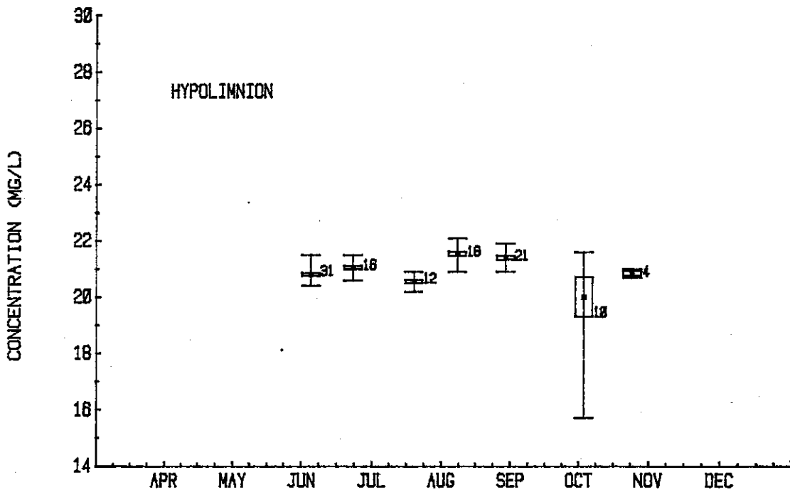
FIGURE 59. THE MEAN EASTERN BASIN EPILIMNION AND HYPOLIMNION CHLORIDE CONCENTRATIONS FOR 1978 (USEPA-GLNPO).
