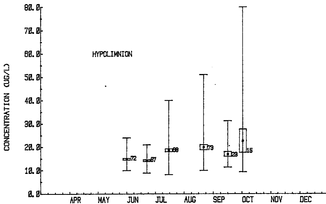
FIGURE 22. THE MEAN CENTRAL BASIN EPILIMNION AND HYPOLIMNION TOTAL PHOSPHORUS CONCENTRATIONS FOR 1978 (CCIW - NWRI).
