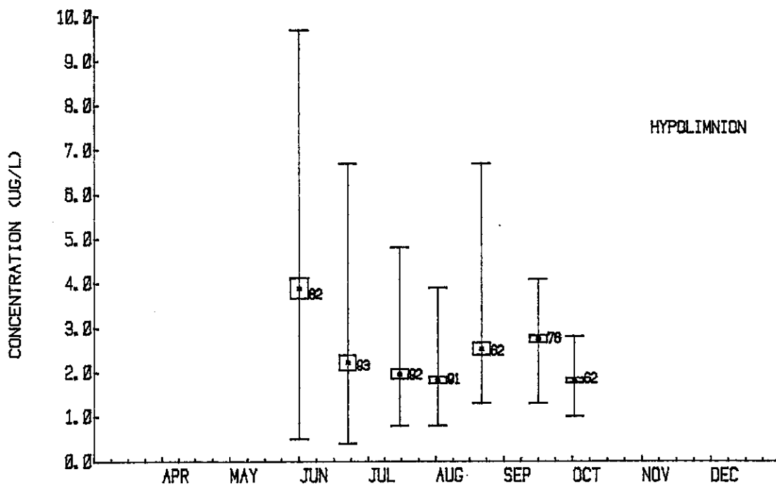
FIGURE 28. THE MEAN EASTERN BASIN EPILIMNION AND HYPOLIMNION SOLUBLE REACTIVE PHOSPHORUS CONCENTRATIONS FOR 1978 (CCIW-NWRI).
