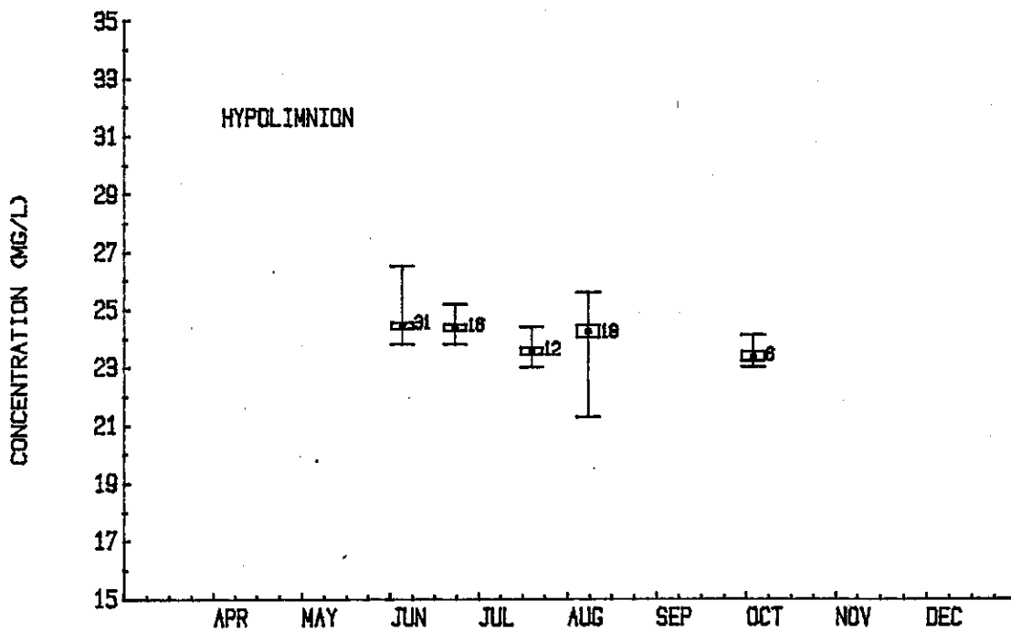
FIGURE 63. THE MEAN EASTERN BASIN EPILIMNION AND HYPOLIMNION SULFATE CONCENTRATIONS FOR 1978 (USEPA-GLNPO).
