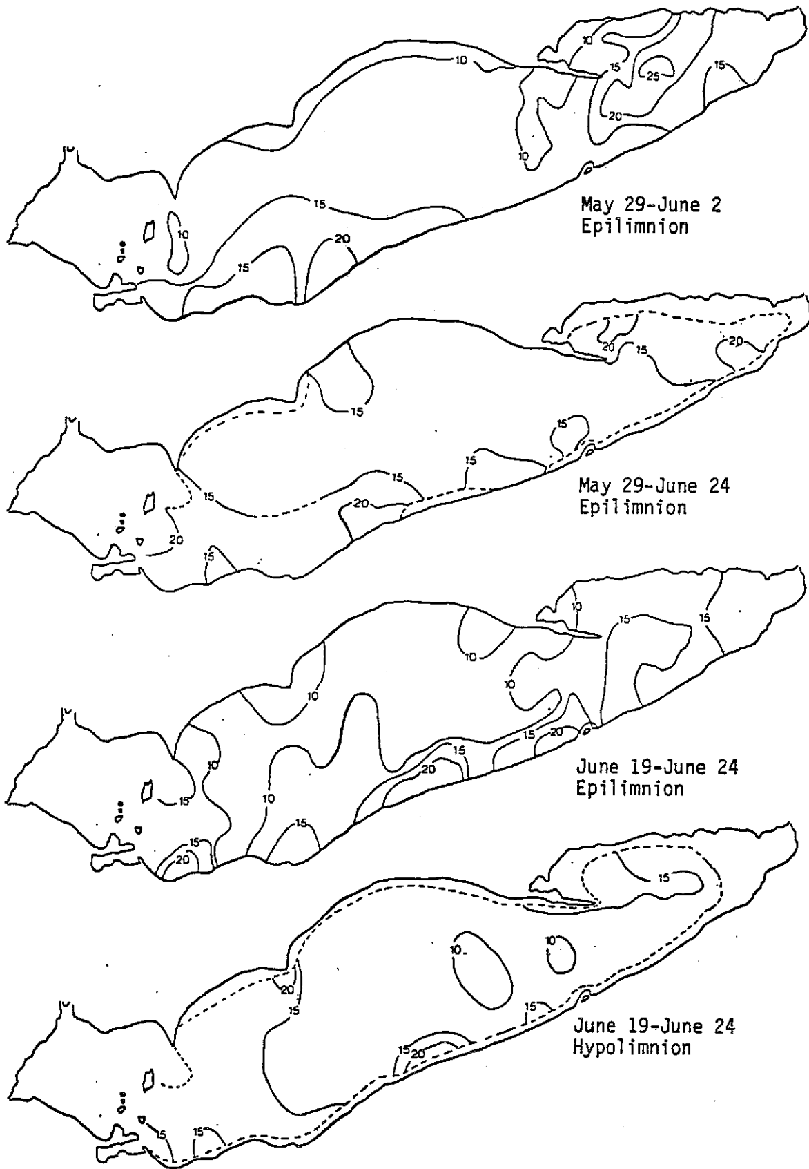
FIGURE 20. THE SEASONAL EPIILMNIION AND HYPOLIMNIION TOTAL PHOSPHORUS (ug/l) DISTRIBUTION PATTERNS FOR THE CENTRAL AND EASTERN BASINS OF LAKE ERIE FOR 1978 (CCIW-NWRI).
