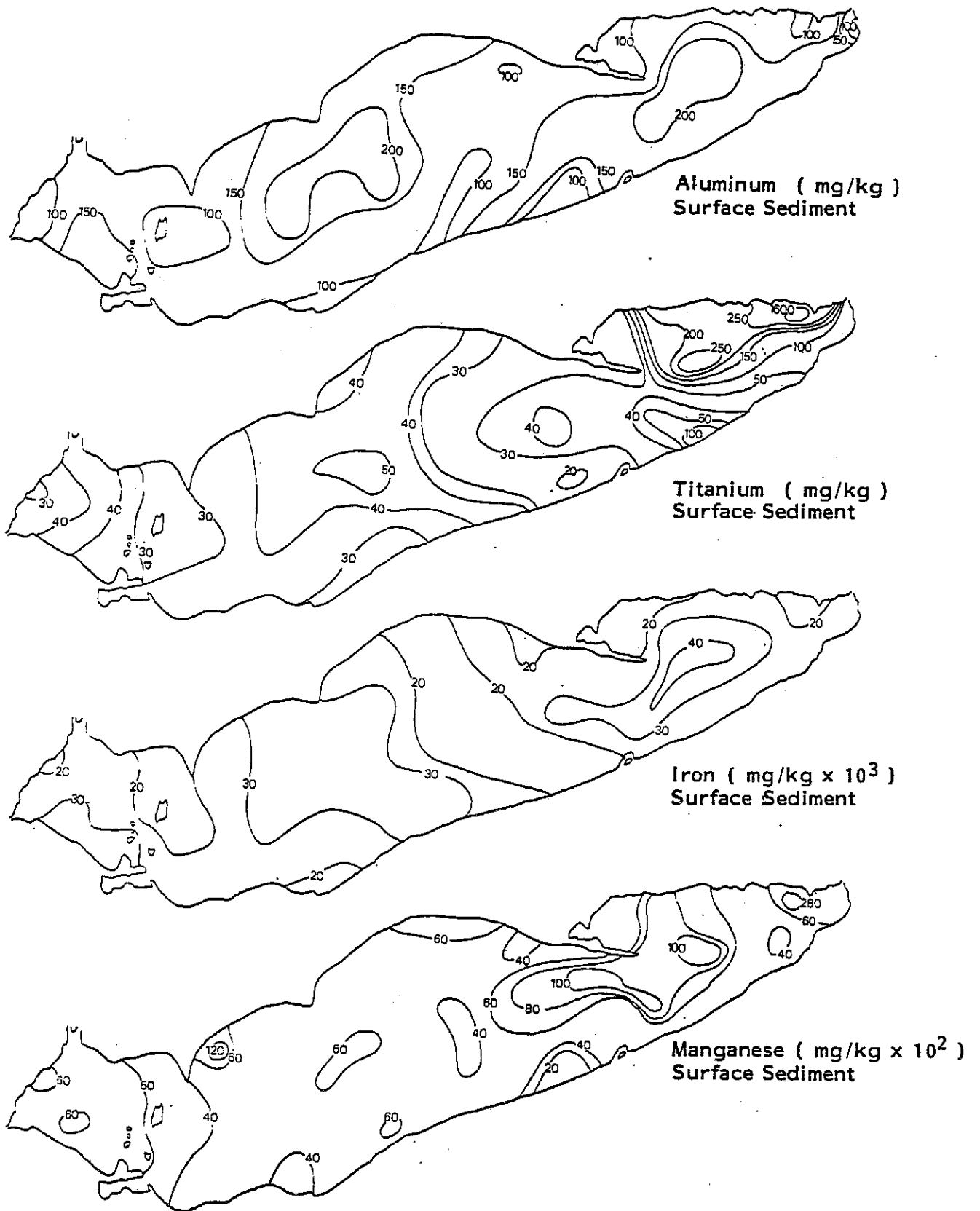
FIGURE 64. THE 1979 DISTRIBUTION PATTERNS OF SURFICIAL SEDIMENT METAL CONCENTRATIONS IN LAKE ERIE (USEPA-GLNPO).
