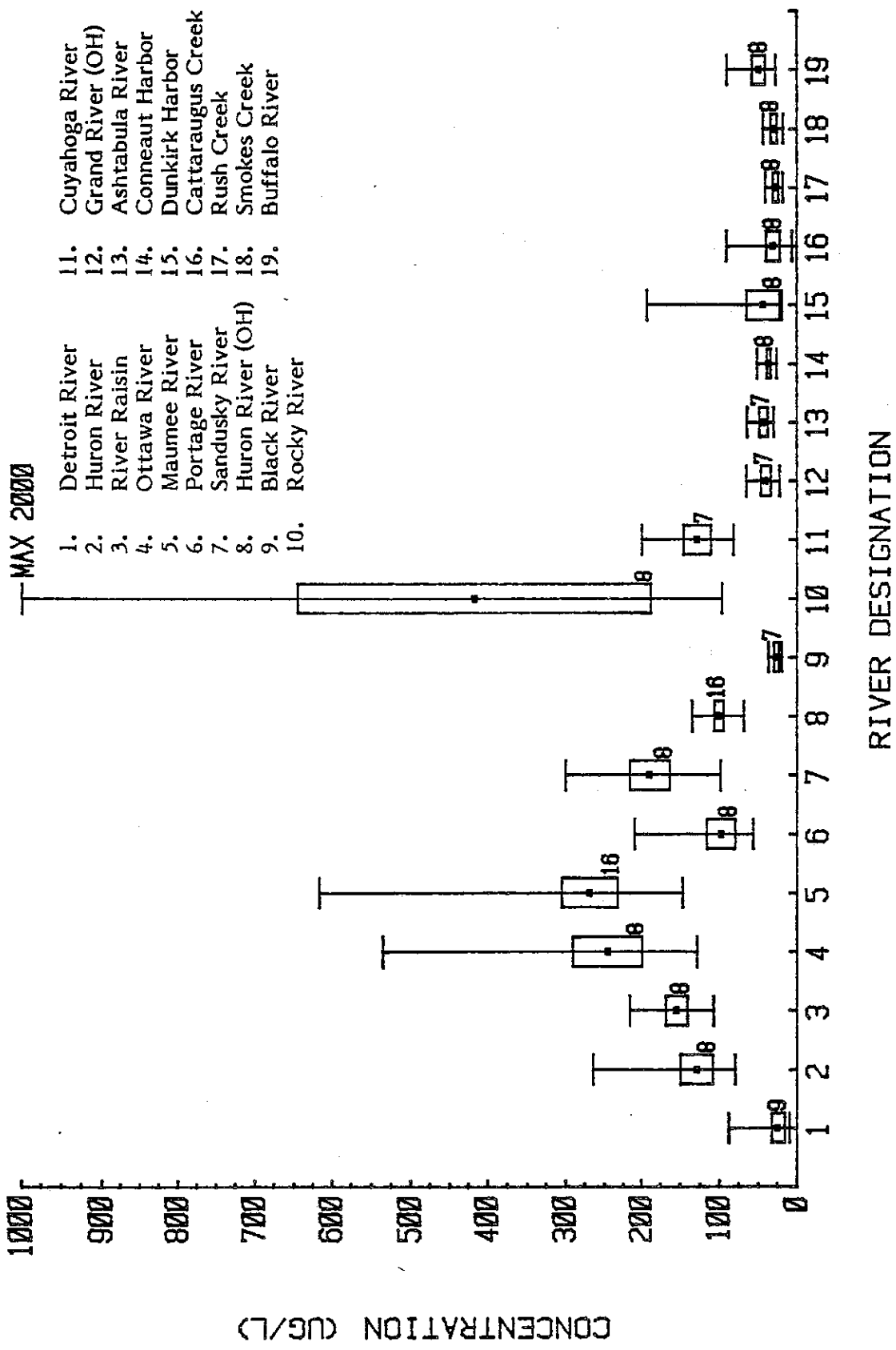
FIGURE 78. SOUTH SHORE RIVER AND HARBOR MEAN TOTAL PHOSPHORUS CONCENTRATIONS SUMMARIZED FOR 1978 - 1979.
