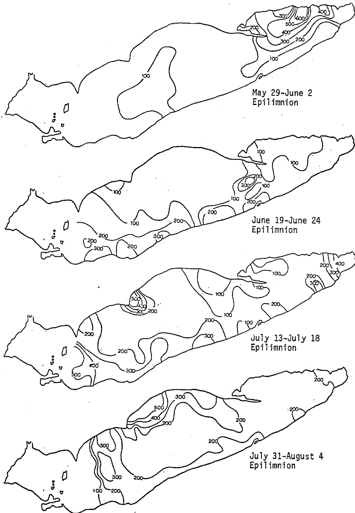
FIGURE 37. THE SEASONAL EPILIMNION DISSOLVED SILICA ( \mu\text{g/l} ) DISTRIBUTION PATTERNS FOR THE CENTRAL AND EASTERN BASINS OF LAKE ERIE FOR 1978 (CCIW-NWRI). F-44
