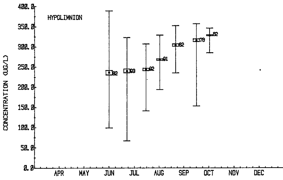
FIGURE 36. THE MEAN EASTERN BASIN EPIILMNION AND HYPOLIMNION NITRATE PLUS NITRITE CONCENTRATIONS FOR 1978 (CCIW-NWRI).
