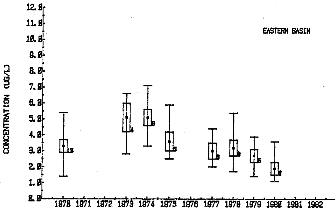
FIGURE 108. CENTRAL AND EASTERN BASIN ANNUAL CRUISE MEAN CONCENTRATIONS OF CORRECTED CHLOROPHYLL A FOR 1970 - 1982.
