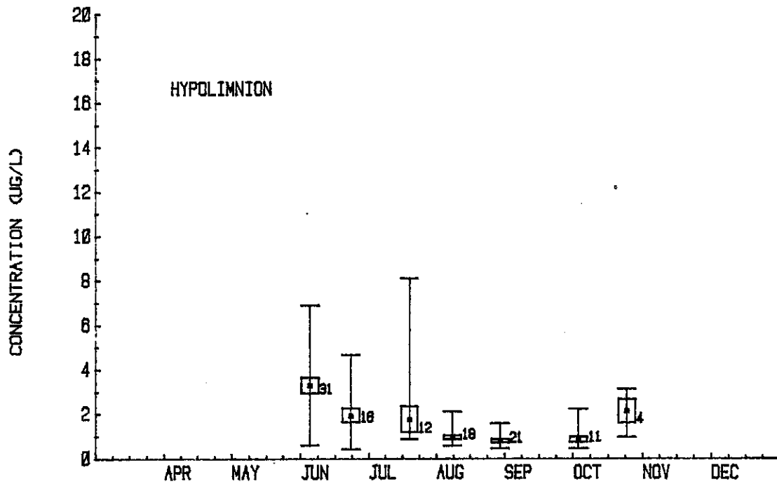
FIGURE 45. THE MEAN EASTERN BASIN EPILIMNION AND HYPOLIMNION CORRECTED CHLOROPHYLL A CONCENTRATIONS FOR 1978 (USEPA-GLNPO).
