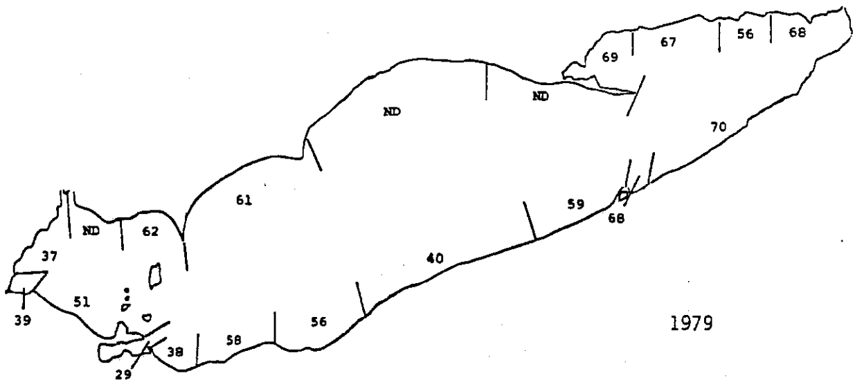
FIGURE 103. STEINHART WATER QUALITY INDEX NUMBERS FOR THE NEARSHORE REACHES 1978 AND 1979.
