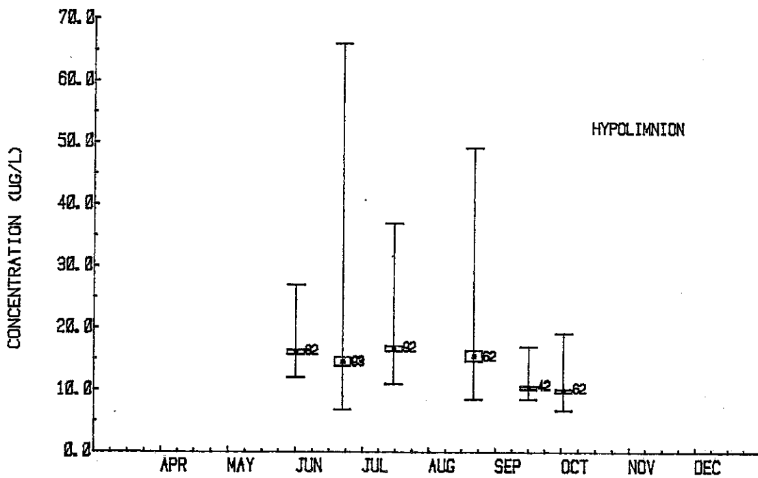
FIGURE 23. THE MEAN EASTERN BASIN EPILIMNION AND HYPOLIMNION TOTAL PHOSPHORUS CONCENTRATIONS FOR 1978 (CCIW - NWRD).
