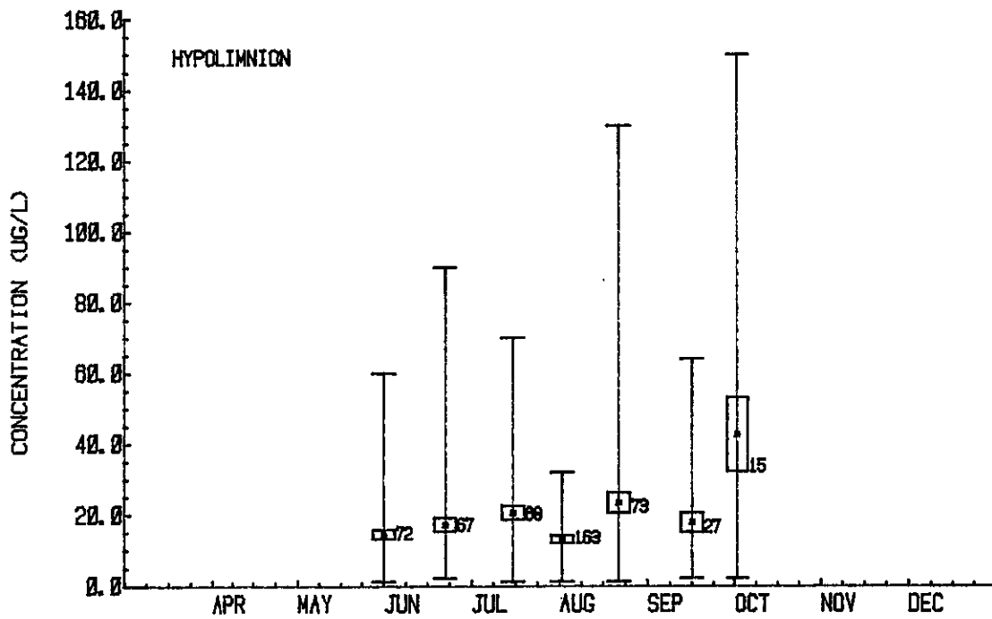
FIGURE 31. THE MEAN CENTRAL BASIN EPIILMNION AND HYPOLIMNION AMMONIA CONCENTRATIONS FOR 1978 (CCIW-NWRI).
