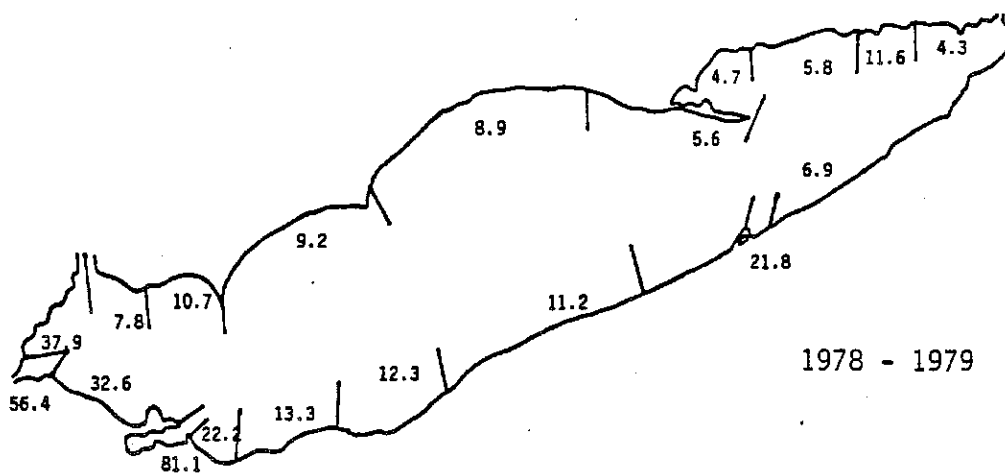
FIGURE 102. COMPOSITE TROPHIC INDEX NUMBERS FOR THE SUMMER MEAN 1972-1973 AND THE ANNUAL MEAN FOR 1978-1979.
