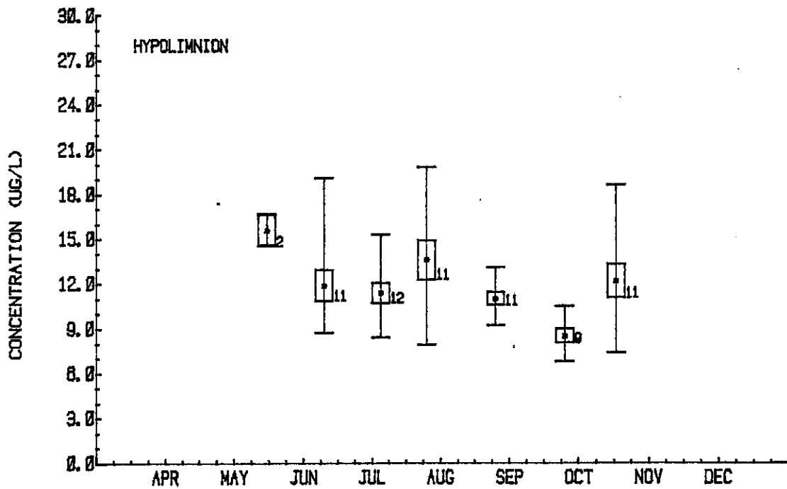
FIGURE 26. THE MEAN EASTERN BASIN EPILIMNION AND HYPOLIMNION TOTAL PHOSPHORUS CONCENTRATIONS FOR 1979 (CCIW-NWRI).
