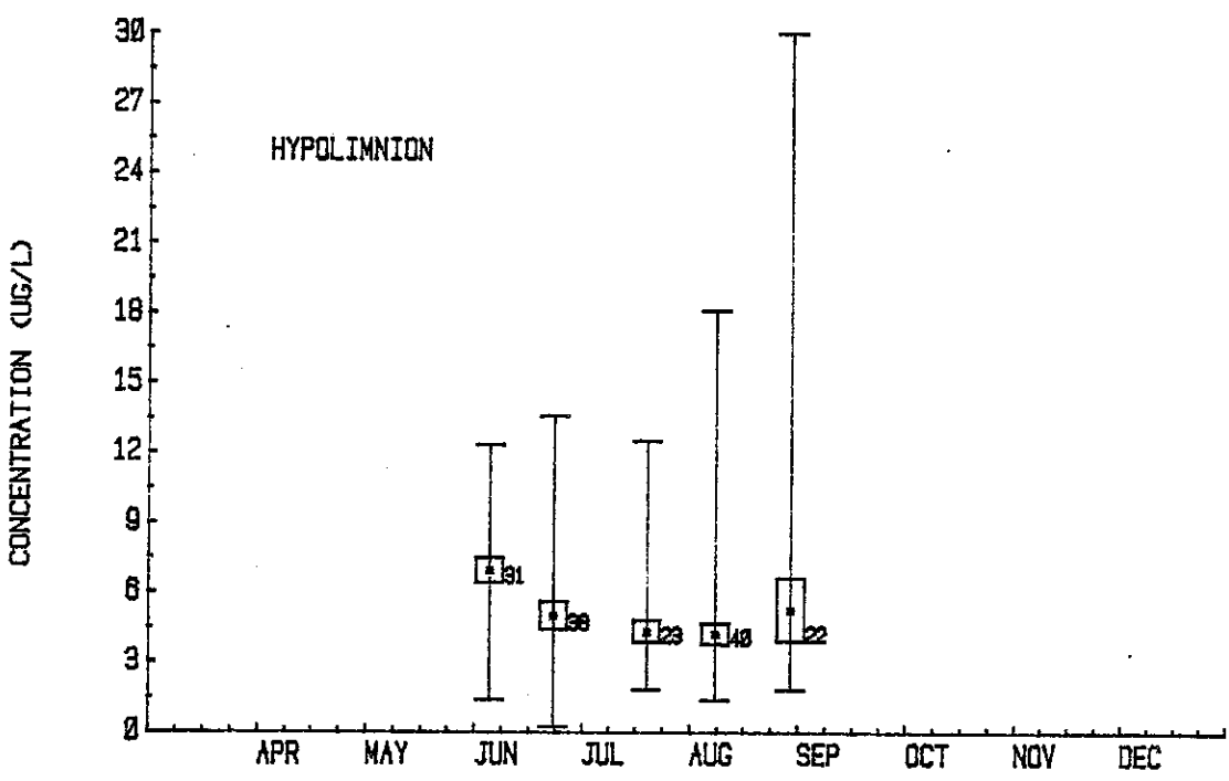
FIGURE 44. THE MEAN CENTRAL BASIN EPIILIMNION AND HYPOLIMNION CORRECTED CHLOROPHYLL A CONCENTRATIONS FOR 1978 (USEPA-GLNPO).
