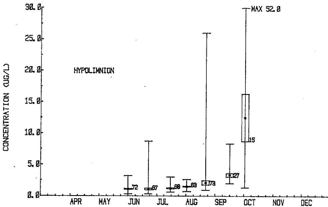
FIGURE 27. THE MEAN CENTRAL BASIN EPIILMNIION AND HYPOLIMNIION SOLUBLE REACTIVE PHOSPHORUS CONCENTRATIONS FOR 1978 (CCIW - NWRI).
