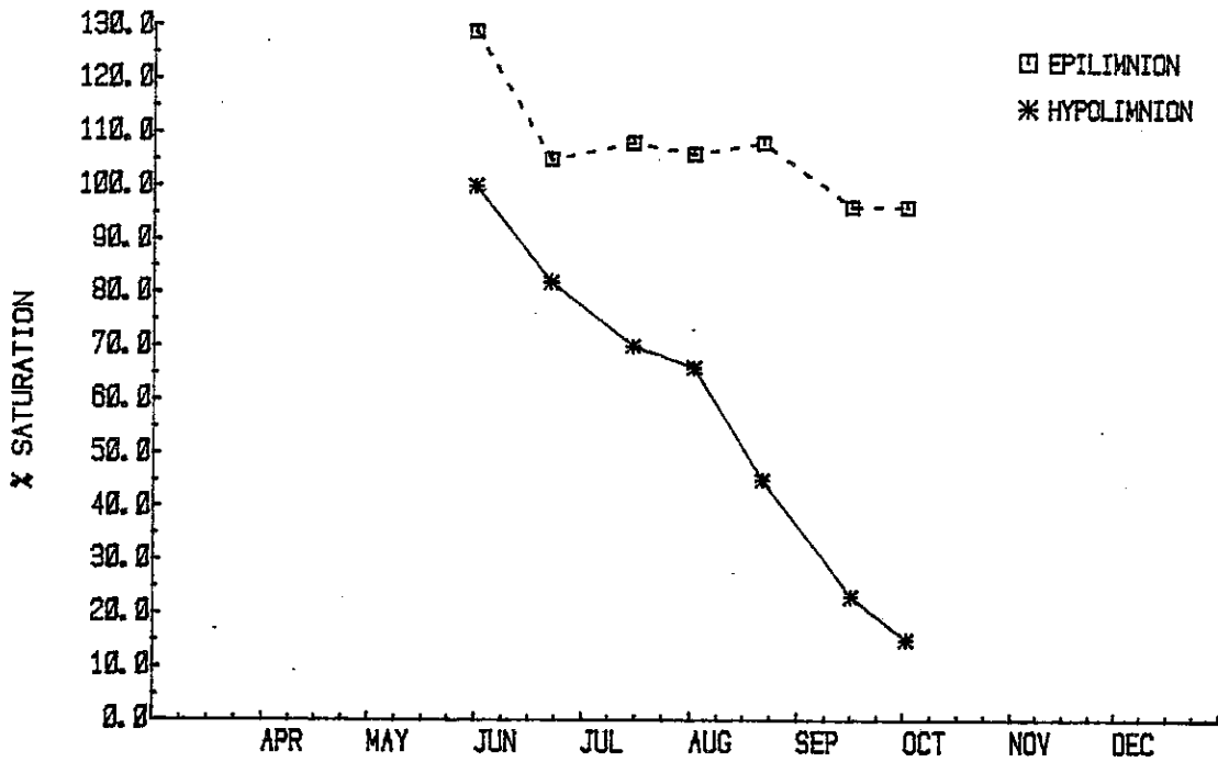
FIGURE 17. THE MEAN CENTRAL BASIN DISSOLVED OXYGEN CONCENTRATIONS AND PERCENT SATURATIONS FOR 1978 CCIW - NWRI.
