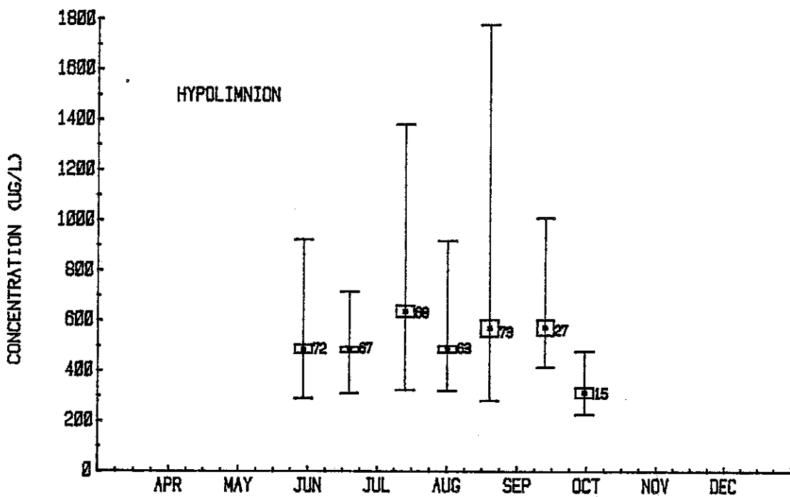
FIGURE 46. THE MEAN CENTRAL BASIN EPILIMNION AND HYPOLIMNION PARTICULATE ORGANIC CARBON CONCENTRATIONS FOR 1978 (CCIW-NWRI).
