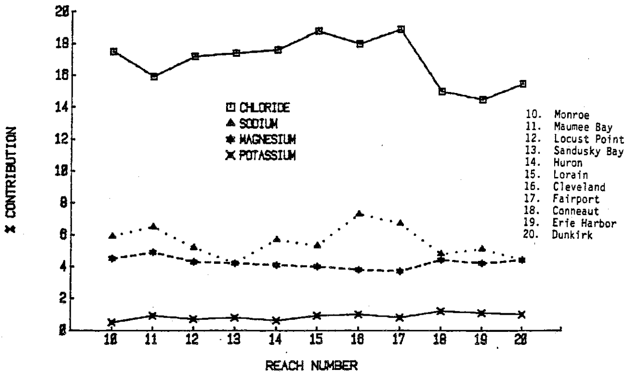
FIGURE 94. THE PERCENT CONTRIBUTION OF THE INDIVIDUAL PRINCIPAL IONS TO THE TOTAL CONDUCTANCE FOR EACH OF THE U. S. REACHES.
