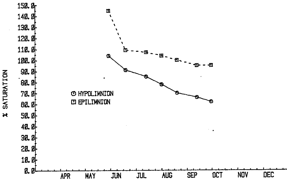
FIGURE 19. THE MEAN EASTERN BASIN DISSOLVED OXYGEN CONCENTRATIONS AND PERCENT SATURATIONS FOR 1978 CCIW - NWRI.
