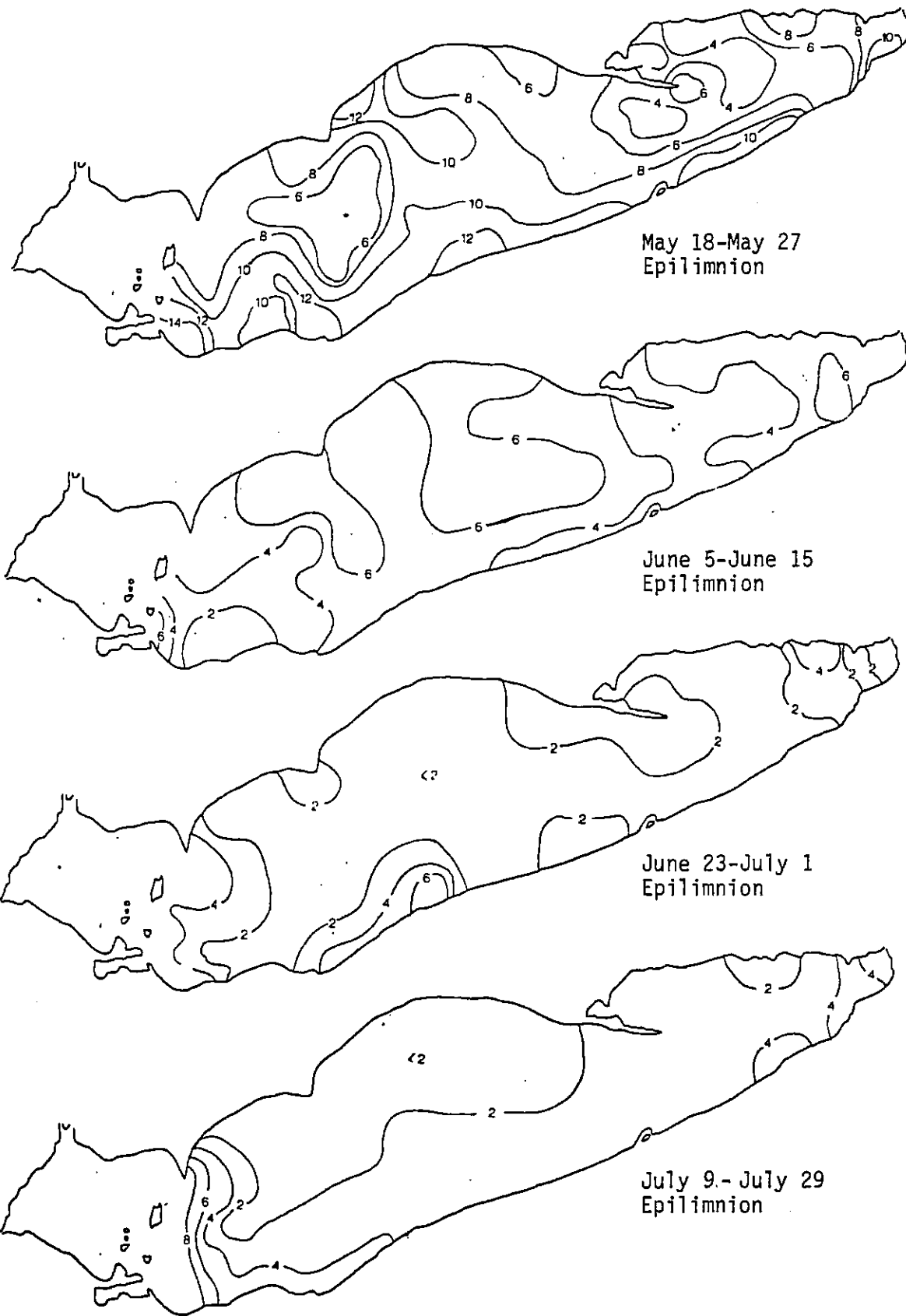
FIGURE 41. THE SEASONAL EPILIMNION CORRECTED CHLOROPHYLL a ( \mu\text{g}/\text{l} ) DISTRIBUTION PATTERNS FOR THE CENTRAL AND EASTERN BASINS OF LAKE ERIE FOR 1978 (USEPA-GLNPO).
