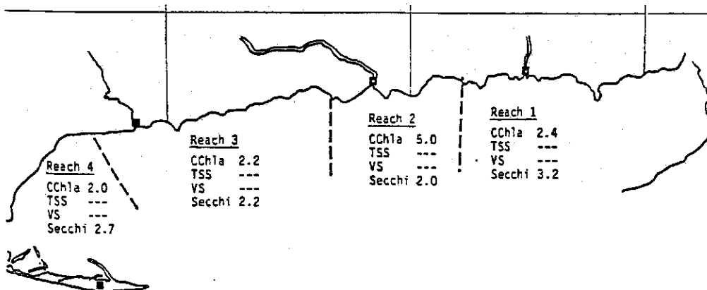
FIGURE 77. MEAN CONCENTRATIONS FOR THE 1978 AND 1979 NEARSHORE DATA BASE SUMMARIZED FOR EACH DESIGNATED REACH AREA.
