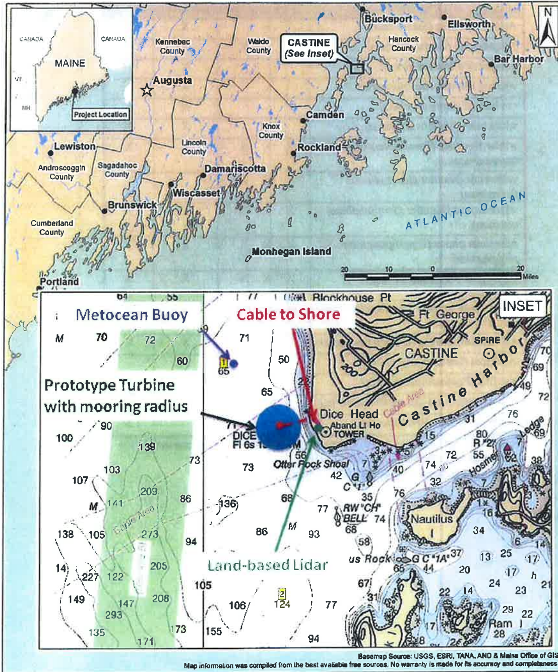
FIGURE 1 PROPOSED LOCATION OF DEPLOYMENT OF FLOATING OFFSHORE WIND TURBINE PLATFORM.
