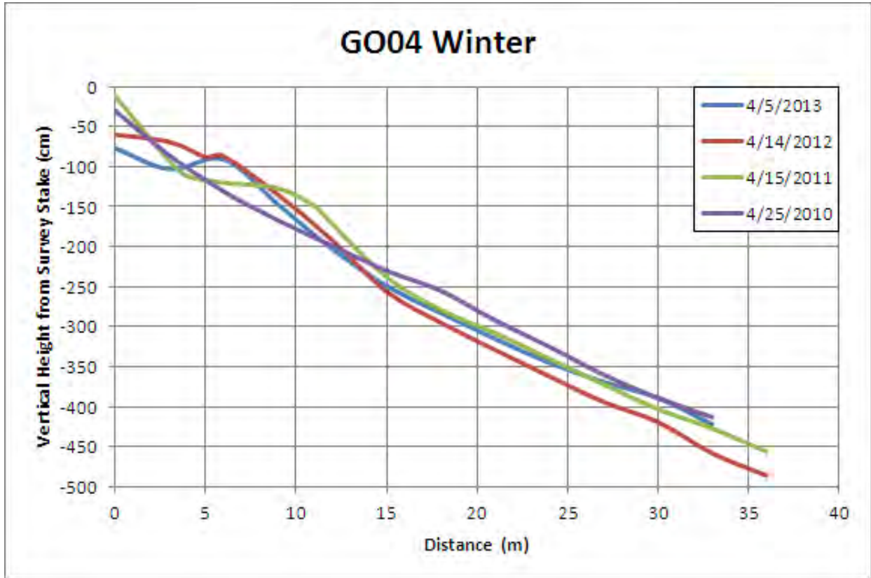
Figure 70. Winter beach profiles for GO04 from 2010, 2011, 2012, and 2013.
