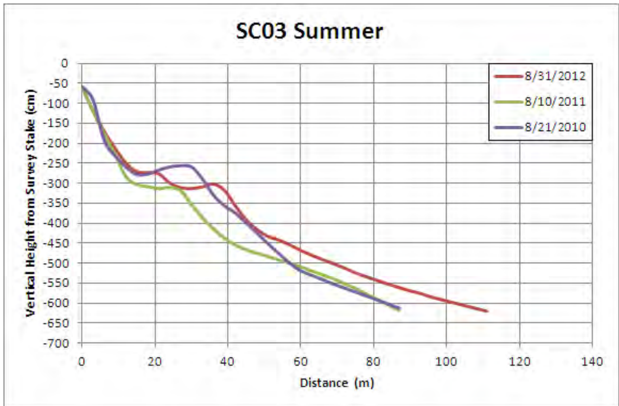
Figure 21. Summer beach profiles for SC03 from 2010, 2011, and 2012.
