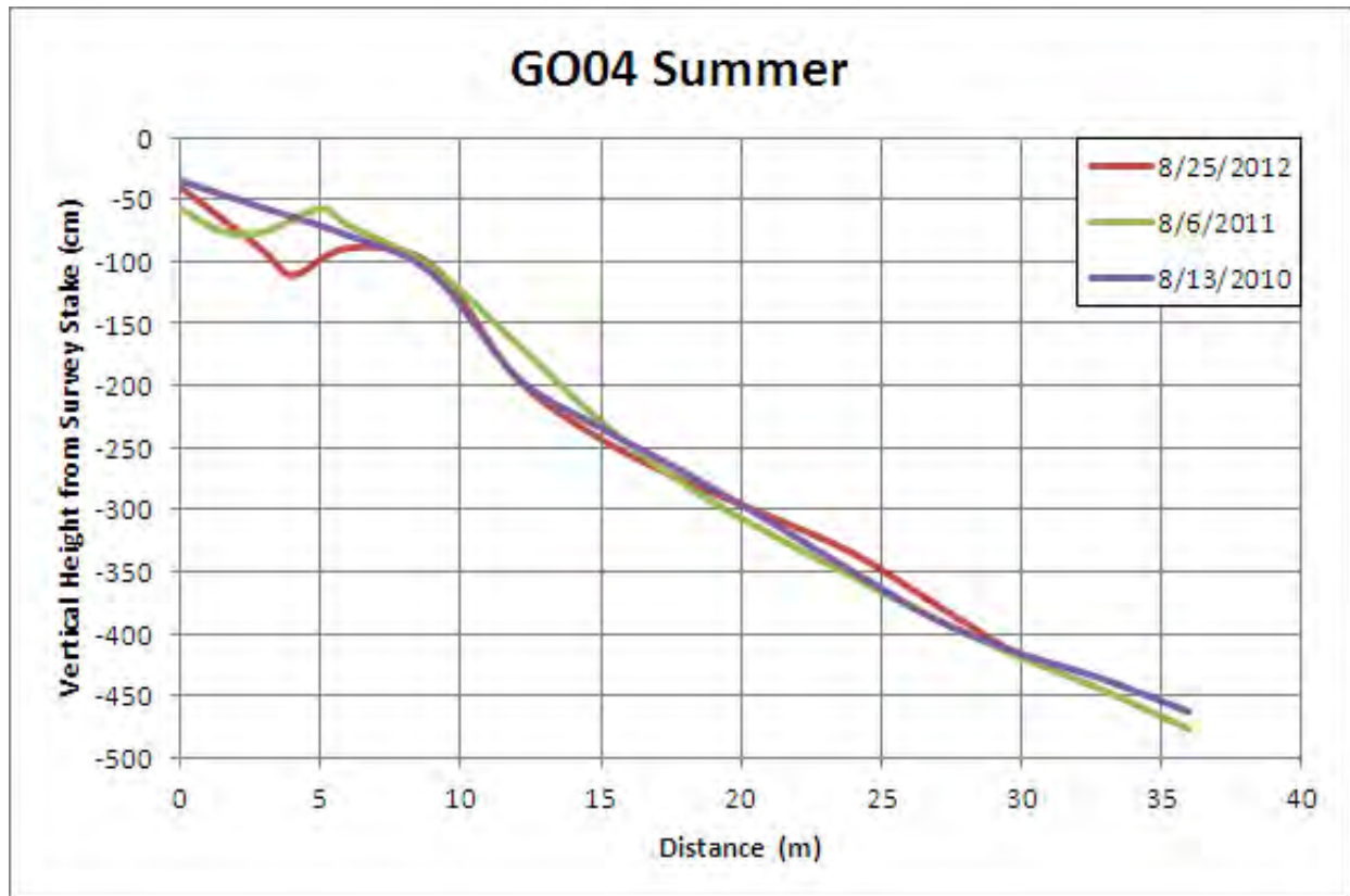
Figure 71. Summer beach profiles for GO04 from 2010, 2011, and 2012.
