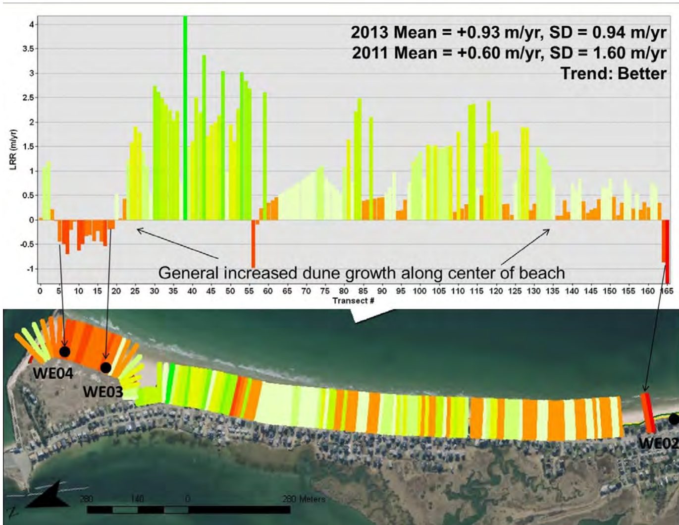
Figure 91. MBMAP shoreline change results along Wells Beach, Wells. Base imagery from Maine OGIS.
