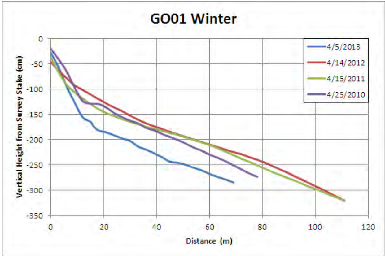
Figure 64. Winter beach profiles for GO01 from 2010, 2011, 2012, and 2013.
