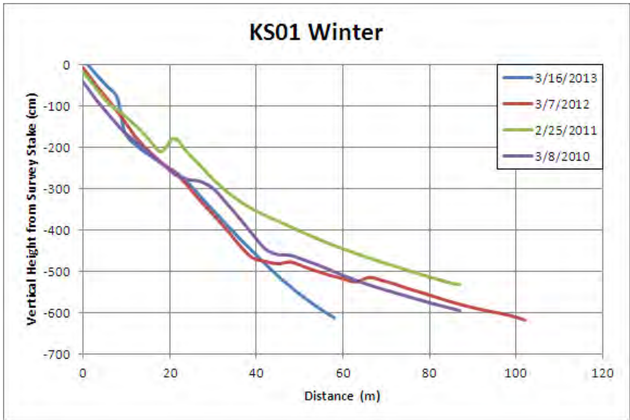
Figure 37. Winter beach profiles for KS01 from 2010, 2011, 2012, and 2013.
