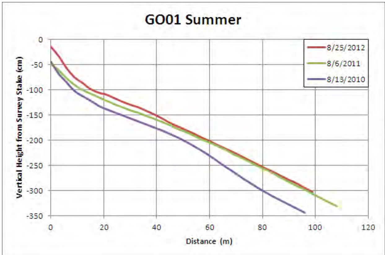
Figure 65. Summer beach profiles for GO01 from 2010, 2011, and 2012.
