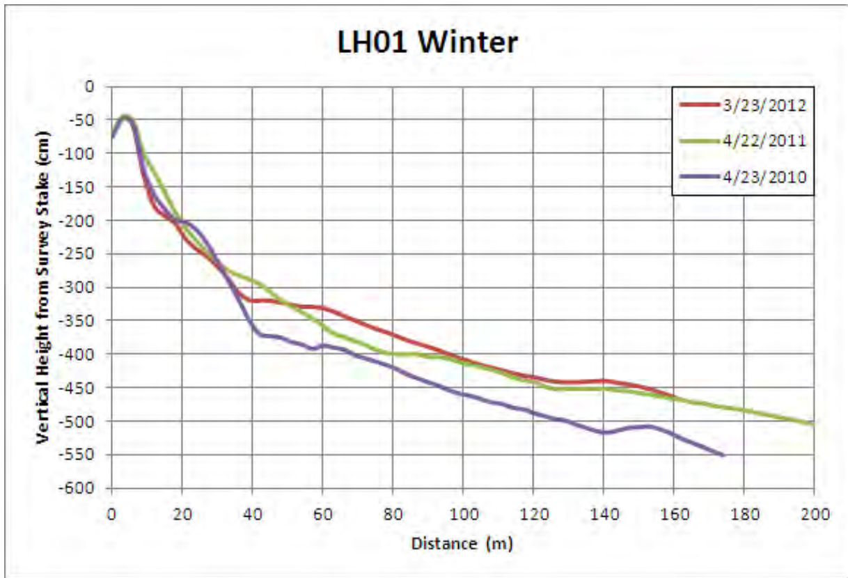
Figure 73. Winter beach profiles for LH01 from 2010, 2011, and 2012.
