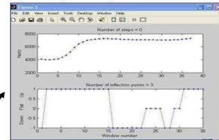
e) measured steps and inflection points (ROCCA)
