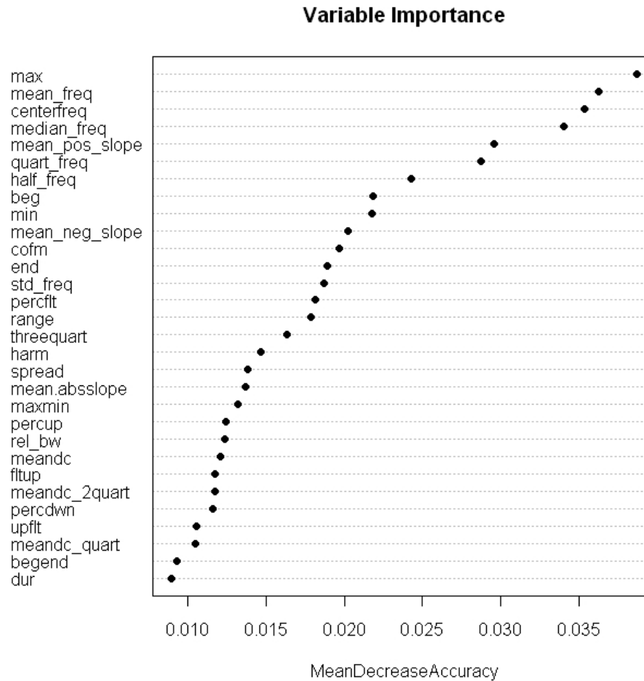
Figure 4. Plot showing the 30 most important variables in ROCCA’s random-forest classifier, starting with the most important variable at the top. Variables are given on the y-axis, and the relative importance (shown as a Mean Decrease Accuracy after variable randomization) is given on the x-axis. Full description of the variables are given in Appendix A.
