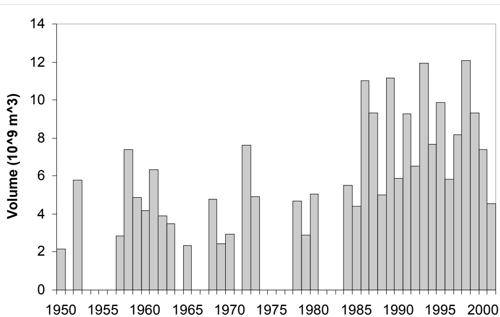
Figure 1. Estimates of Chesapeake Bay hypoxic volume during 1949-2001 (Hagy et al. 2004). Blanks are missing values.
