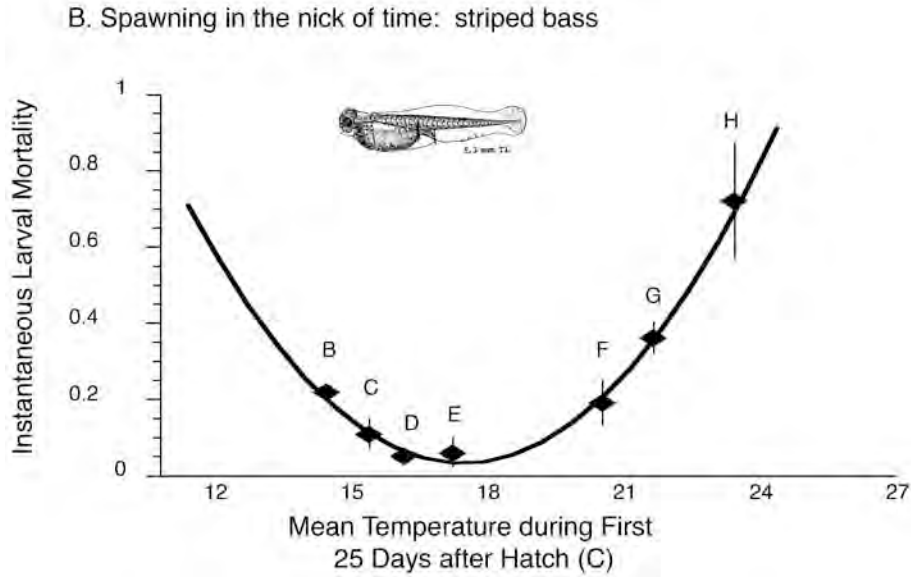
Figure 3. Relationship larval mortality and temperature experienced during the first 25 days after life. Weekly cohorts denoted by letters. Note that optimal larval survival conditions occur in the midst of the larval production season for cohorts C, D, and E. Data from Patuxent River estuary, 1991; Secor and Houde 1995.
