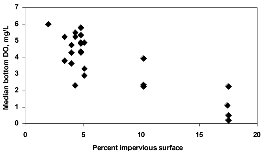
Figure 2. Plot of annual median dissolved oxygen during July-September and percent impervious surface for Chesapeake Bay tributaries sampled during 2003-2005 (Uphoff et al. submitted).
