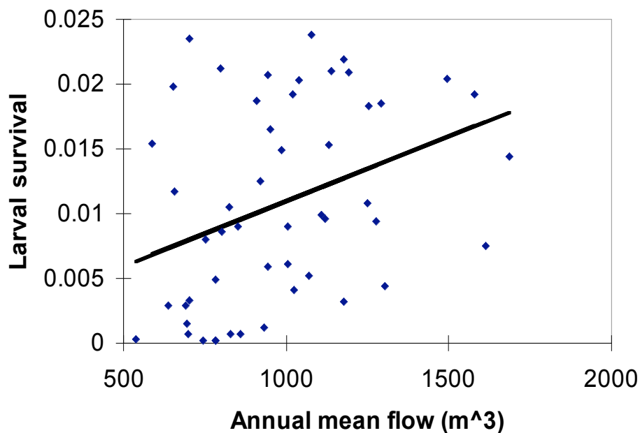
Figure 1. Plot of 1957-2005 observed and predicted Head-of-Bay annual striped bass egg-larval survival estimates and USGS annual mean Susquehanna River flow at Harrisburg, PA ( r^2 = 0.12 , P = 0.01 ).
