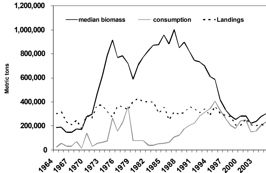
Figure 4. Estimated menhaden biomass and estimated biomass of menhaden consumed by striped bass from a logistic surplus production model that included a Type III striped bass predation function. Landings were an input into the model.
