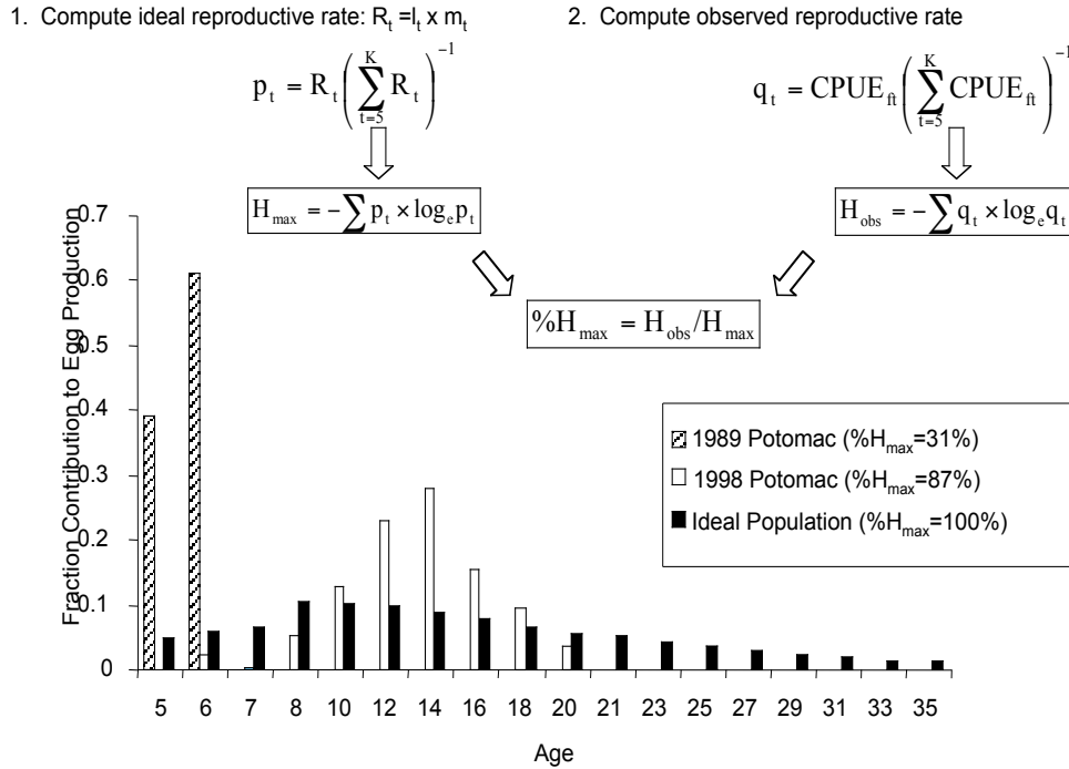
Figure 6. Age diversity index based upon age-specific reproductive rates.
