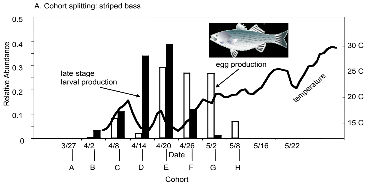
Figure 2. Relationship between weekly egg production, temperature and subsequent survival of striped bass larvae. Weekly cohorts denoted by letters. Data from Patuxent River estuary, 1991; Secor and Houde 1995.
