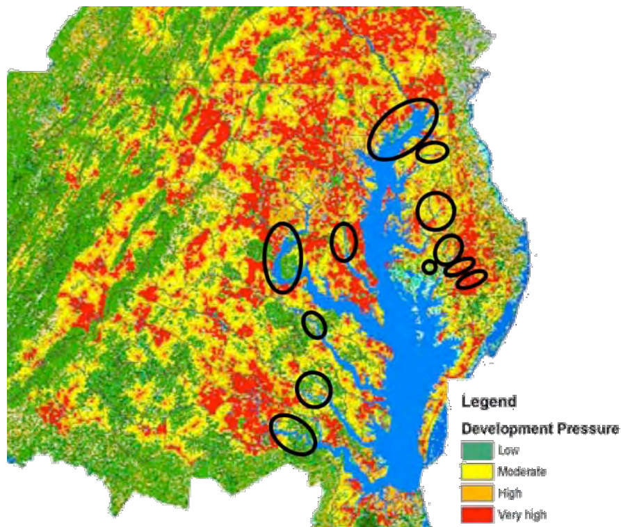
Figure 1. U.S. Geological Survey Projections of development pressure (prepared for the Chesapeake Bay Program) with ovals indicating striped bass spawning areas. Two lower Eastern Shore ovals may contain multiple spawning areas.
