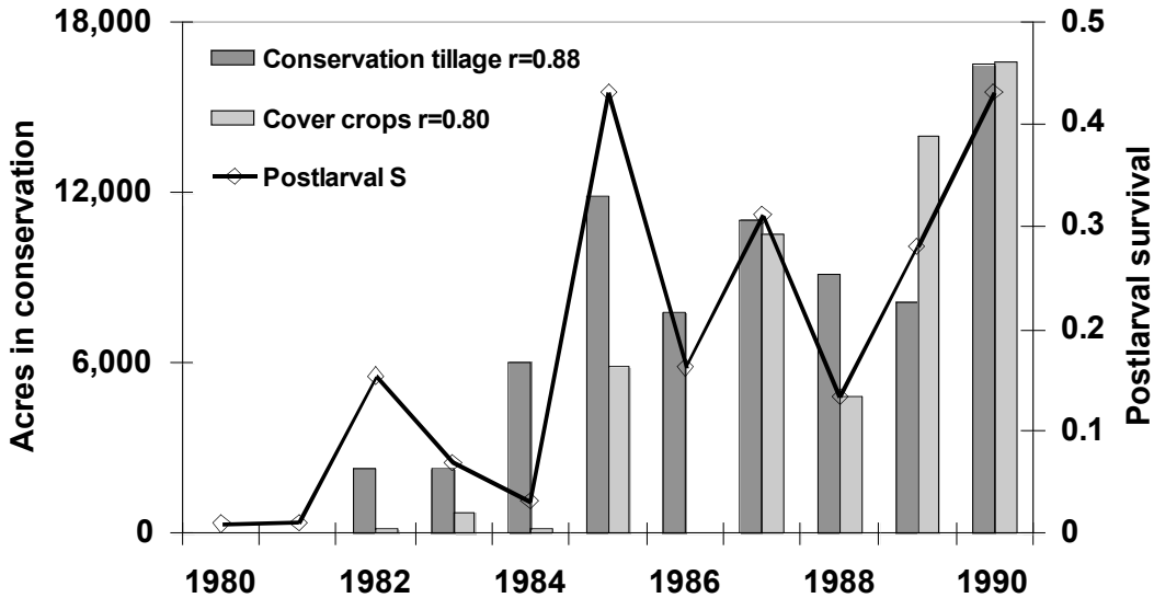
Figure 1. Trends in Choptank River striped bass postlarval survival and acreage of agricultural best management practices (BMP) implemented in Caroline County, Maryland. Correlation coefficients of BMPs and larval survival are reported next to BMP keys.
