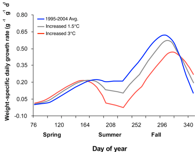
Figure 5. The effect of different seasonal temperature regimes on juvenile striped bass growth rates during the first year of life. Simulations were run using the Wisconsin bioenergetics model for three different seasonal temperature trends including (1) the average daily temperatures in upper Chesapeake Bay for the years 1995-2004, (2) an increase of 1.5°C above average temperatures, and (3) an increase of 3°C Celsius above the average.
