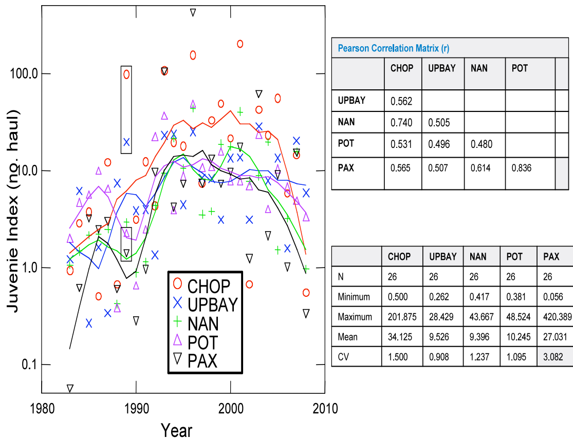
Figure 1. Temporal patterns of covariance in juvenile abundance among Maryland sub-estuaries. Left panel shows smoothed Lowess trends in juvenile production by system. Rectangles highlight production in 1989 (see text). Also shown are correlations between system pairs and inter-annual statistics for each system. Note that systems that are most proximate (PAX v. POT; NAN v. CHOP) show highest synchrony. Smaller systems tend to have higher coefficient of variation (CV) than larger systems.
