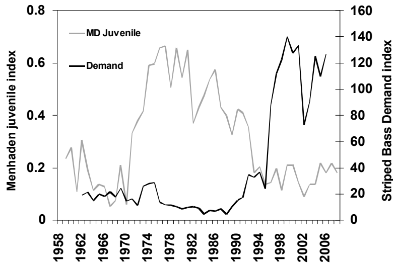
Figure 3. Index of relative demand for menhaden by striped bass and the Maryland menhaden juvenile index. Relative demand index is based on menhaden consumption per recruit * recruitment index (recruitment index = Maryland striped bass juvenile indices; demand index smoothed three years and projected three years forward). Menhaden juvenile index is proportion of seine hauls with menhaden.
