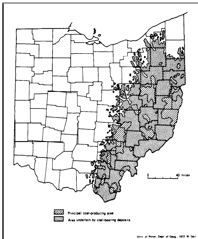
Figure 4. Coal deposits in Ohio (Brant and DeLong, 1960).
