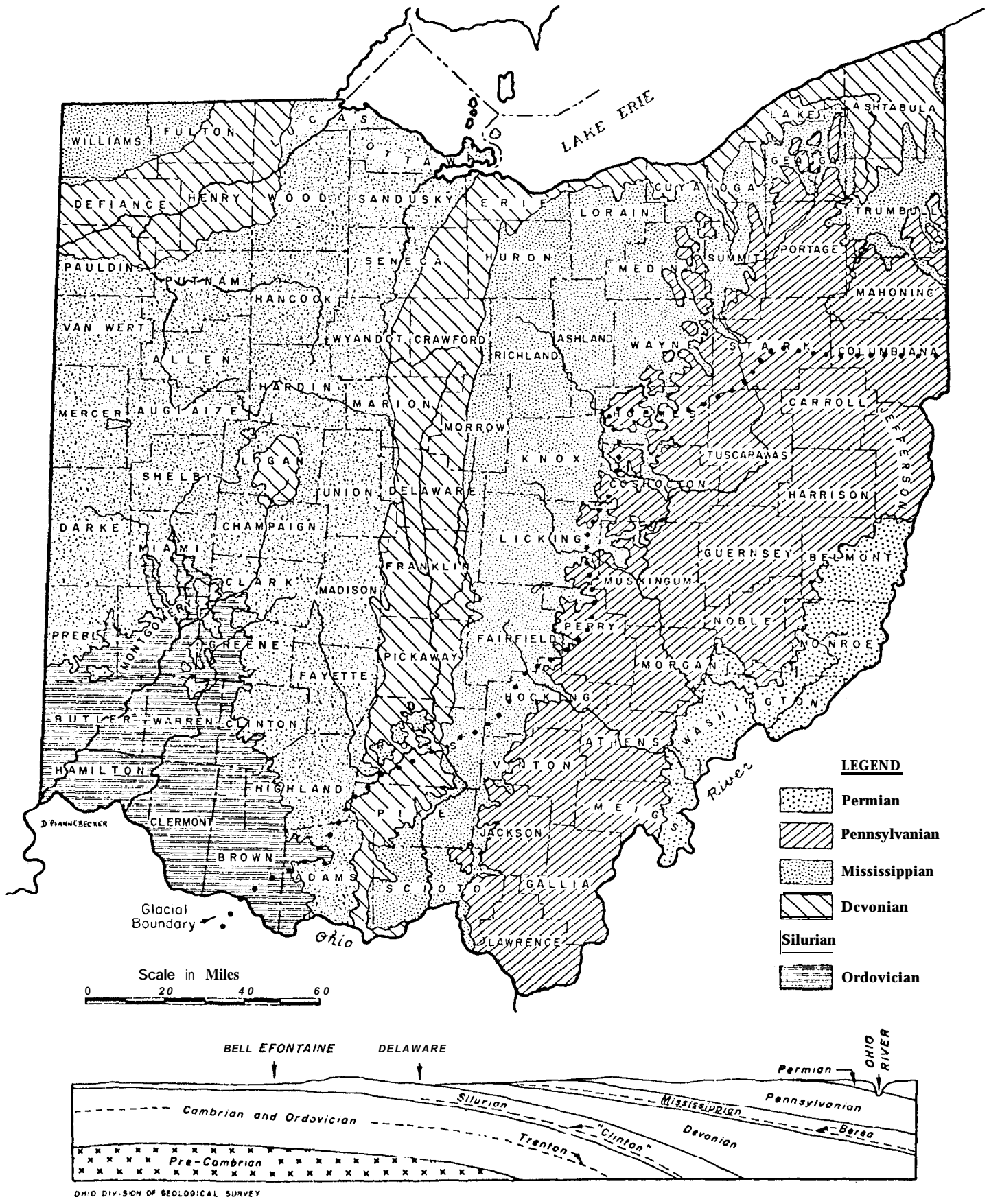
Figure 1. GEOLOGIC MAP OF OHIO
