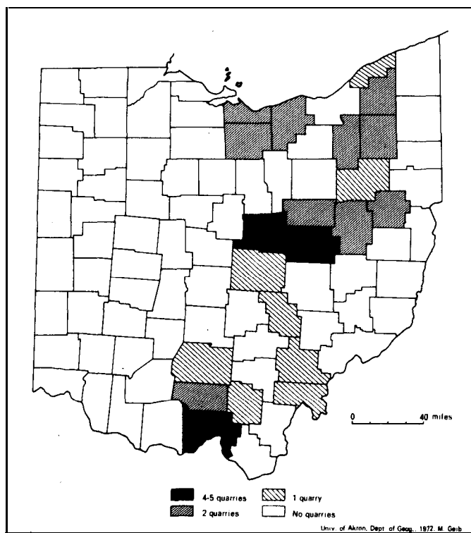
Figure 2. Active sandstone quarries (Ohio Division of Mines, 1970); no counties reported three active quarries.
