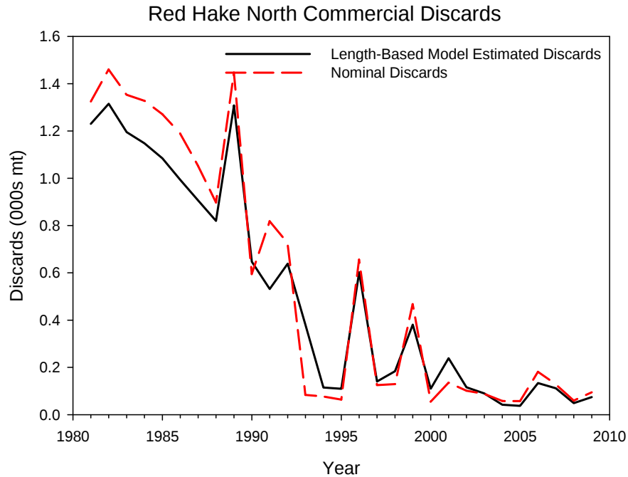
C11. Comparison of nominal discards with length-based model estimated discards of red hake from the northern stock. (Length-based estimates were not used in the assessment.)
