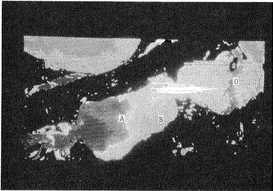
Figure 3. Categorized water colorant classes from the June 28, 1981 Landsat scene. Description of letter symbols is in the text.
