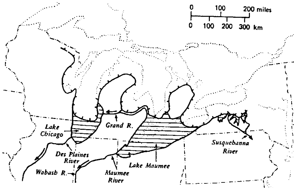
Figure 10. Lake Chicago and Lake Maumee stages (after Hough 1958).
