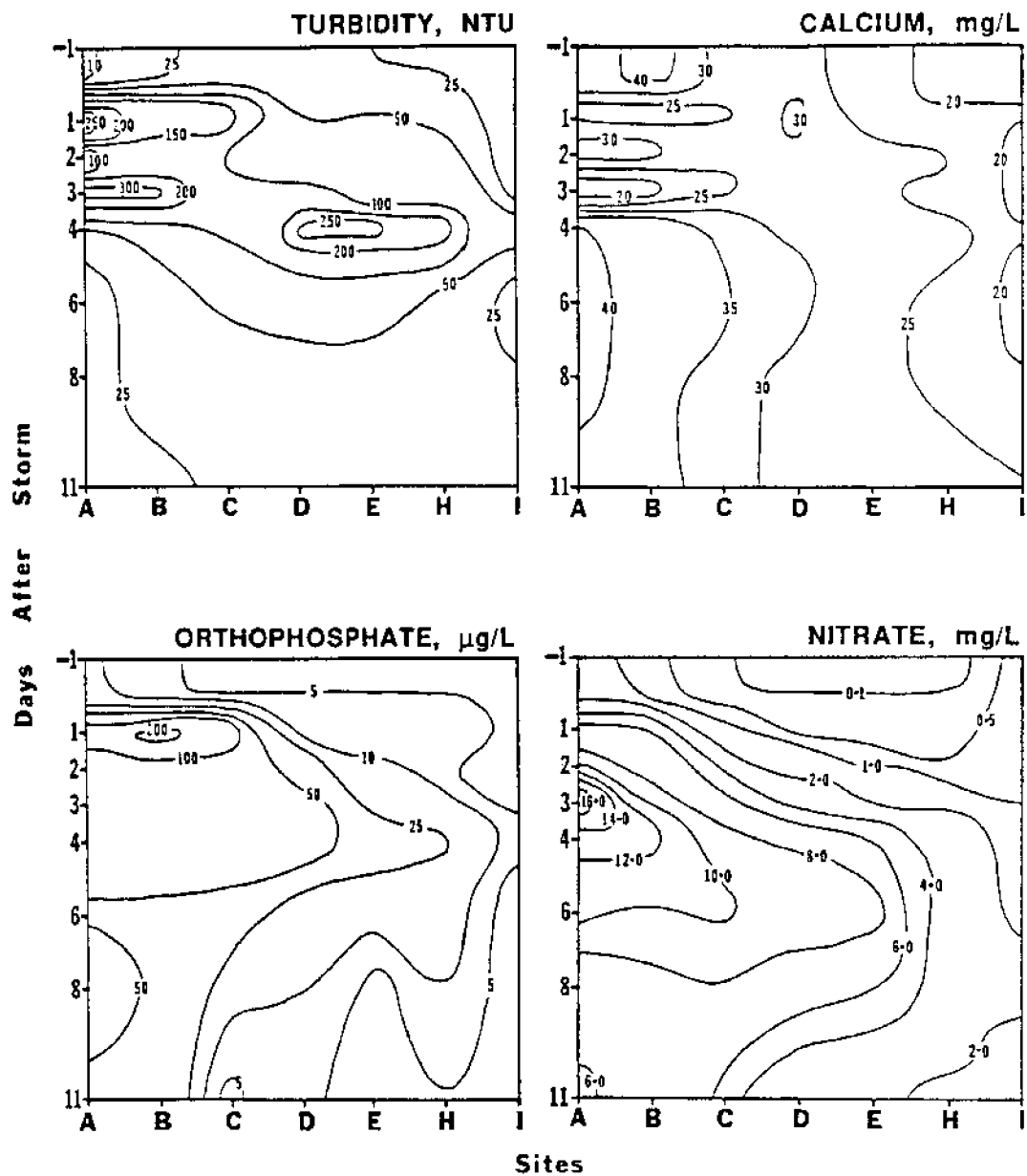
Figure 4. Temporal and spatial concentration patterns of turbidity, calcium, orthophosphate and nitrate following a May 1985 storm in the Old Woman Creek Wetland (modified from Klarer 1988). Site A is at the creek above the wetland, sites B-H are progressively downstream in the wetland, and site I is in the wave zone of Lake Erie about 100 m west of the wetland mouth.
