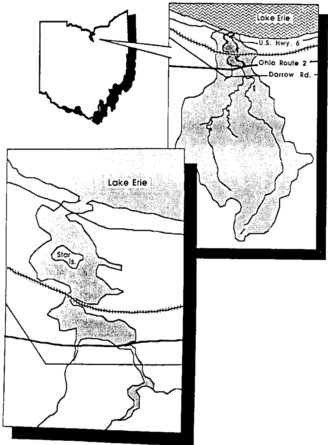
Figure 23. Old Woman Creek Estuary and watershed (after Reeder 1988).
