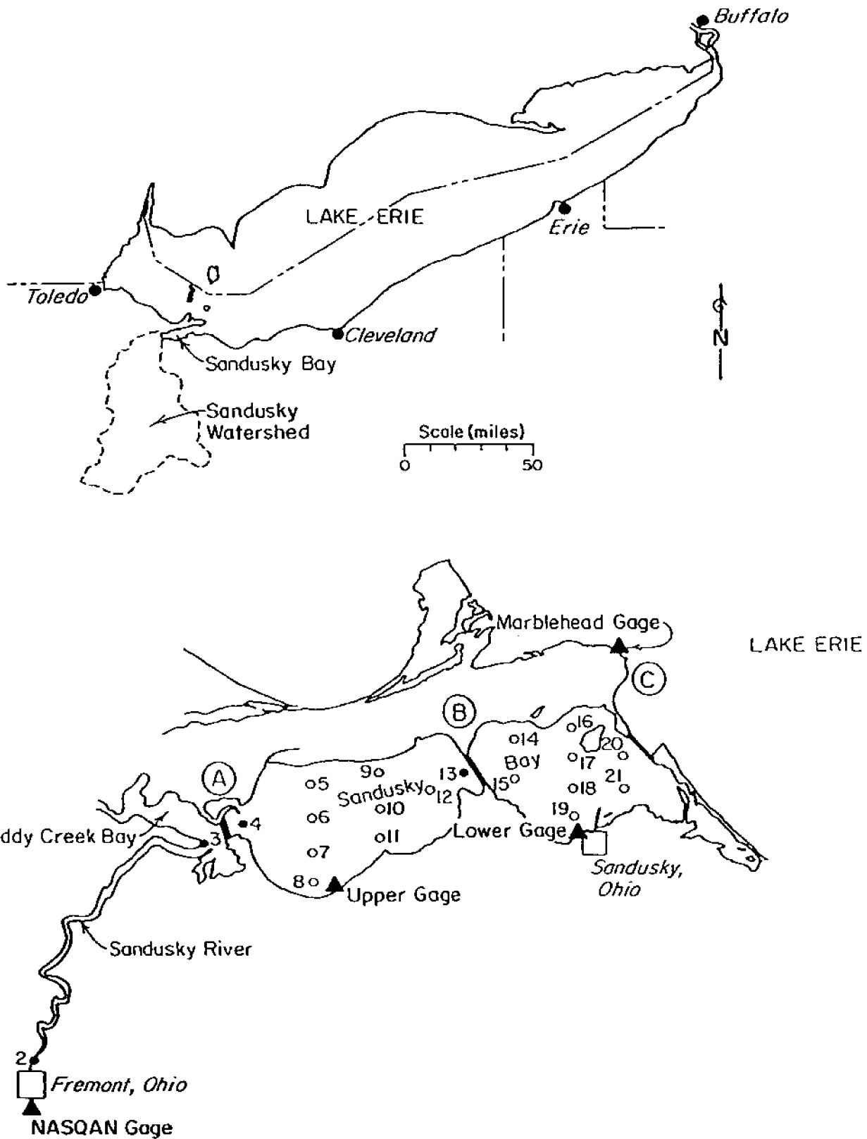
Figure 14. Sandusky Bay and transect location and data collection station definition map (Bedford and Mark 1988, and Richards and Baker 1982).
