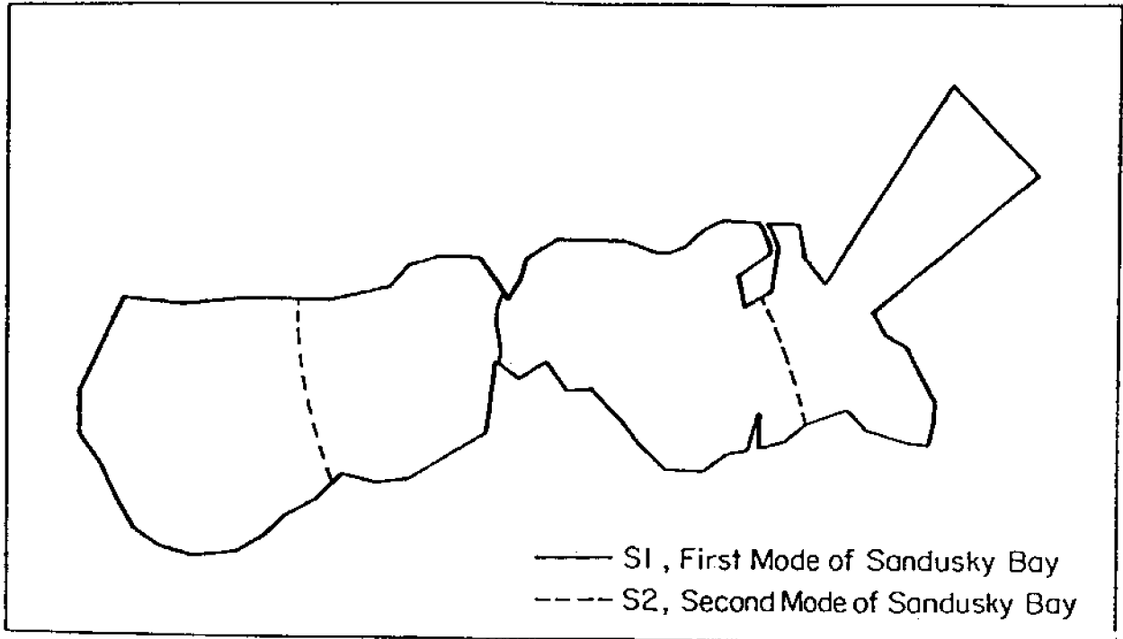
Figure 15. Null oscillation lines for the first (7.0 hour) and second (3.1 hour) Sandusky Bay free oscillation modes (Bedford et al. 1988).
