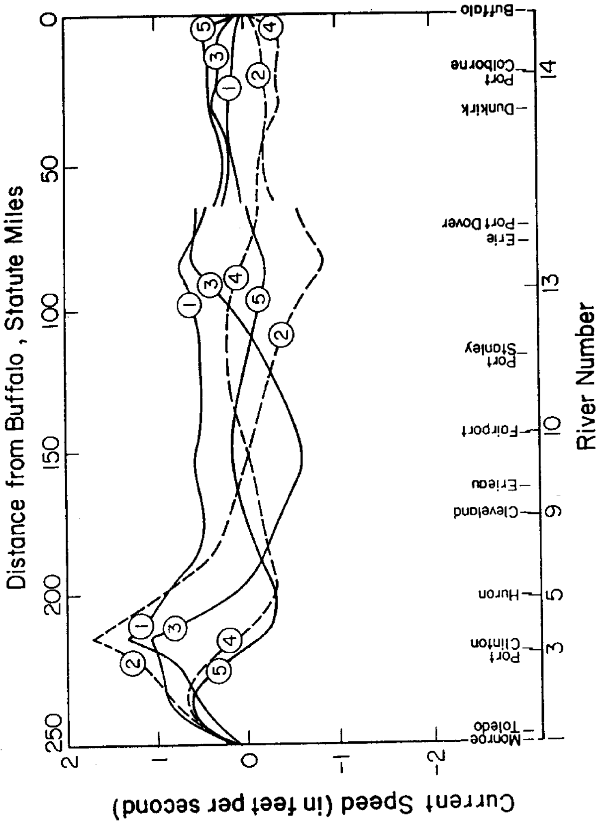
Figure 10c. Normalized current speeds for the first five Lake Erie modes (redrawn from Platzman and Rao 1964b).
