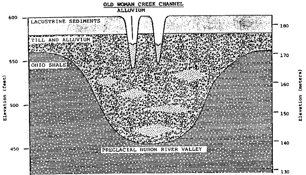
Figure 24. Geological cross-section of the Old Woman Creek estuary.
