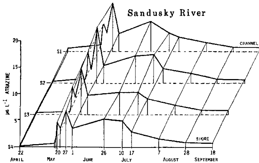
Figure 6. Changes in the concentrations of atrazine from April to September 1985 at four stations along a transect in Old Woman Creek Wetland (W1-W4) and a lower Sandusky River marsh (S1-S4). Stations W1 and S1 were in the stream channel; W4 and S4 were about 10 m from shore (Krieger 1986).
