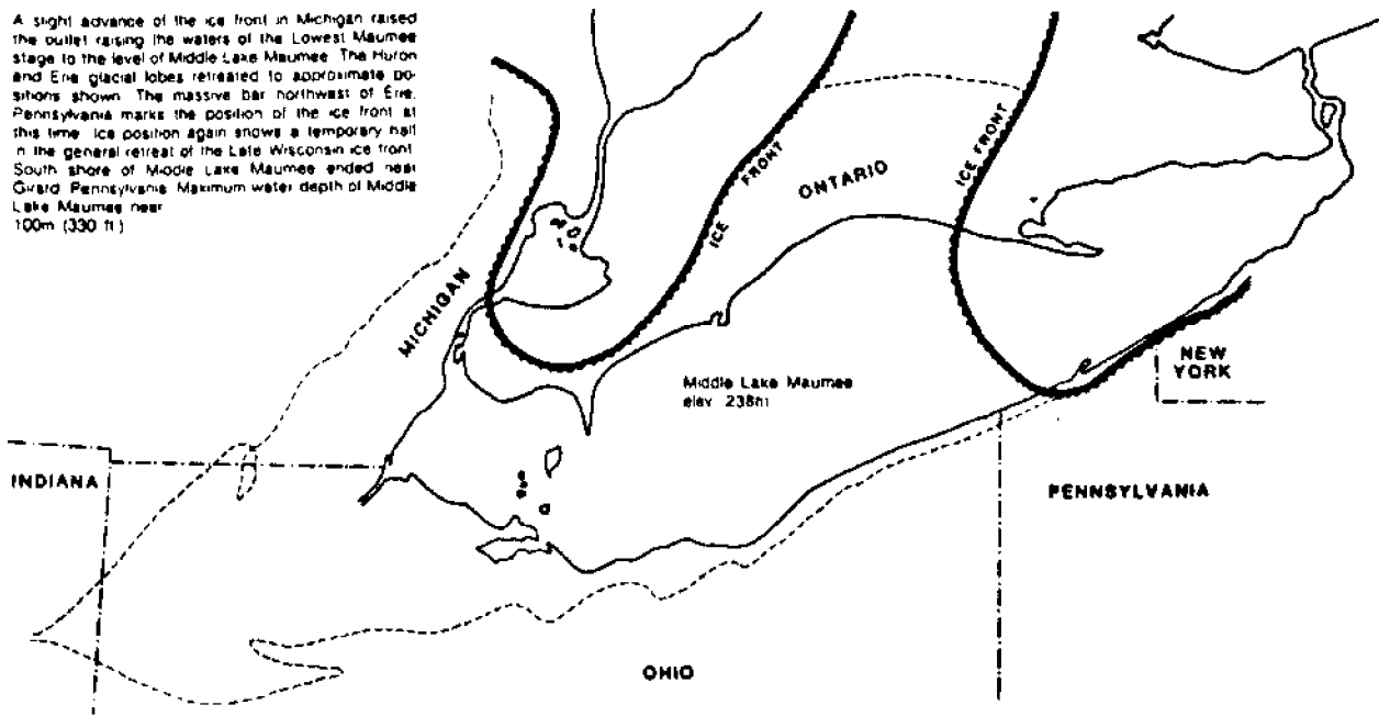
Figure 9. Middle Lake Maumee.
