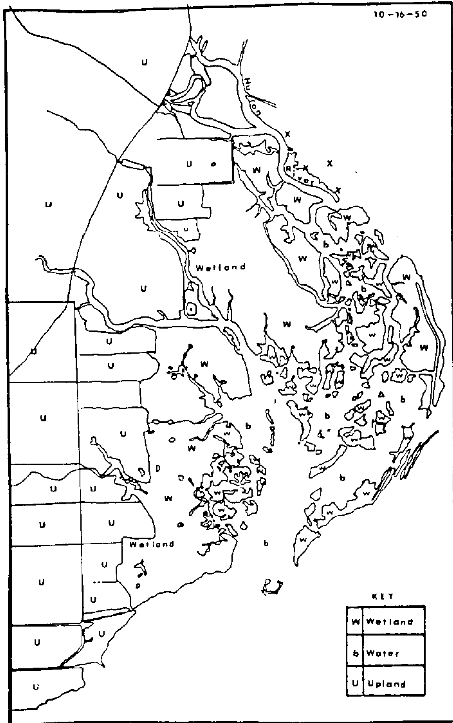
Figure 9. Interpretation of 1950 aerial photographs, Pointe Mouillee Area outside of the study area are shown as an 'x'.
