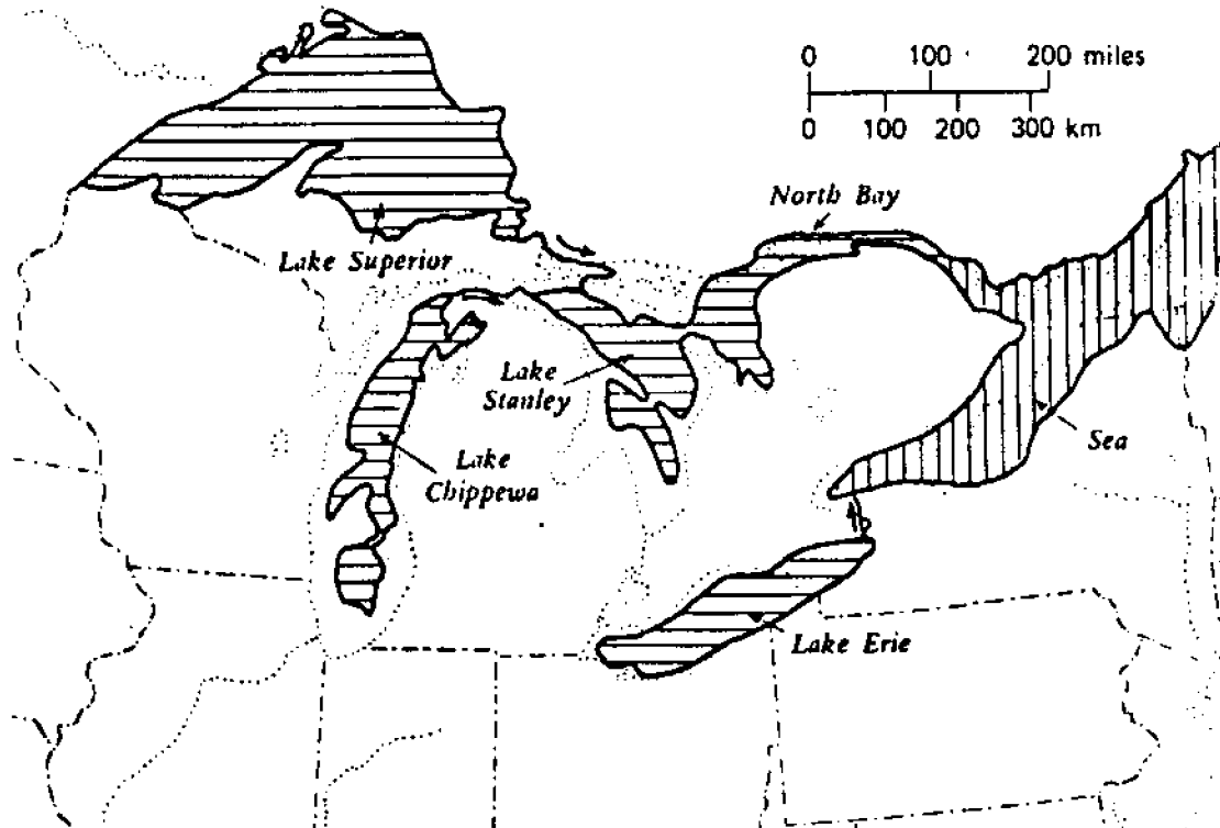
Figure 14. Lake Chippewa and Lake Stanley stages (after Hough 1958).
