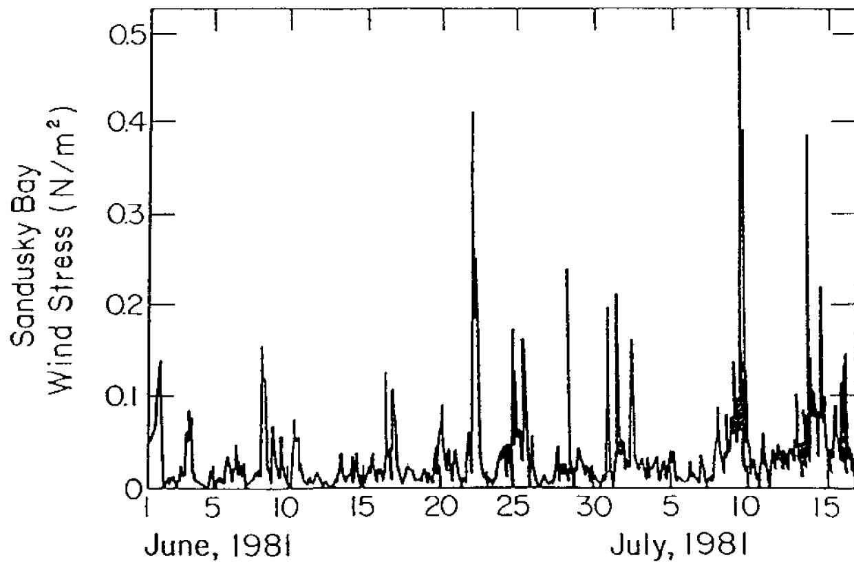
Figure 16b. Sandusky Bay wind shear time series (Bedford and Mark 1988).
