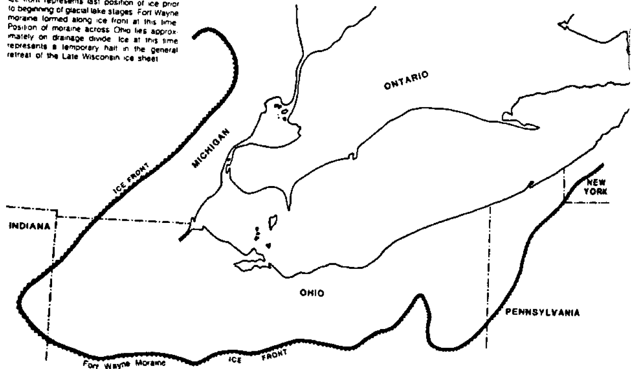
Figure 5. Pre-Maumee ice front.
