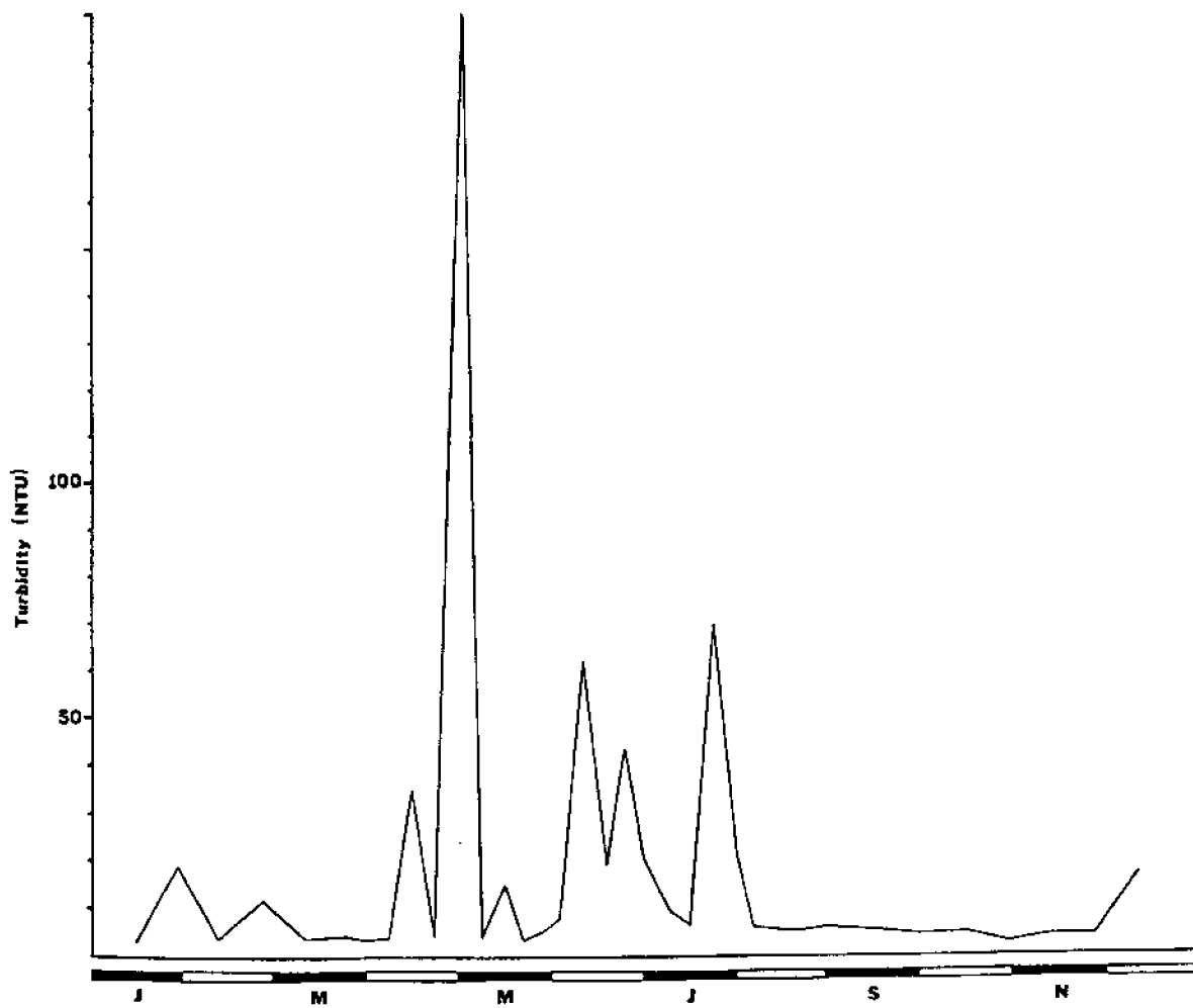
Figure 2. Seasonal pattern of turbidity (measured in NTU's) in Old Woman Creek estuary during 1980. (from Klarer, 1983)
