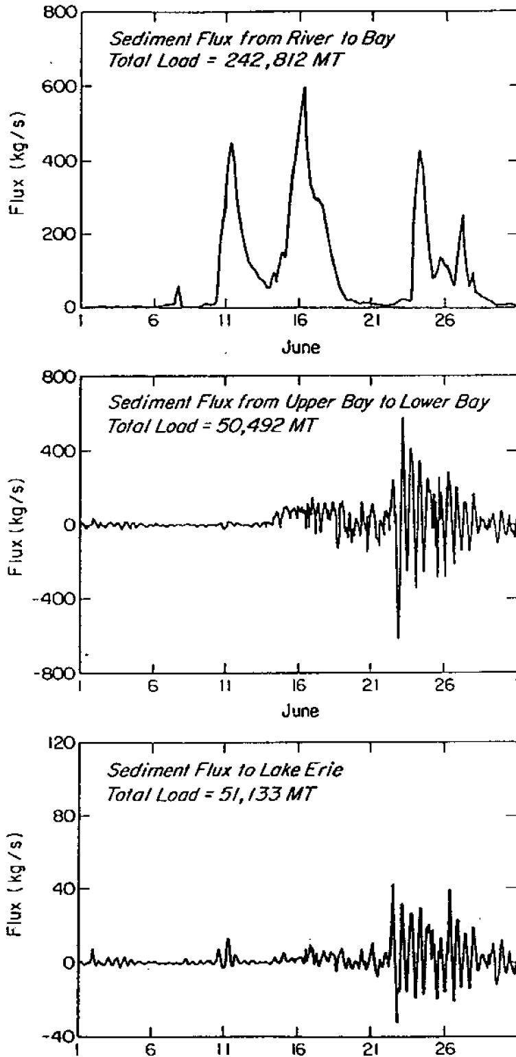
Figure 17. Sediment flux time series at three Sandusky Bay transects.
