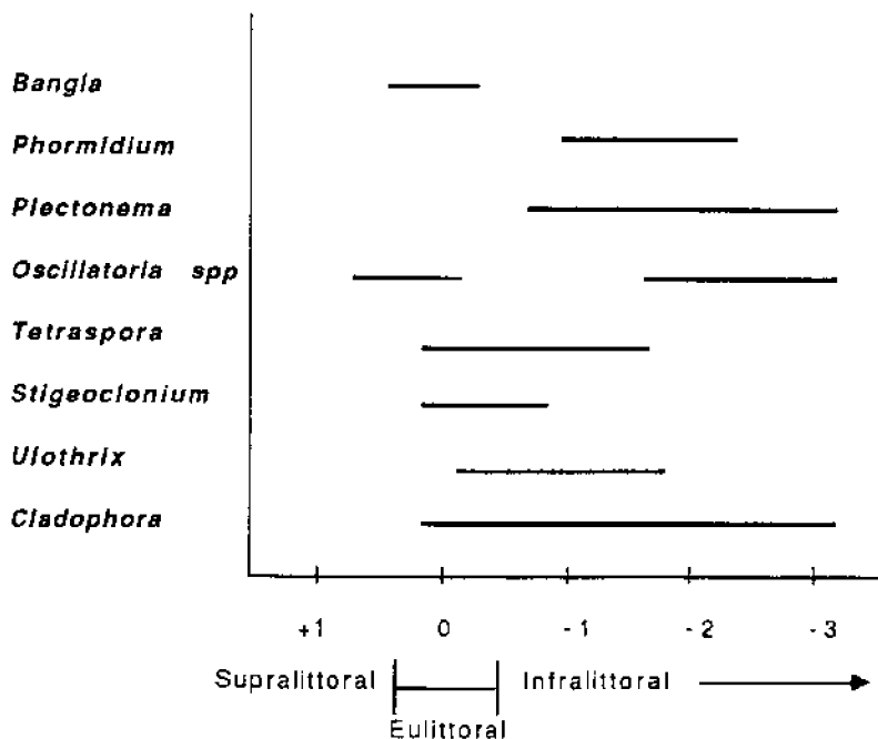
Figure 1. General zonation pattern of major attached algae in western Lake Erie.
