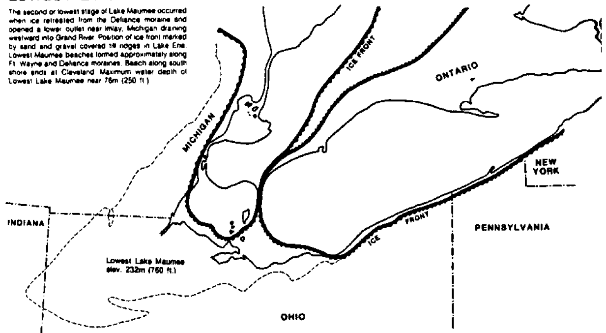
Figure 8. Lowest Lake Maumee.
