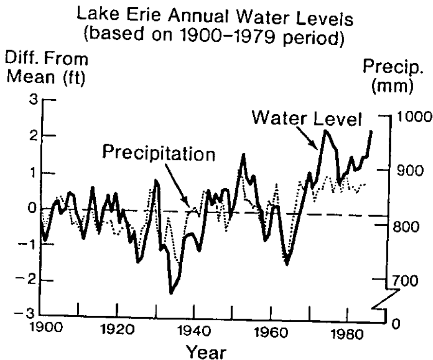
Figure 11. Comparison of Lake Erie annual water levels (from F. Quinn, Great Lakes Environmental Research Laboratory, NOAA; Carter 1986).
