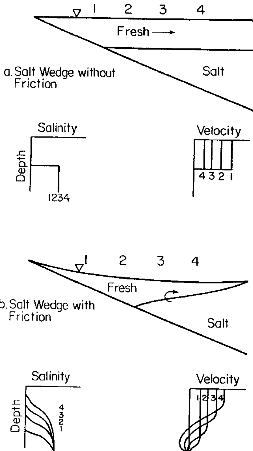
Figure 11a-e. Schematics of the five estuary density and velocity structures defined from Dyer (1973).
