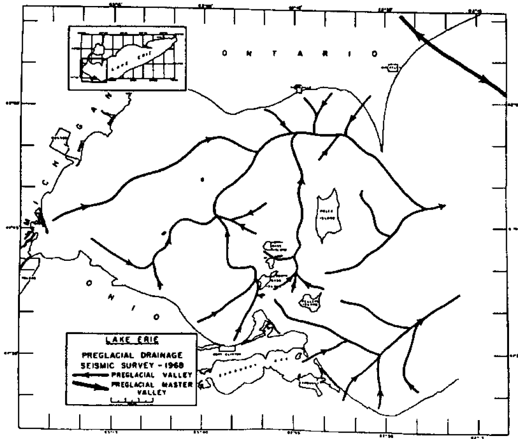
Figure 3. Preglacial drainage pattern of western Lake Erie Basin (after Hobson et al. 1969).
