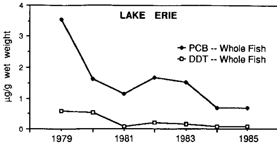
Figure 9. Trends for whole-fish tissue burdens of DDT and PCBs in Lake Erie (modified from Baumann and Whittle 1988).
