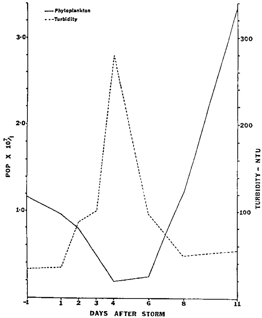
Figure 3. Changes in phytoplankton population numbers and turbidity (measured in NTU's) following a storm event in May, 1985.
