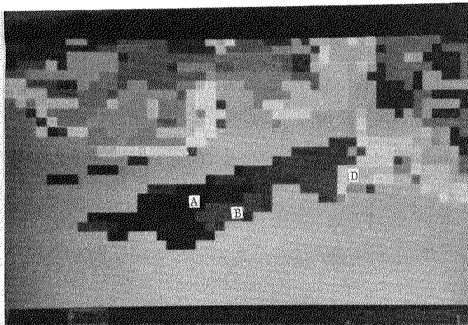
Figure 5. Categorized water colorant classes from the June 27 AVHRR scene.
