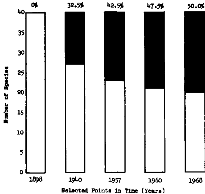
Figure 7. Graph showing loss in numbers and percentages of species from Put-in-Bay Harbor from 1898 (0% lost) to 1968 (50% lost).
