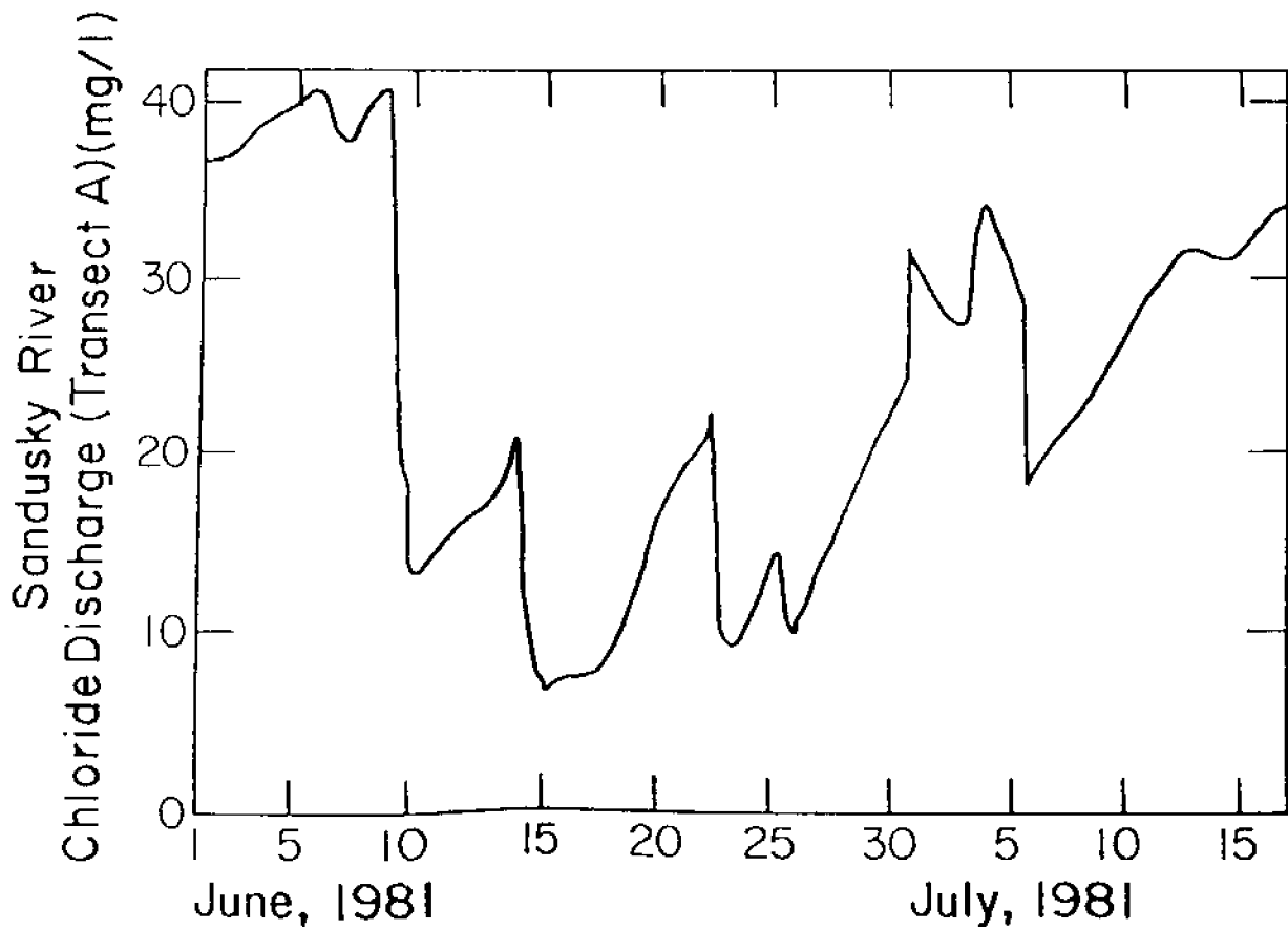
Figure 16d. Sandusky River chloride inflow time series (Bedford and Mark 1988).
