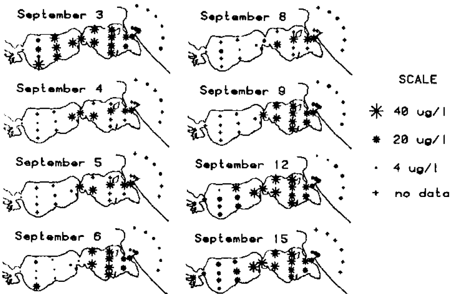
Figure 5. Concentration gradients in Sandusky Bay for soluble reactive phosphorus and chlorophyll a following a typical storm in September 1981 (modified from Richards and Baker 1985).
