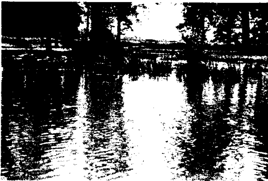
Figure 6. 1968. Aquatic plants in Squaw Harbor, Put-in-Bay, looking toward the southwest shoreline. Floating-leaved plants are absent from the foreground and only a few remaining cat-tails and sedges remain in the background. All of these plants disappeared from this location by the summer of 1970, following a rise of higher water level in early 1969. (photograph by Ronald L. Stuckey, 8 August 1968).
