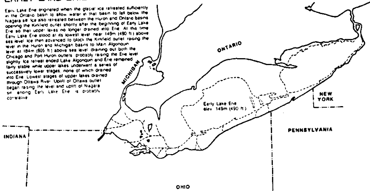
Figure 15. Early Lake Erie.
