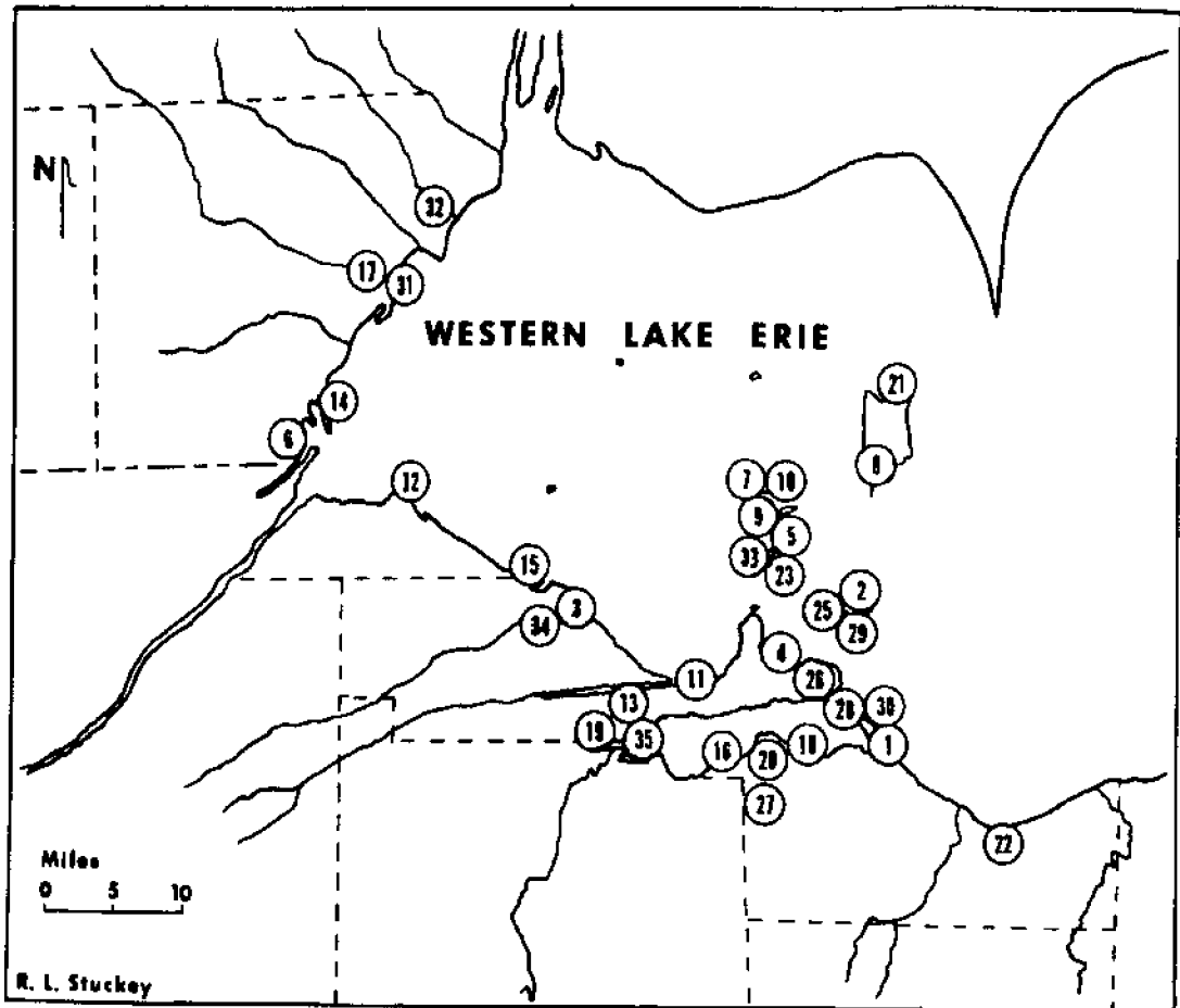
Figure 2. Map of western Lake Erie showing study localities by Ronald L. Stuckey and associates (1967-1987).
