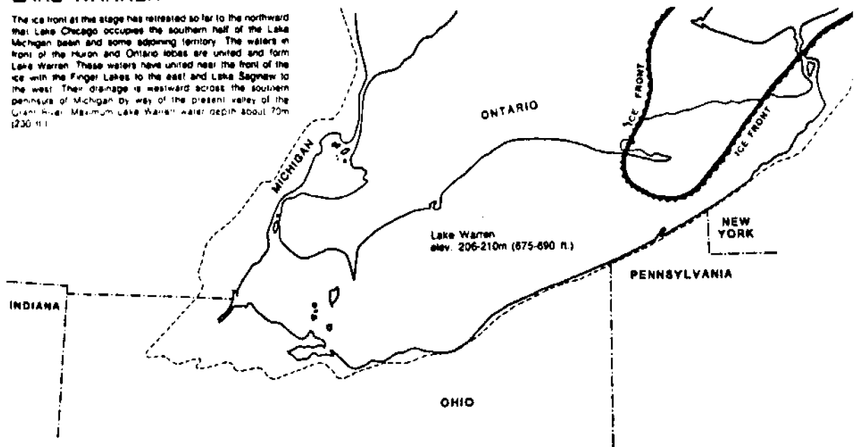
Figure 12. Lake Warren.
