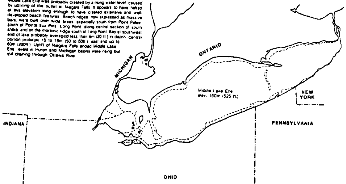
Figure 17. Middle Lake Erie.
