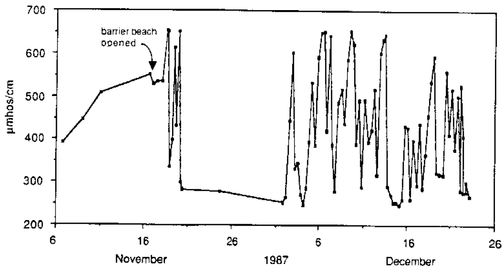
Figure 3. Oscillations in specific conductance (measured at 25°C) about 100 m upstream of the mouth of Old Woman Creek Wetland, revealing the frequent alternation of lake and marsh water masses in that region of the marsh (Krieger, unpubl.).
