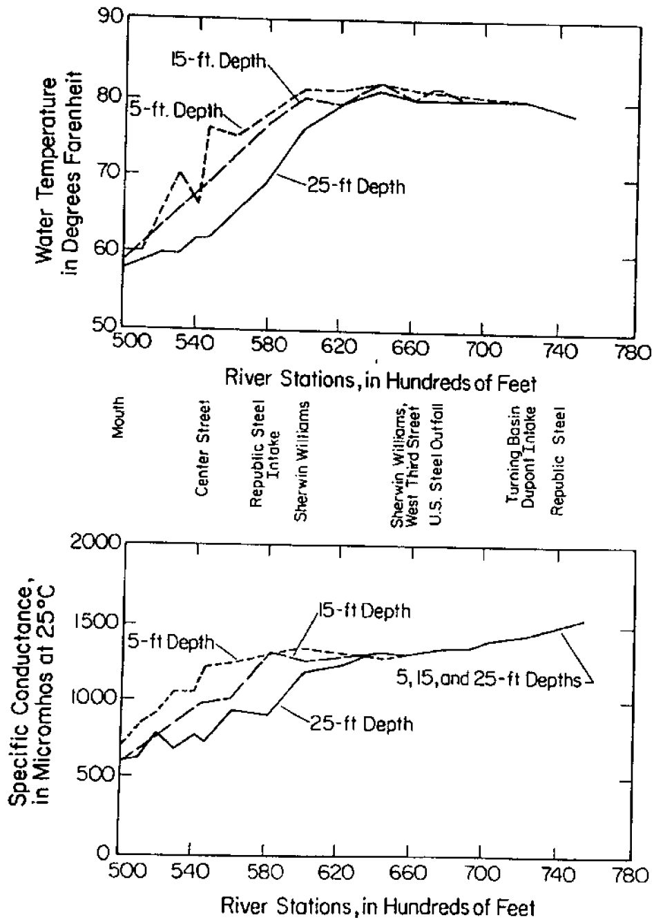
Figure 12b. Water temperature vs. station distribution in the Cuyahoga River at three depths, October 21, 1964 (redrawn from Schroeder and Collier 1966).
