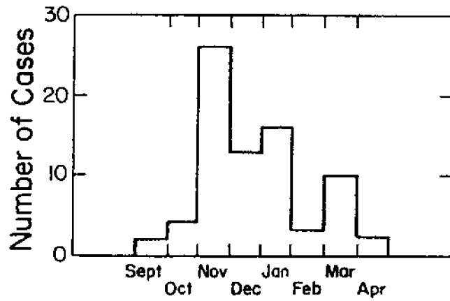
Figure 6b. Histogram of monthly setups in excess of six feet (redrawn from Pore et al. 1975).
