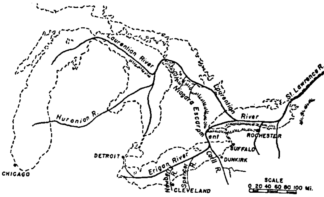
Figure 2. Preglacial drainage system of the Great Lakes region (after Spencer 1891).
