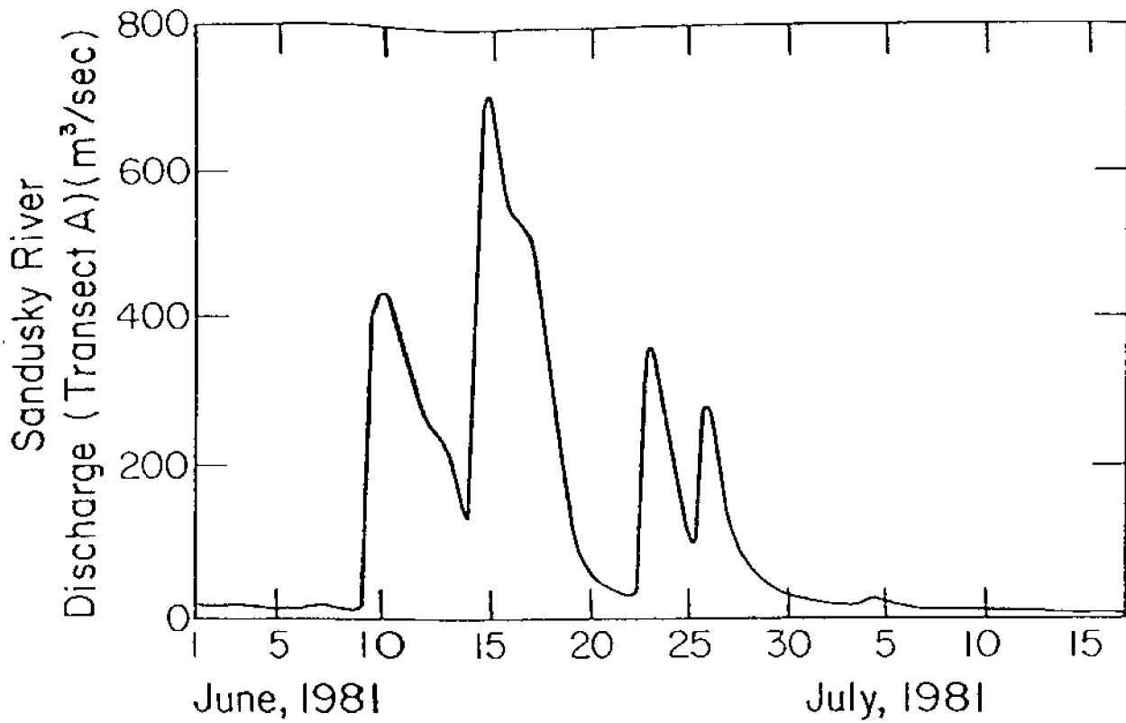
Figure 16c. Sandusky River discharge inflow time series (Bedford and Mark 1988).
