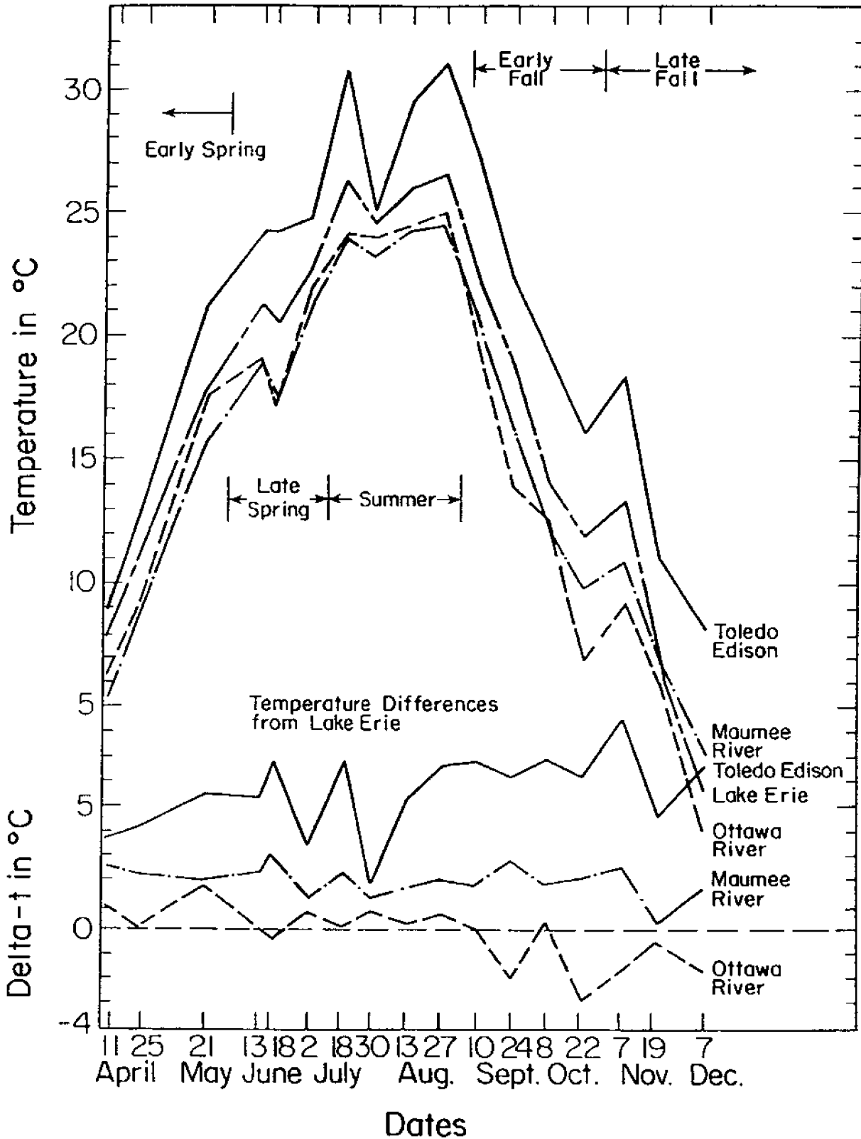
Figure 13. Maumee Bay/Ottawa River temperature variation over the year 1974 (redrawn from Fraleigh et al. 1975).
