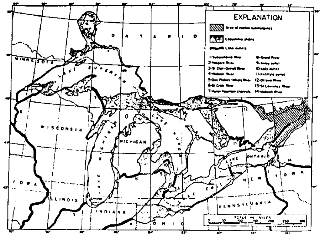
Figure 4. Outlets of the glacial lake stage in the Great Lakes Basin (after Leverett and Taylor 1915).
