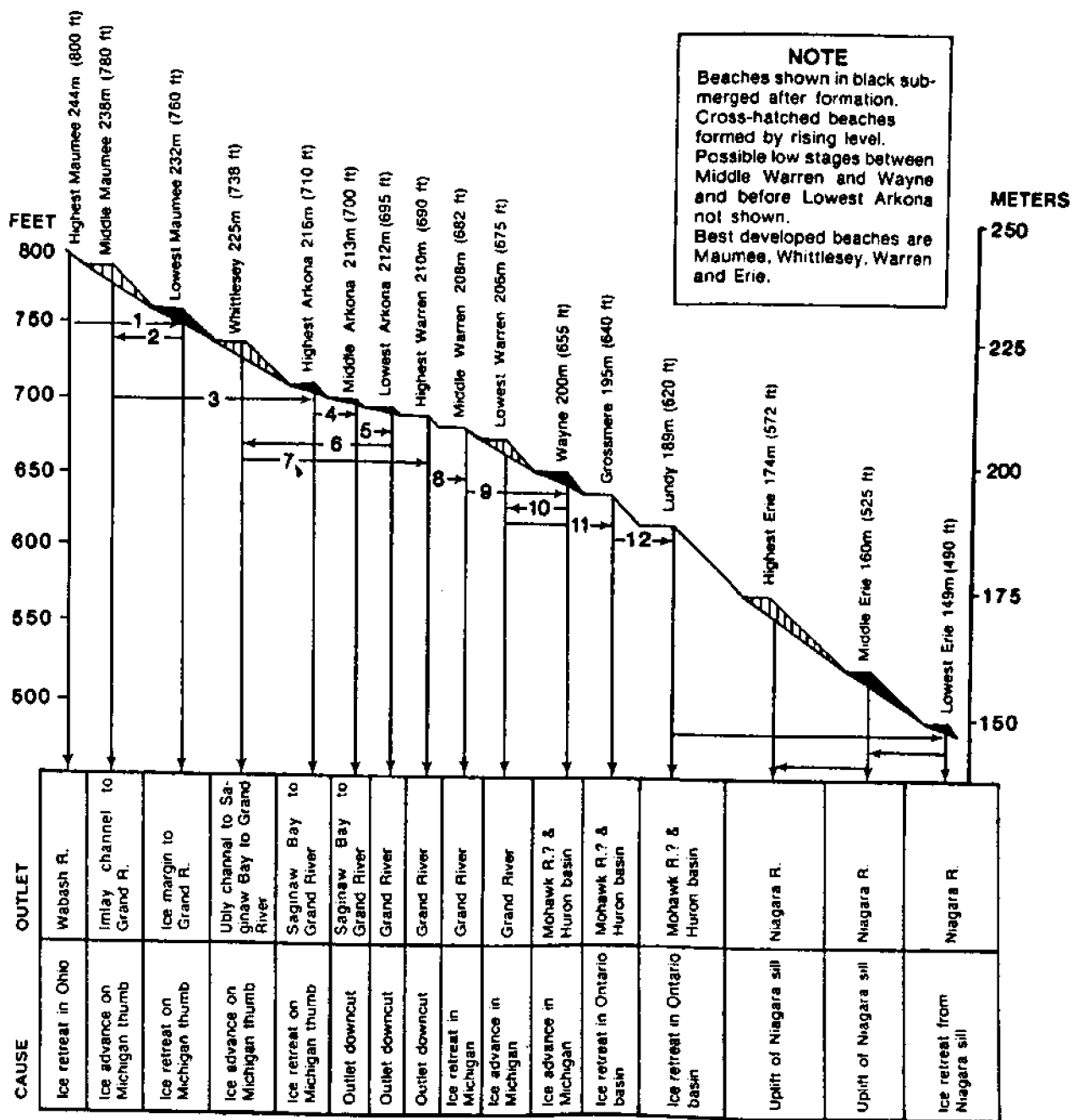
Figure 6. Chronology of glacial lake beach ridges in the Erie Basin.
