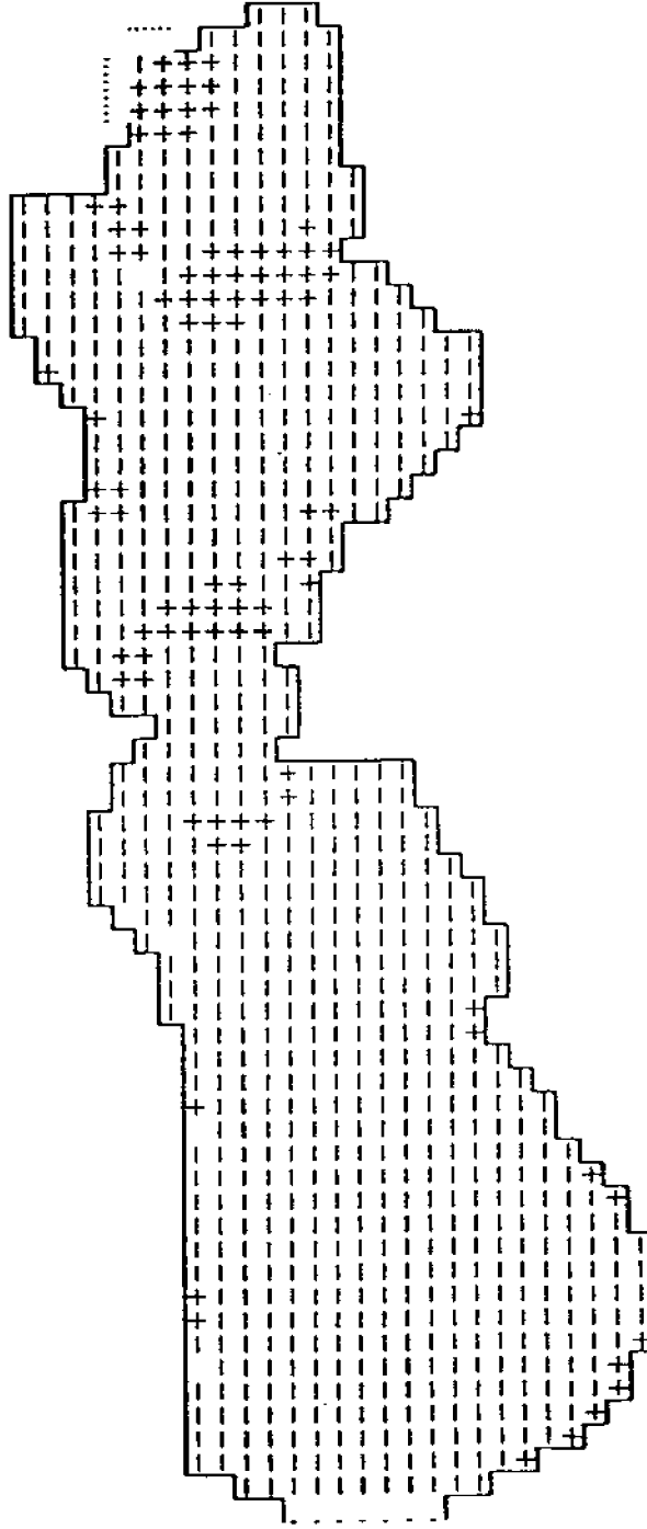
Figure 20. Net scour/deposition in Sandusky Bay, June 1 - July 13, 1981 (Bedford et al. 1988).
