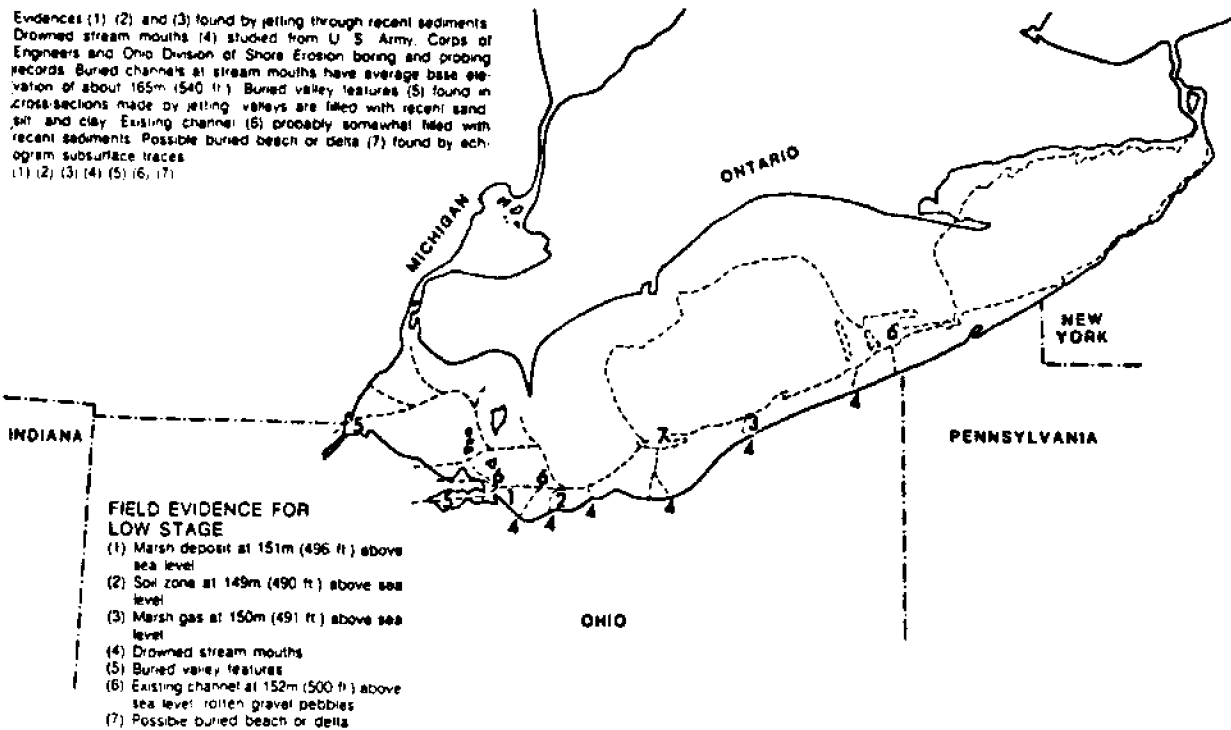
Figure 16. Early Lake Erie.
