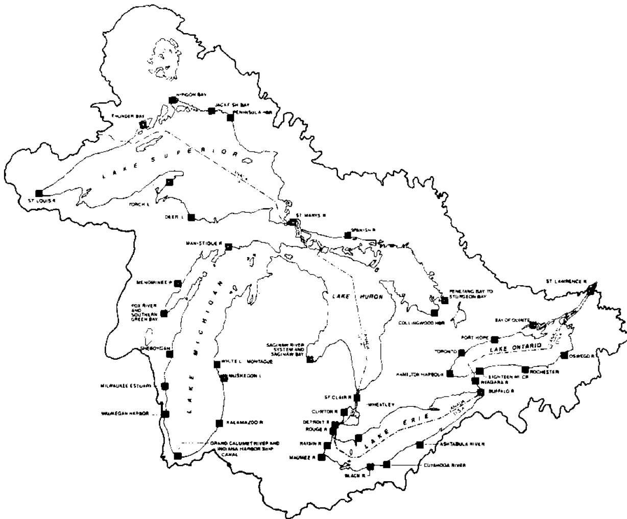
Figure 10. Areas of Concern in the Great Lakes Basin (Great Lakes Water Quality Board 1987).
