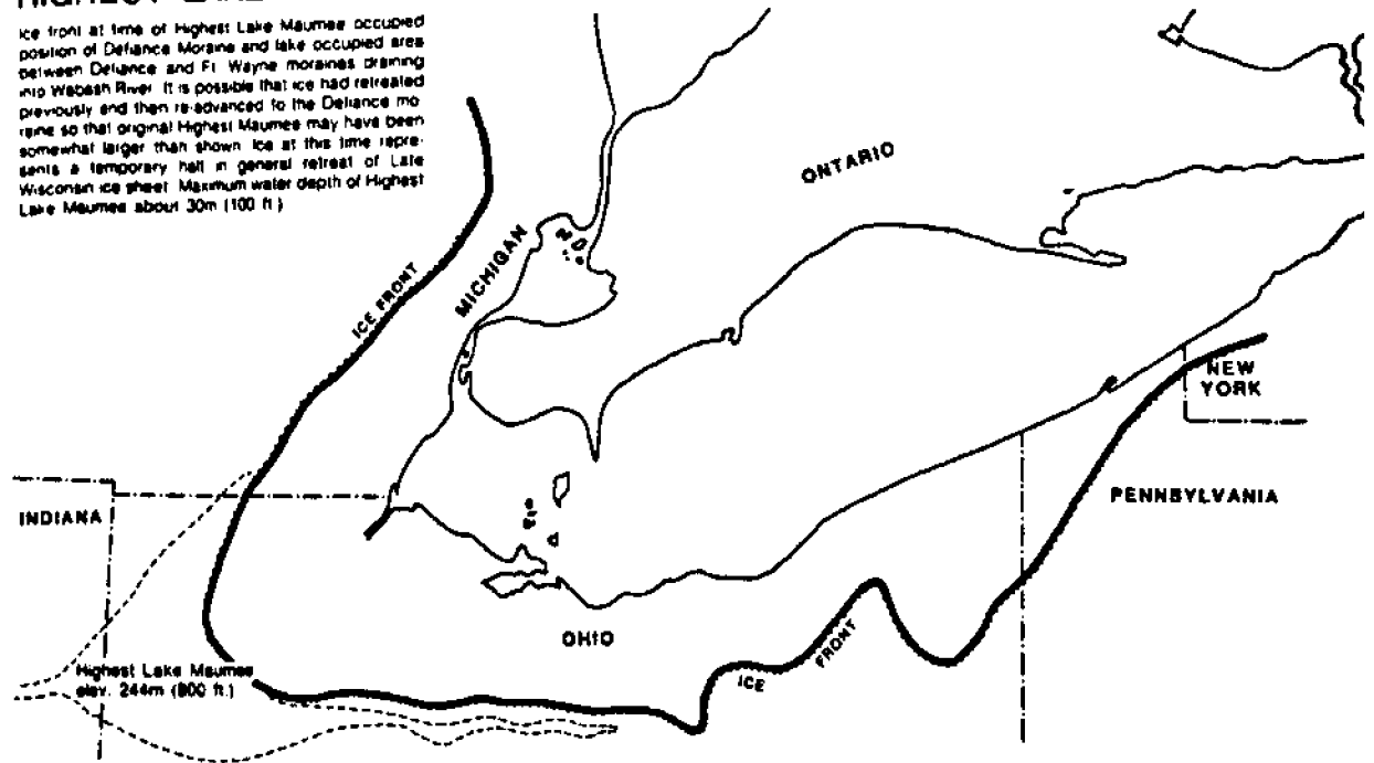
Figure 7. Highest Lake Maumee.
