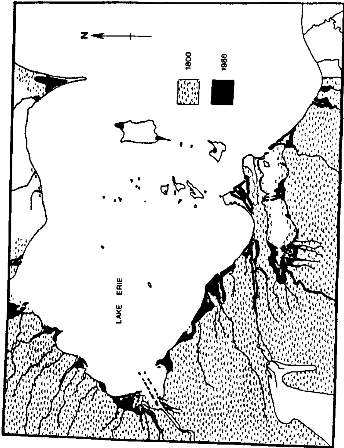
Figure 8. Loss of coastal wetlands surrounding western Lake Erie 1800-1988.
