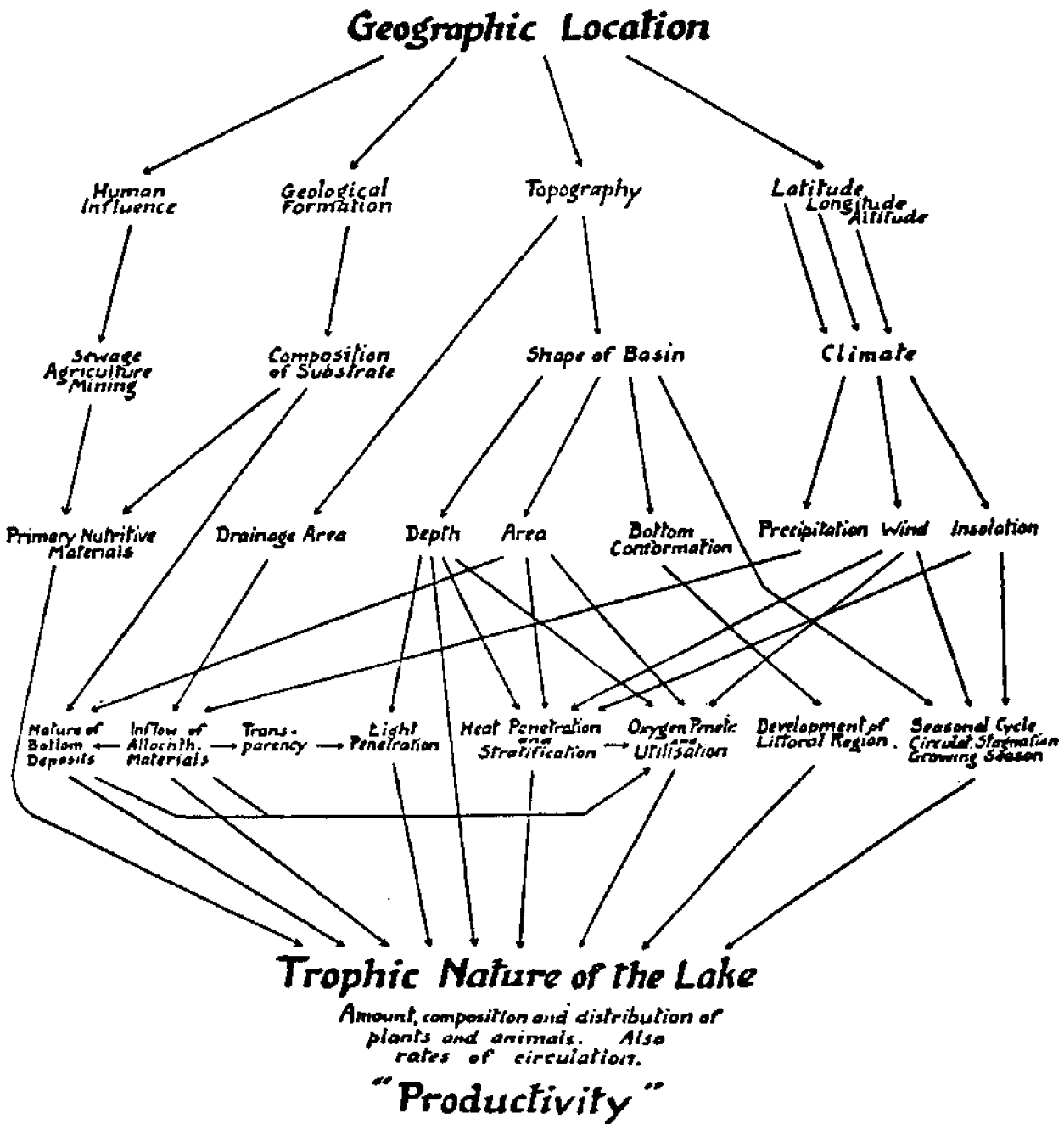
Figure 3. Factors influencing the biological productivity of a lake (after Rawson 1939)
