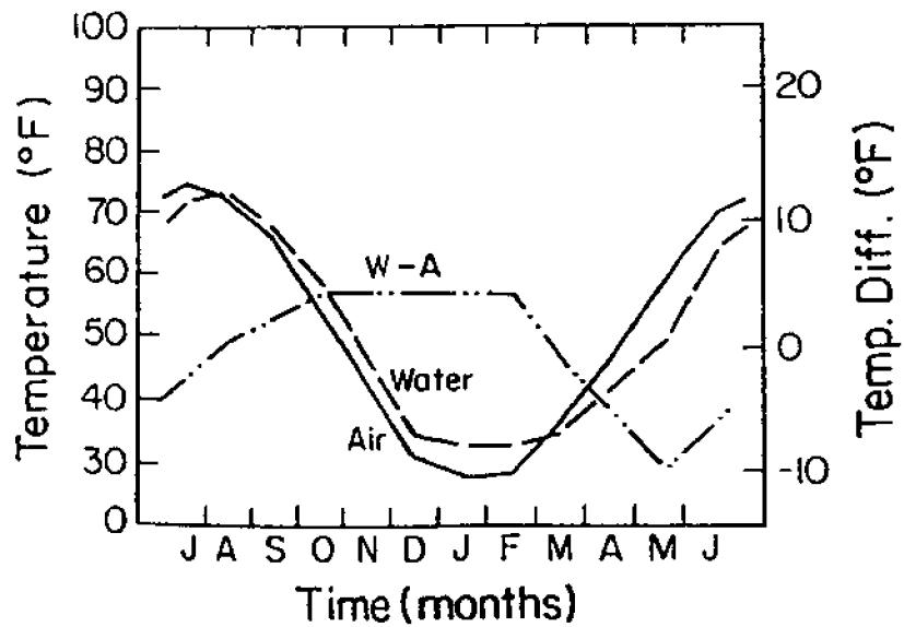
Figure 7. Monthly air and water temperatures for Lake Erie (redrawn from Hunt 1958).
