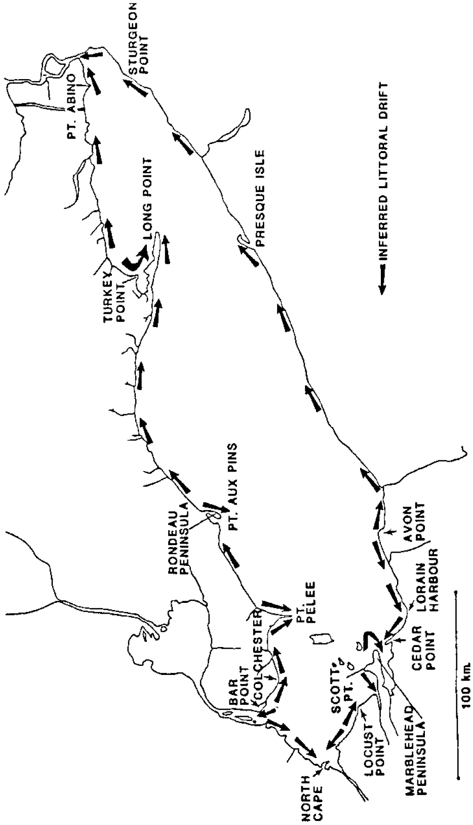
Figure 21. Dominant alongshore currents in Lake Erie.
