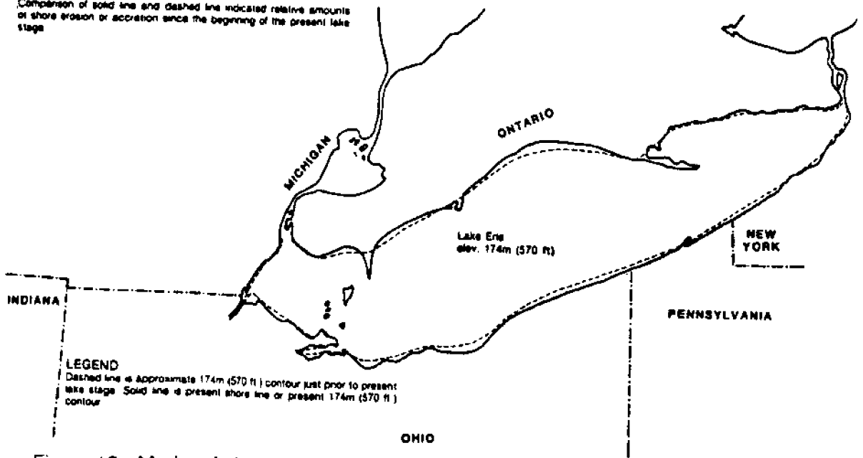
Figure 18. Modern Lake Erie.
