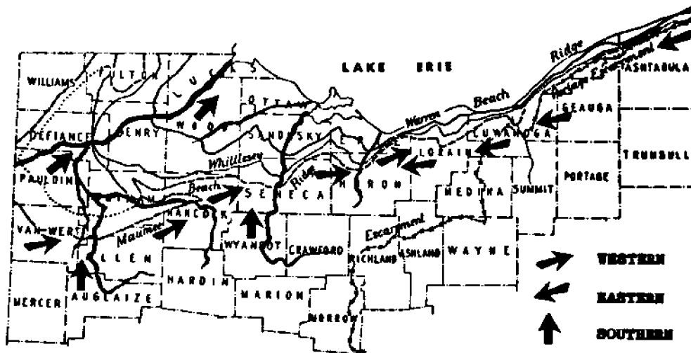
Figure 3. Map of northern Ohio showing suggestive migration routes of western, eastern, and southern species into western Lake Erie (base map from Ohio Geological Survey in Herdendorf 1987, p. 32).
