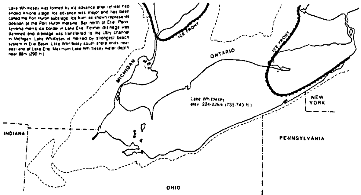
Figure 11. Lake Whittlesey.
