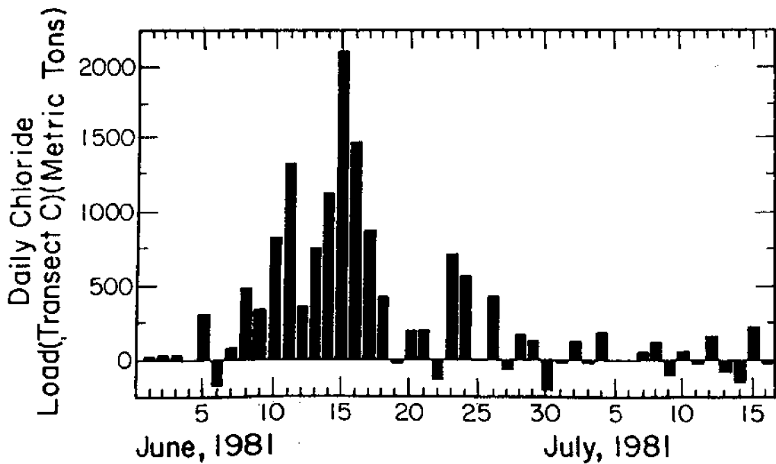
Figure 18. Daily average loads of chloride in Sandusky Bay at Transects A and C (see Fig. 14).
