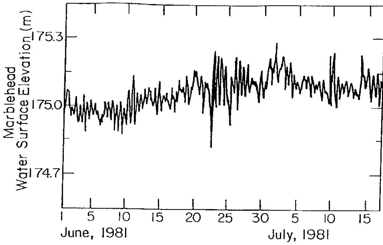
Figure 16a. Marblehead water level time series (Bedford and Mark 1988).
