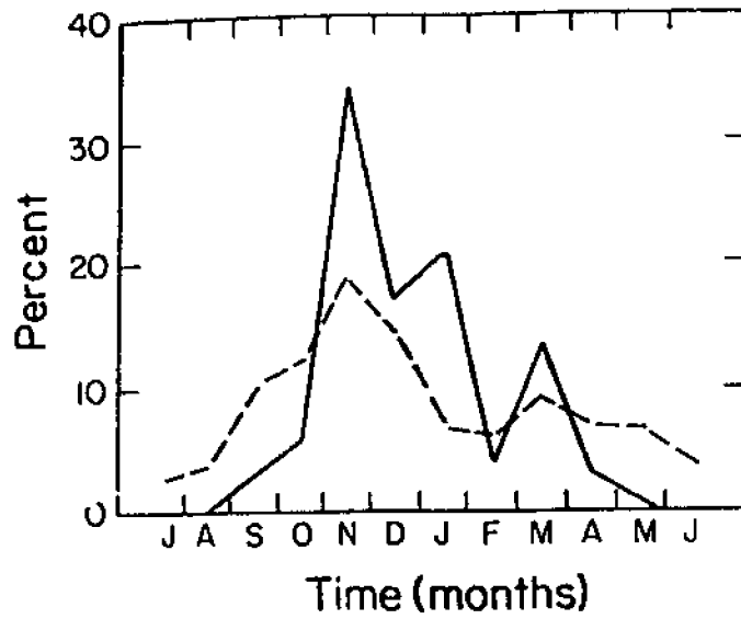
Figure 6c. Frequency distribution of six foot setups or greater (——) and severe storms (- - - -) (redrawn from Pore et al. 1975).
