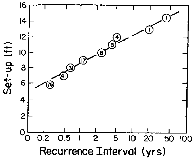
Figure 6a. Recurrence intervals for Buffalo-Toledo setups; circled numbers are number of cases for observed setup at one foot increments as of 1973 (redrawn from Pore et al. 1975).
