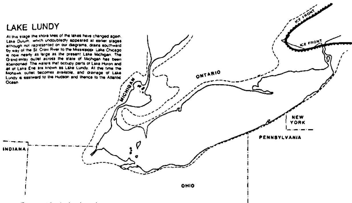
Figure 13. Lake Lundy.
