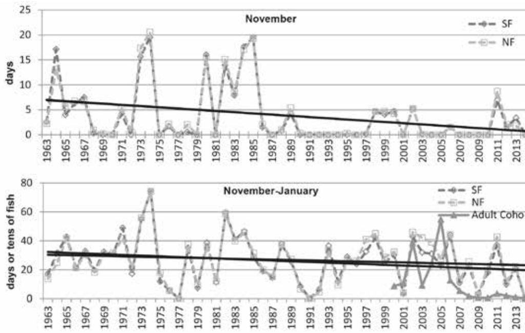
Figure 4—Duration of fish-passage flows (85 to 1331 L s -1 ) expressed as days within flow range for North Fork and South Fork and adult coho abundance estimate expressed as tens of fish. Only November trends significant ( p=0.017 SF, 0.013 NF).
