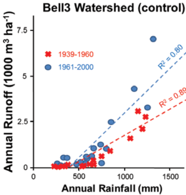
Figure 2—Rainfall-runoff relationships in Bell3 watershed during the pre- and post-type-conversion time periods of Bell1 and Bell2 watersheds. The immediate post-fire years of 1961-1964 have been omitted from this analysis.
