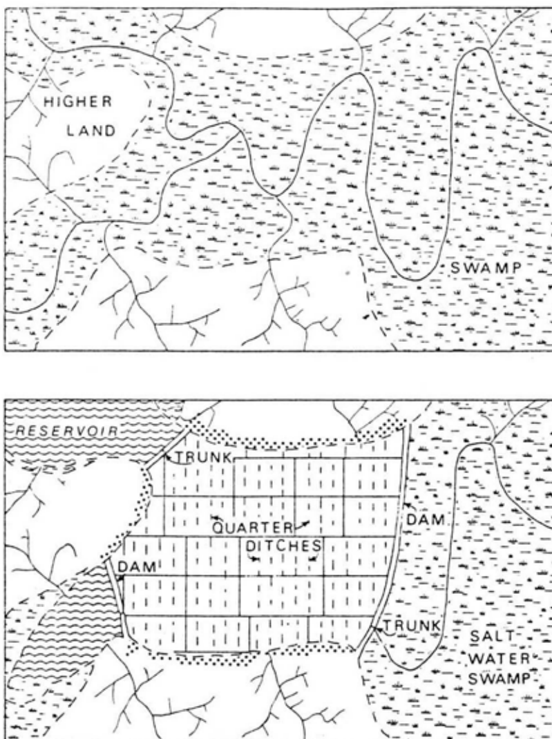
Figure 1 – Basic inland rice field
