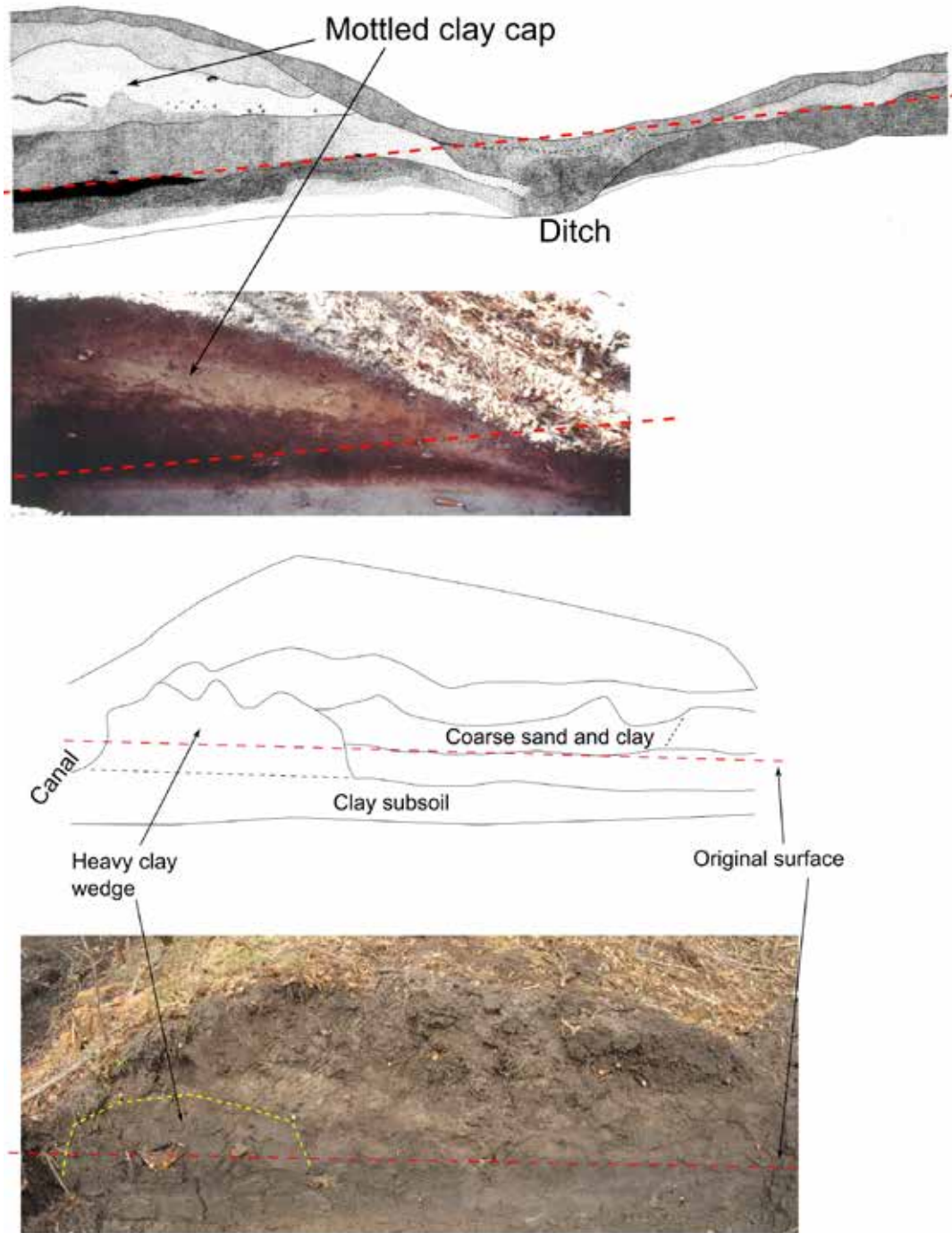
Figure 1 – Profile drawing and photo of embankment excavation at Willtown (top), profile drawing and photo of embankment at Bluehouse Swamp (bottom).
