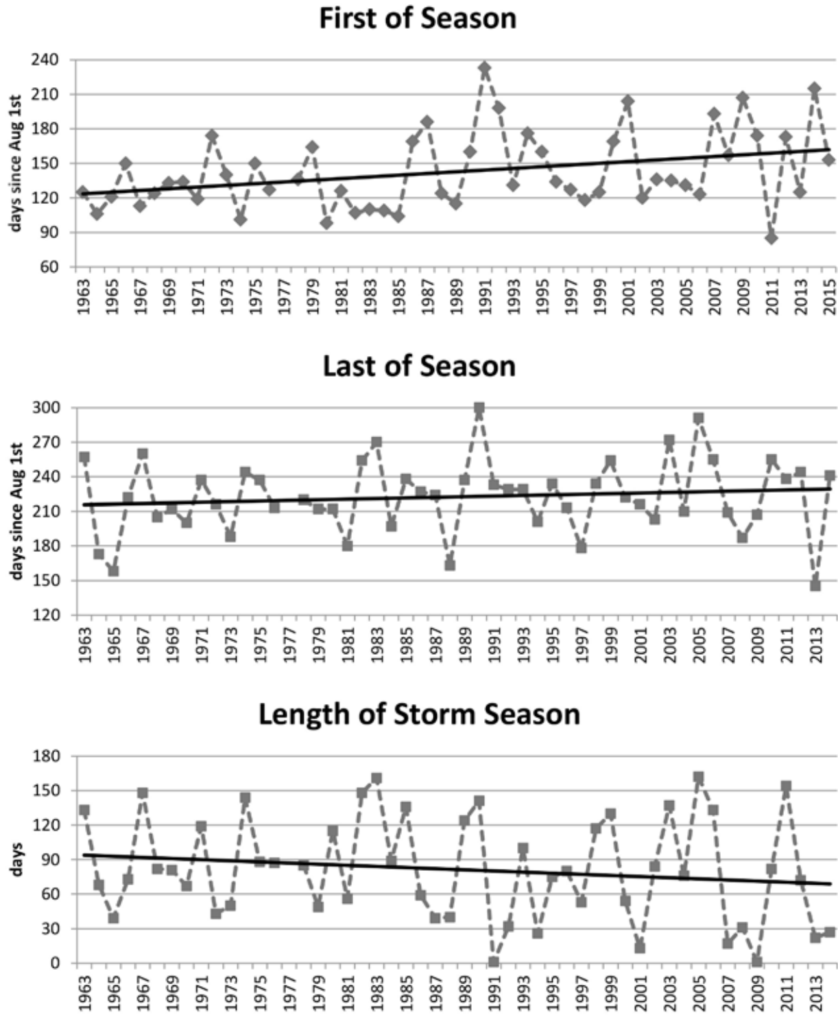
Figure 5—First fall peak flow, last spring peak flow, and length of storm season by hydrologic year. Only first-of-season trend significant ( p=0.013 ).
