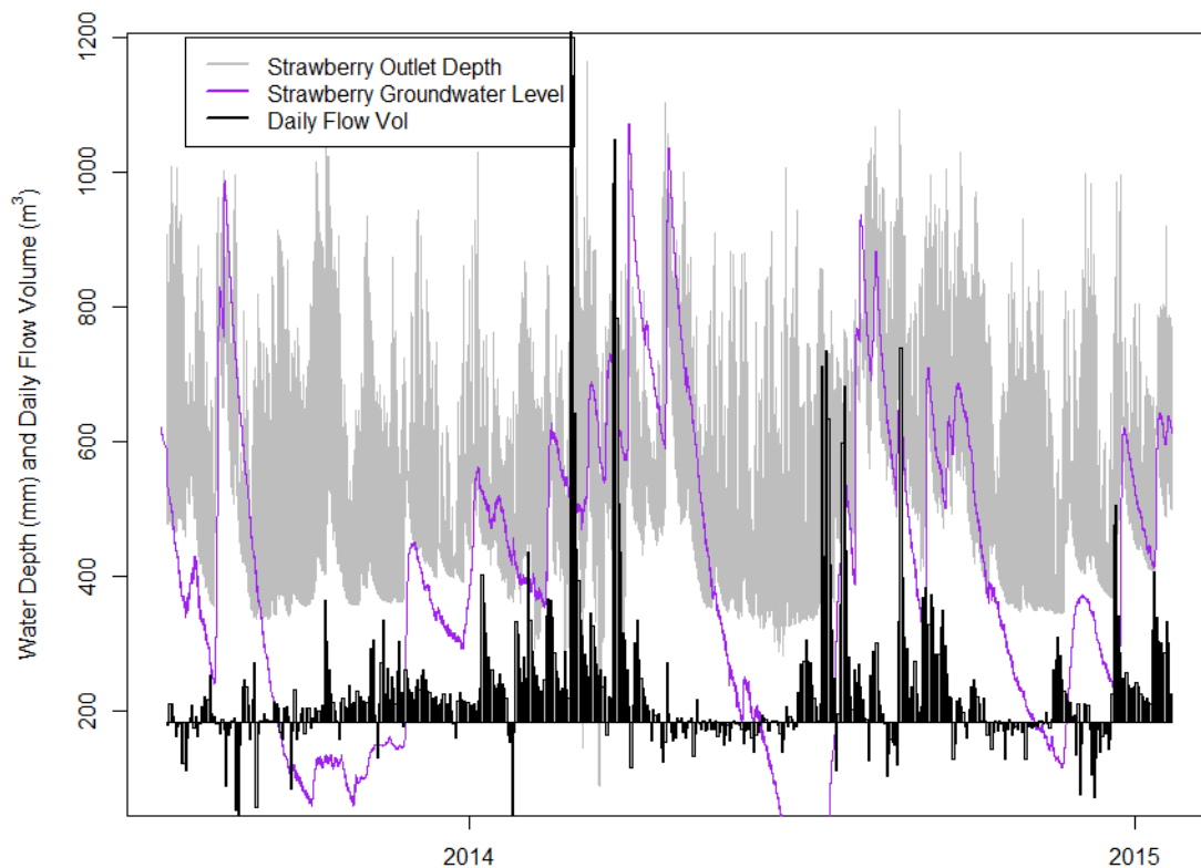
Figure 1—Net daily flow volumes measured at Strawberry Swamp outlet between June 2013 and January 2015 represented as vertical bars. Water level at the wetland outlet is depicted as a gray line and show the influence of tidal, backwater, and upland flow dynamics. Groundwater level measured at an upland location is shown with a purple line and represent water elevations above a datum that is 3.3m below the ground surface.
