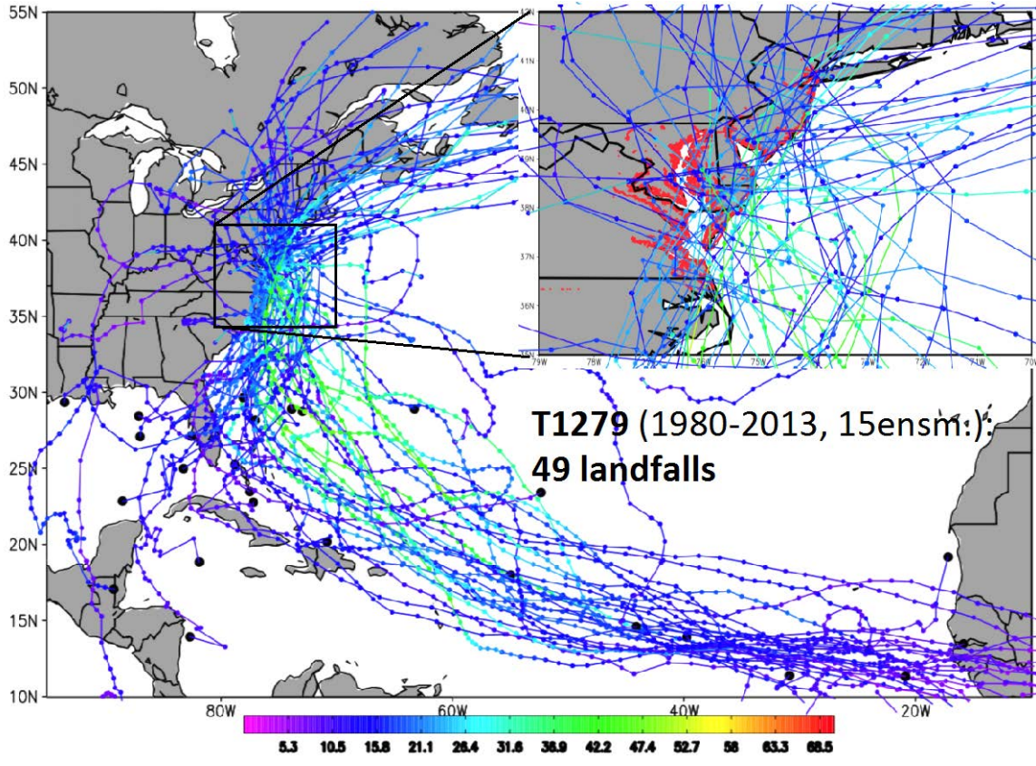
Figure S1: TC tracks (in 6-hourly segments) with landfalls in the Mid-Atlantic from Minerva hindcasts at T1279 (1980-2013; 15 ensemble members). Color along the track represents the values of the 10-min MSW (see horizontal bar; scale is m/s). Genesis locations are shown in black filled circles. Mid-Atlantic coastline is shown in red in the inset.
