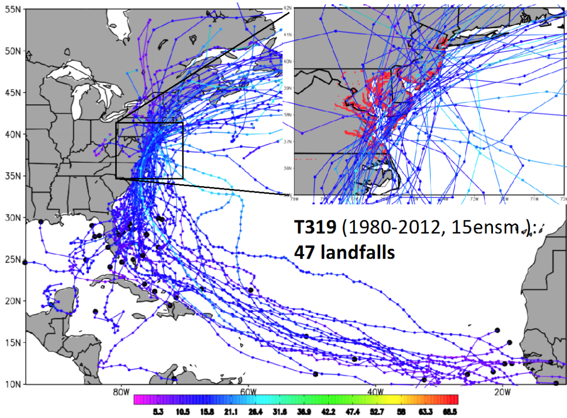
Figure S2: TC tracks (in 6-hourly segments) with landfalls in the Mid-Atlantic from Minerva hindcasts at T319 (1980-2012; 15 ensemble members). Color along the track represents the values of the 10-min MSW (see horizontal bar; scale is m/s). Genesis locations are shown in black filled circles. Mid-Atlantic coastline is shown in red in the inset.
