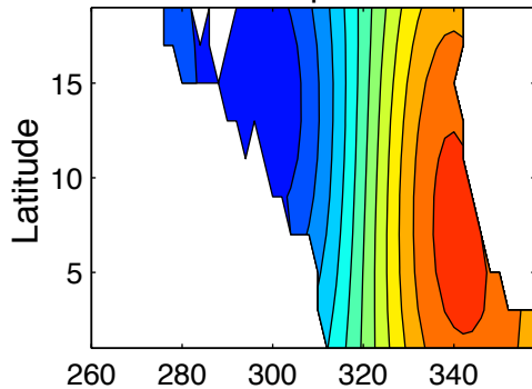
2nd Laplacian
