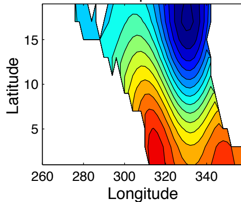
4th Laplacian
