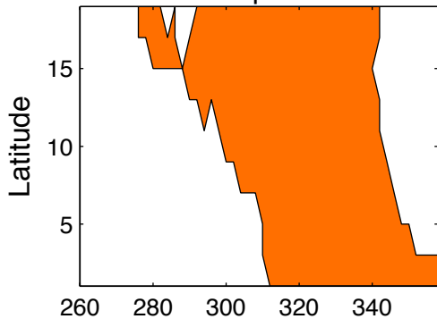
1st Laplacian
