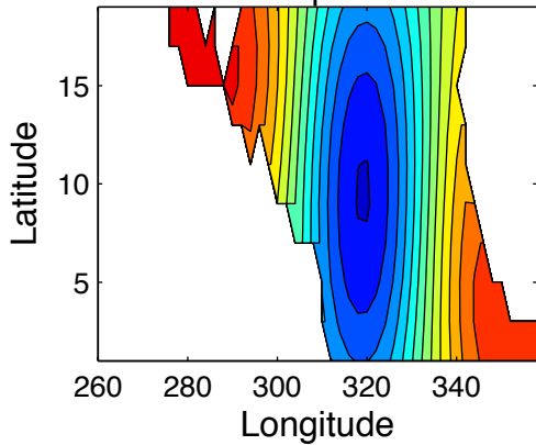
3rd Laplacian
