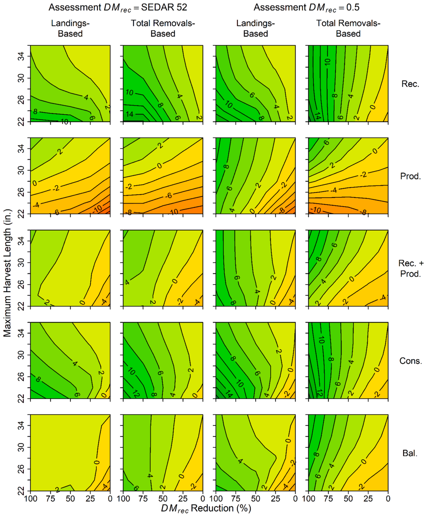
Fig. 4. Summary metric ( SM ) values (unitless) for harvest slots and reductions in recreational discard mortality rate ( DM_{rec} ) demonstrated for a variety of management priority emphasis schemes (Table 4): Recreation (Rec., row 1), Production (Prod., row 2), Recreation + Production (Rec. + Prod., row 3), Conservation (Cons., row 4), and Balanced (Bal., row 5). For each contour plot, minimum harvest length is 16 in. TL, maximum harvest length ranges from 22 to 34 in. TL and no maximum (top) on the y-axis, and relative reduction of DM_{rec} in the projection years are shown on the x-axis. The landings-based and total removals-based quota accounting approaches are contrasted for assumed assessment DM_{rec} = \text{SEDAR } 52 values (left columns) and 0.5 (right columns).
