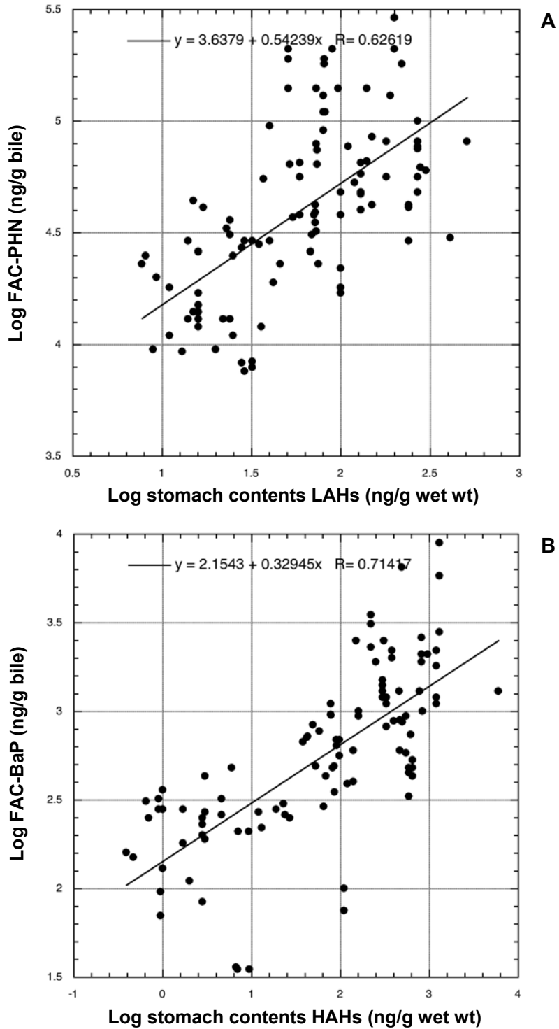
Figure 14. Relationship between (A) concentrations of \Sigma LAHs in stomach contents and fluorescent metabolites of \Sigma LAHs in bile, measured as FACs-PHN, and (B) concentrations of \Sigma HAHs in stomach contents and fluorescent metabolites of \Sigma HAHs in bile, measured as FACs-BaP, for juvenile Chinook salmon from sites within Kitimat Arm (Alcan Inner Harbour, Hospital Beach, Inner Eurocan Beach, Outer Eurocan Beach, Minette Bay, and Wathlsto Creek) and from reference sites outside Kitimat Arm (Kemano Village and Kildala Arm).
