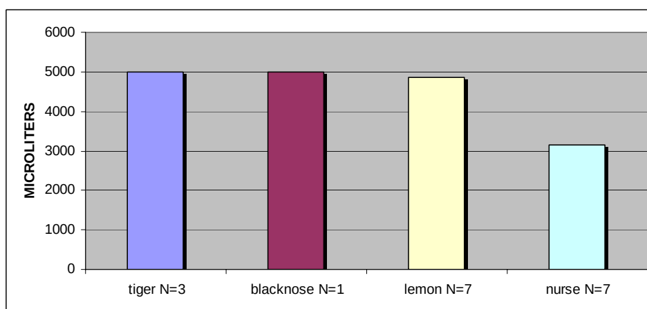
Figure 3.--Average volume of ( E )-2 butenoic acid in microliters required to terminate tonic immobility in various shark species using a dose released at least 15 cm from the nares.
