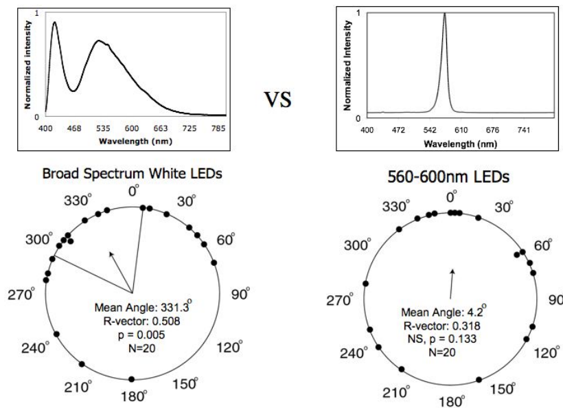
Figure 4.--Juvenile loggerhead turtles were attracted to all activated lights, but appear to be less attracted to LEDs that produce light in the 560-600 nm range than they are to other sources of illumination.
