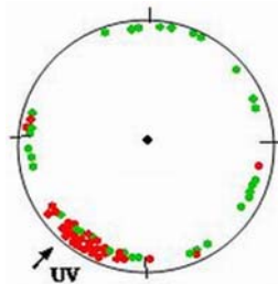
Figure 5.--Turtles' behavioral responses to UV light.
