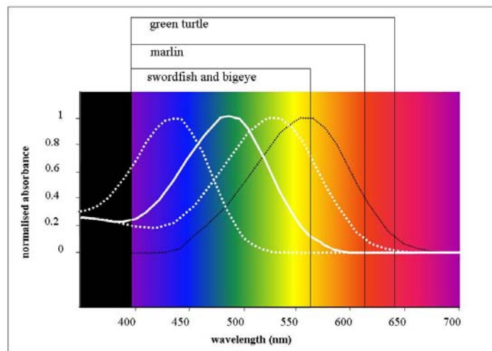
Figure 1.--Hypothesized spectral sensitivities of marine fishes and turtles.
