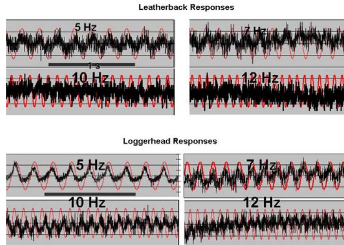
Figure 1.--Tracking capabilities of leatherback and loggerhead retinas to varying speeds of individual light pulses. These electroretinograms are from retinal cup preparations without the vitreous, lens, and cornea. Oscillating red line shows the flash rate. The light is on at maximum intensity at the top of each cycle, and off at the bottom of each cycle. Retina responses are shown by the black line.
