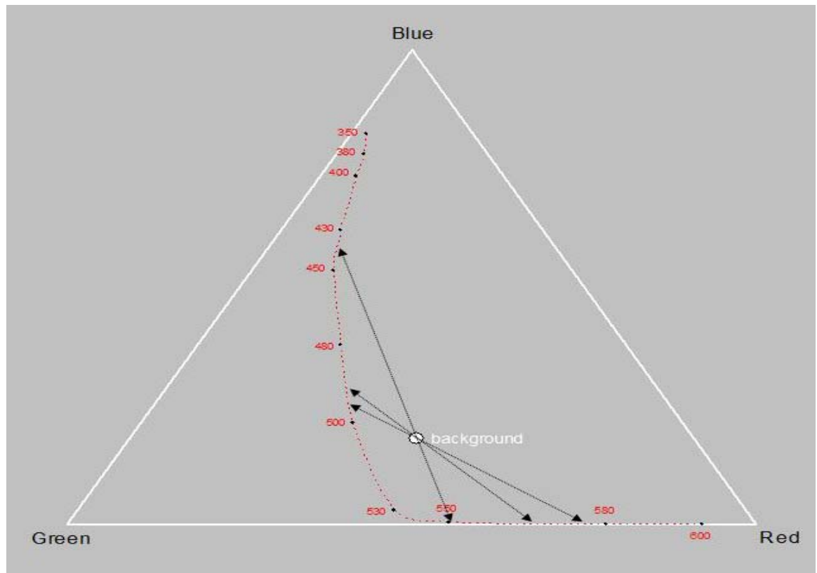
Figure 2.--LEDs can be modified to match background ocean color. Different wavelength distributions which have the same chromaticity and color response are called metamers . For example, a yellow formed by monochromatic light at 580 nm looks the same as a roughly equal mixture of 560 nm and 610 nm light; these are metamers of each other. Different chromaticities that lie across gray from each other are called complementaries . Additions of any two chromaticities lie on the line between them; additions of any three chromaticities lie in the triangle between them.
