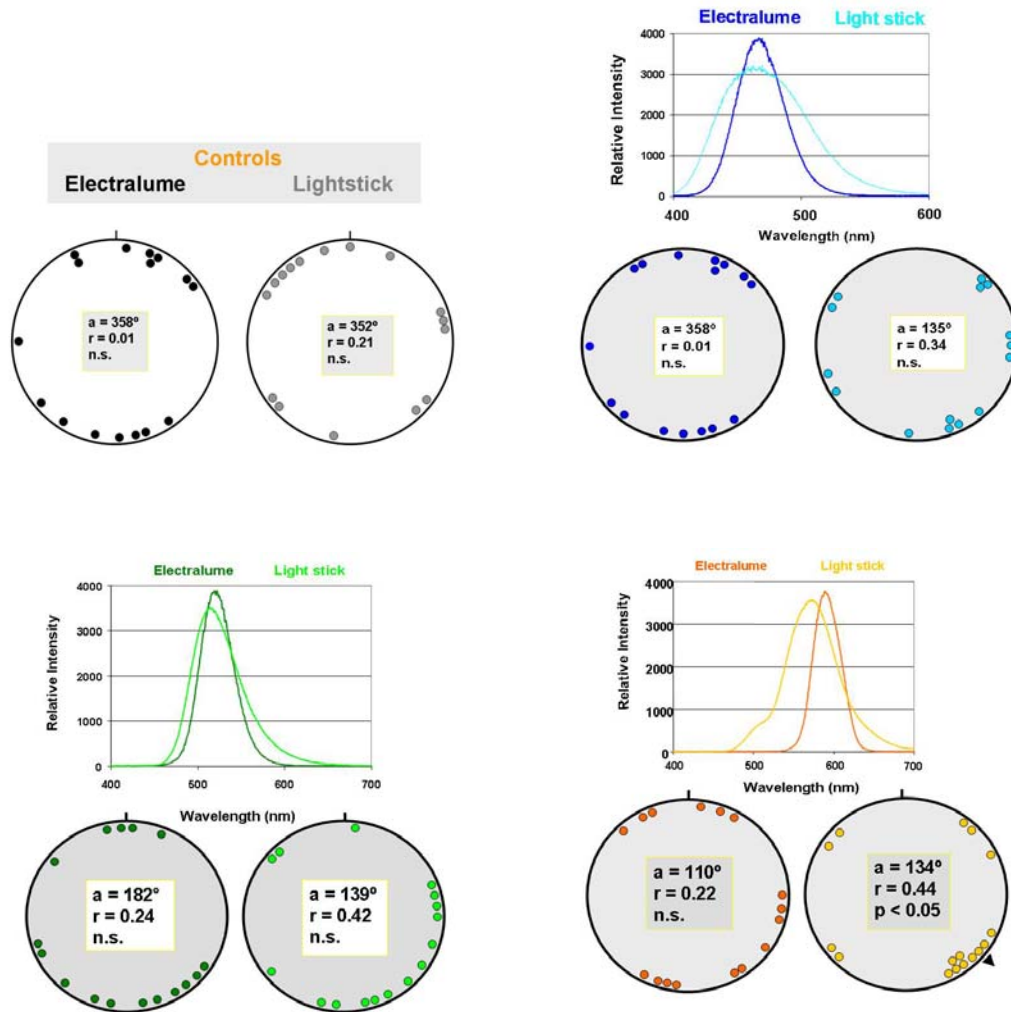
Figure 3.--Orientation of captive-reared leatherbacks to lightsticks and electralumes under three experiments (light spectra) and control conditions (no light). In each diagram, upper graph shows spectrum of light transmitted by the light source (except in the top left pair of the diagram's figure, where there was no light because this was a control). The circle diagrams show orientation; each point is a turtle's heading. The 12 o'clock mark is the position of the light (off, in this case).
