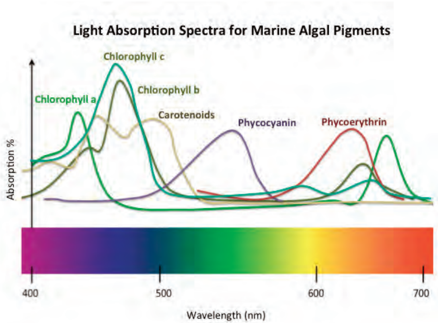
Figure 2.6. Light absorption spectra for photosynthetic pigments
