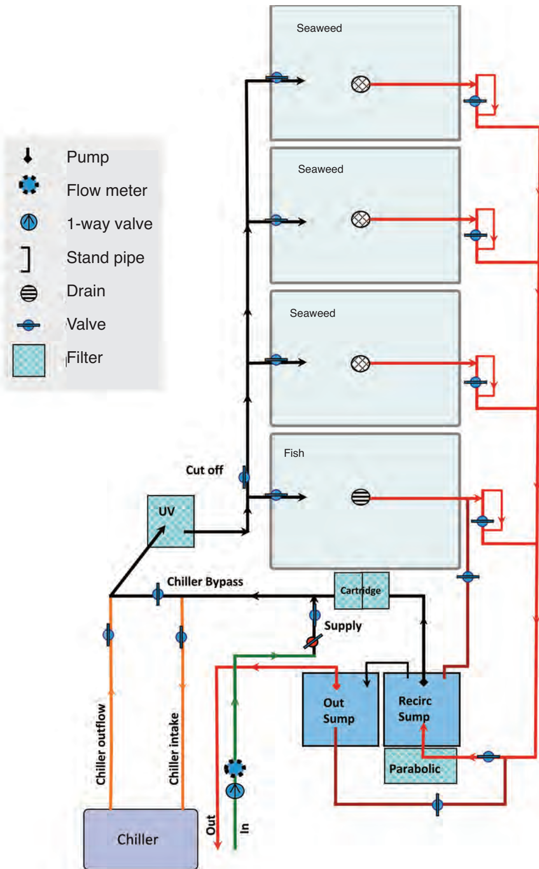
Figure 6.14. Schematic of experimental recirculating integrated multi-trophic aquaculture system containing cod and nori. The tank closest to the filters contained the fish while the three other tanks contained seaweed (Courtesy of Day, 2008).
