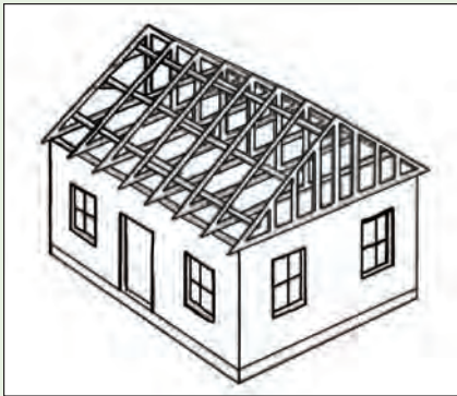
Figure 4-2. Trusses are built with a peak at the ridgeline of the house. The trusses at the end of the house form an A-shaped pattern known as a gable end. During a hurricane, the gable end is subject to great forces from the wind and could tip over, collapsing the other trusses in a domino fashion. Source: FEMA's Against the Wind brochure 247
