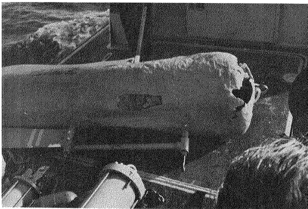
Figure 11. Polyurethane buoy: ice and pressure damage.
