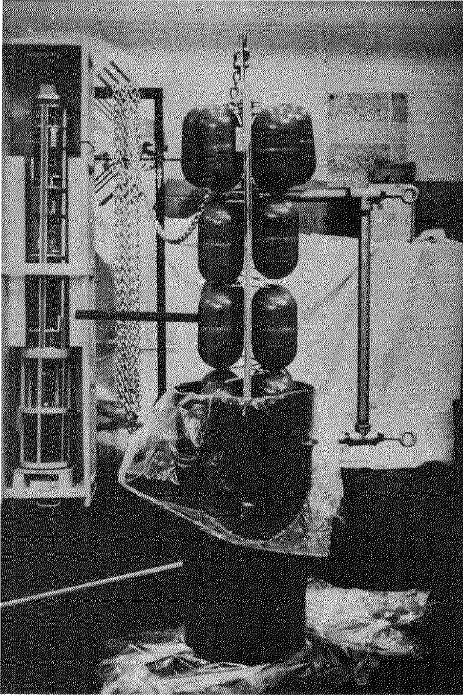
Figure 2. Polyurethane buoy: foaming process.
