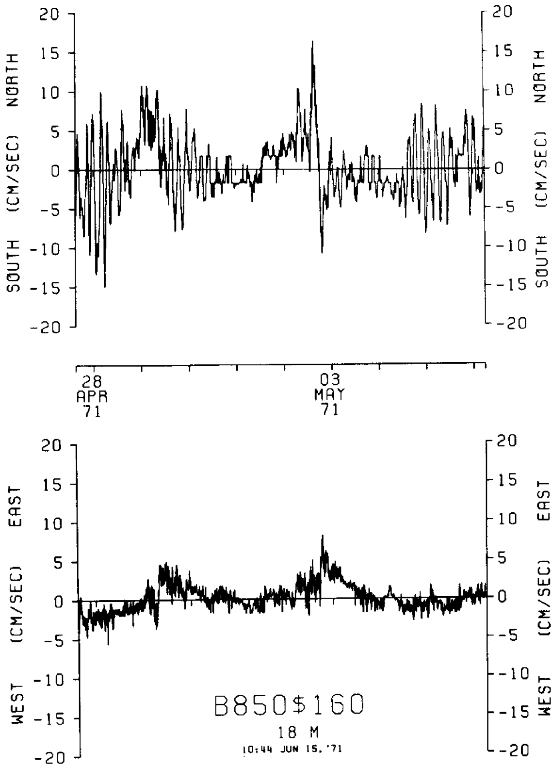
Figure 22. North-east velocity component diagram: Mooring B.
