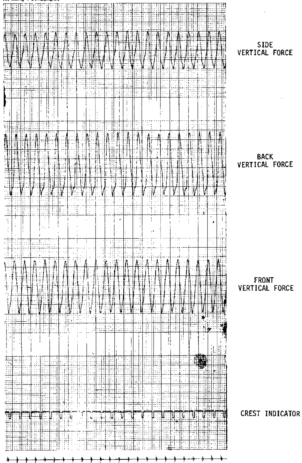
FIG. 10.-RECORDER OUTPUT FOR VERTICAL FORCES AND WAVE CREST INDICATOR
