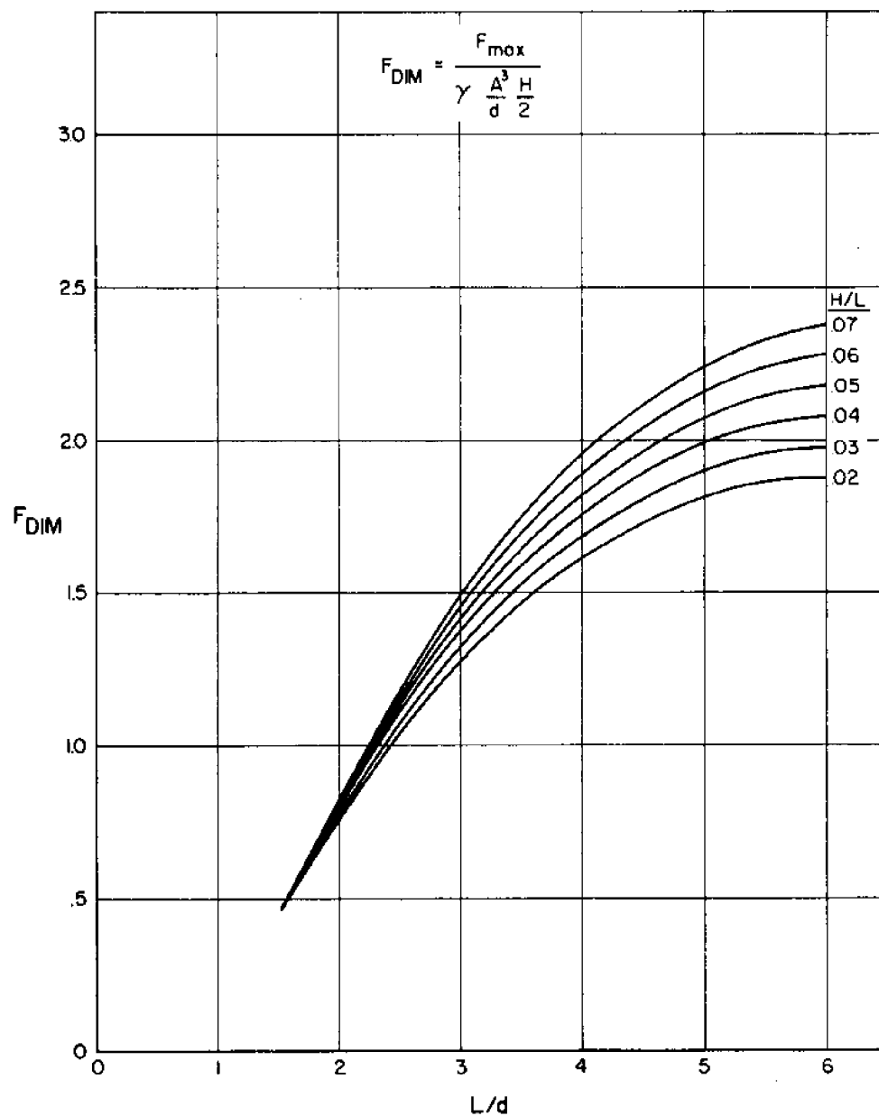
FIG. 16 — DIMENSIONLESS HORIZONTAL FORCE (COMPUTED AS A FLAT PLATE) FOR 2 INCH RECTANGULAR MODEL
