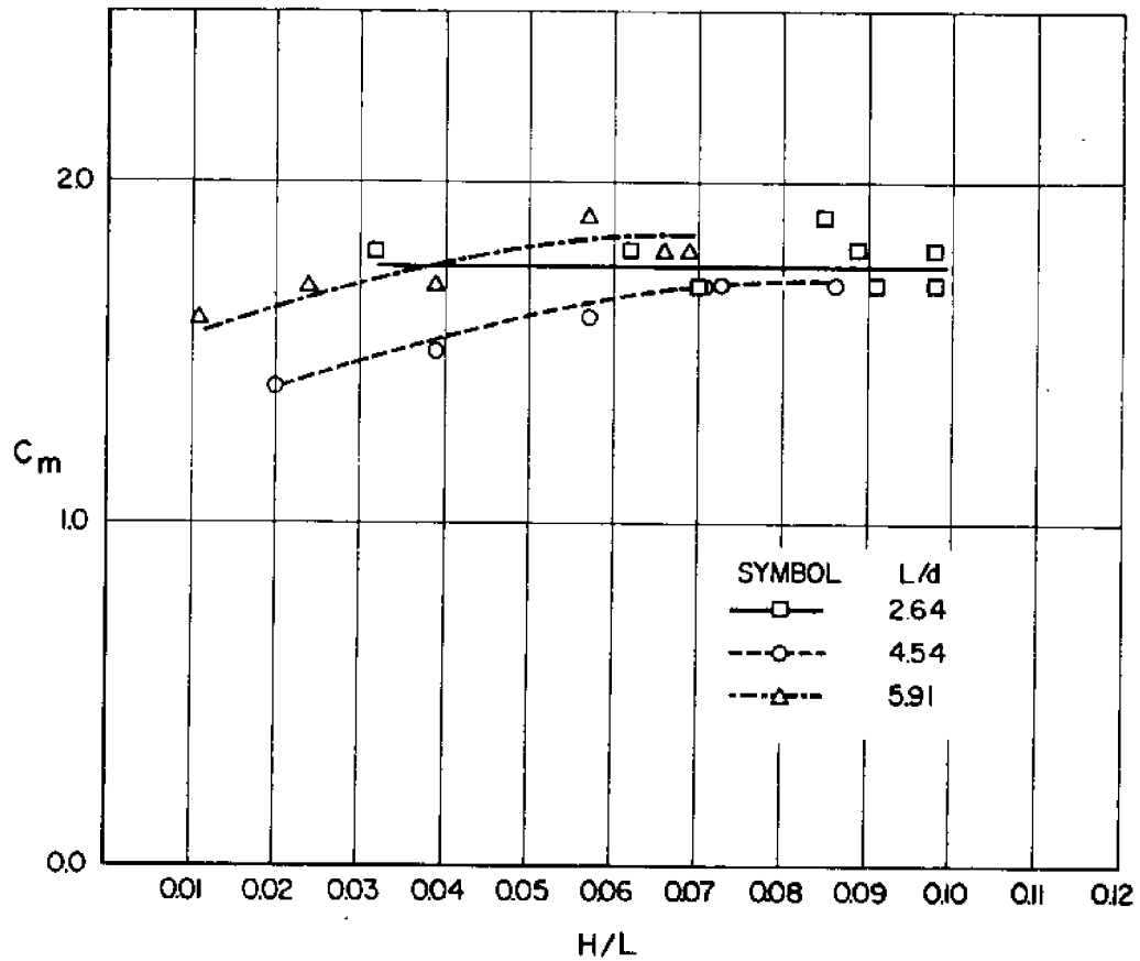
FIG. 29— COEFFICIENT OF INERTIA FOR RECTANGULAR MODEL 4 - INCHES LONG (WATER DEPTH 13 INCHES)
