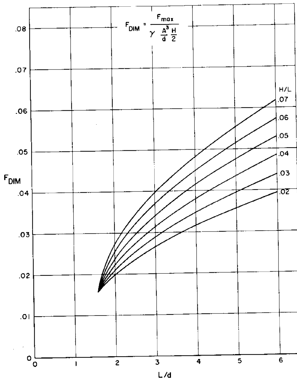
FIG. 15—DIMENSIONLESS VERTICAL FORCE (COMPUTED AS A RECTANGULAR MODEL) FOR 2 INCH RECTANGULAR MODEL
