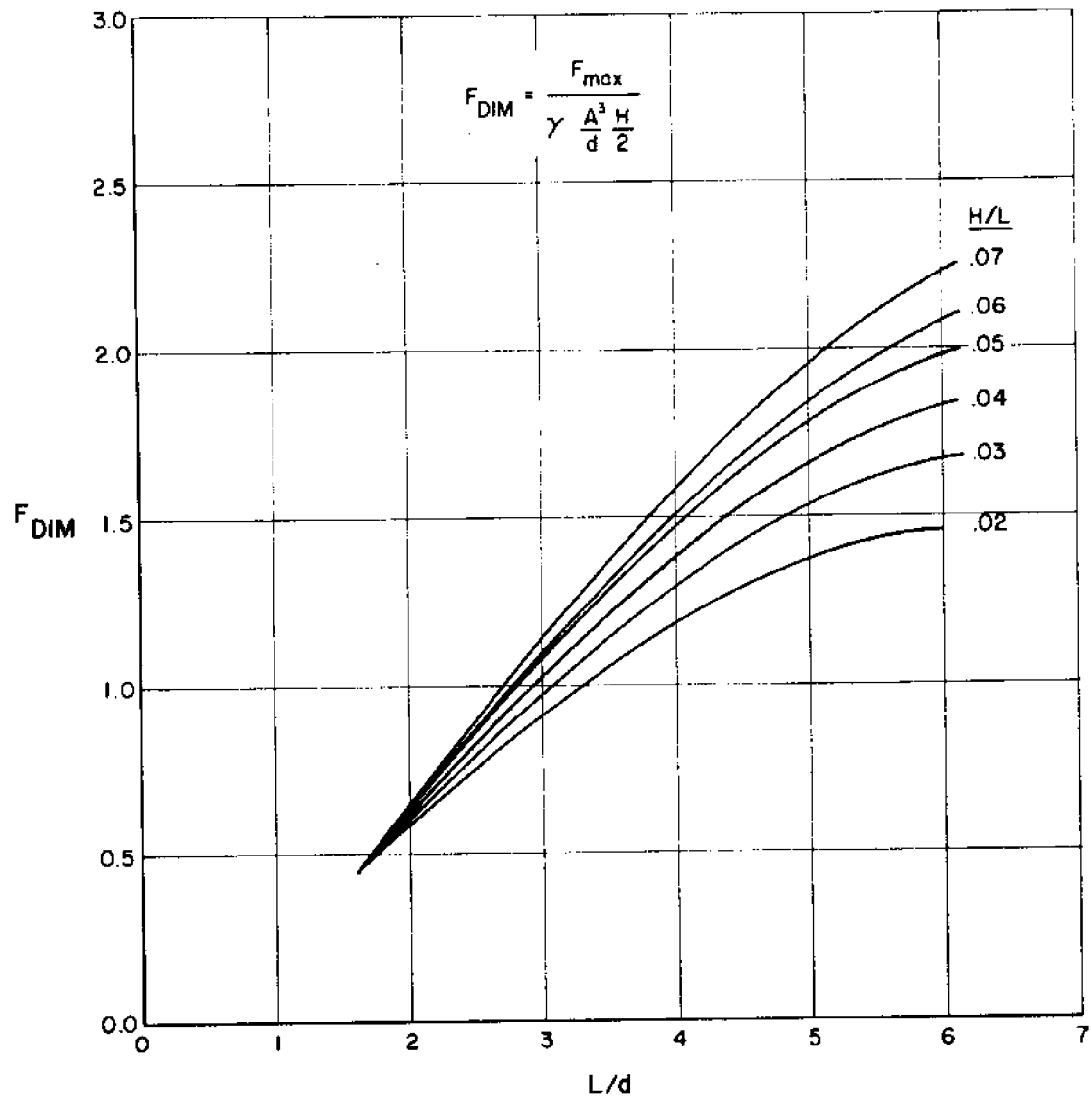
FIG. 13—DIMENSIONLESS HORIZONTAL FORCE PLOT FOR FLAT PLATE.
