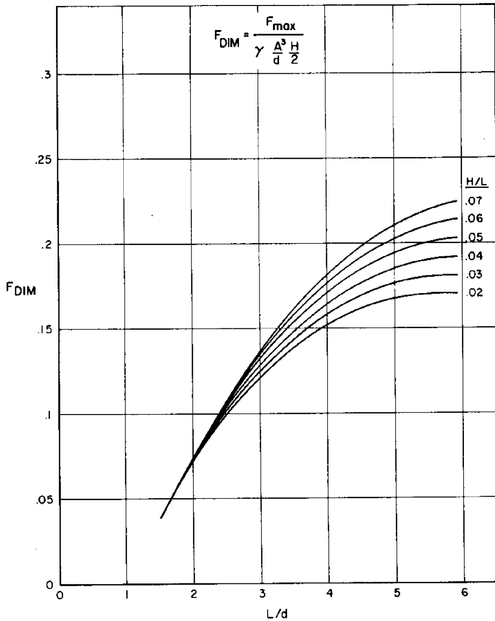
FIG. 14—DIMENSIONLESS HORIZONTAL FORCE (COMPUTED AS A RECTANGULAR MODEL) FOR 2 INCH RECTANGULAR MODEL
