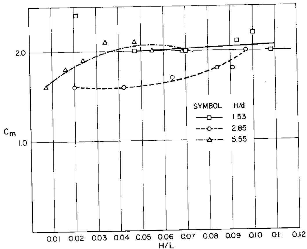
FIG. 37—COEFFICIENT OF INERTIA FOR HALF CYLINDER MODEL (END FACING INCIDENT WAVE, WATER DEPTH 24 INCHES)
