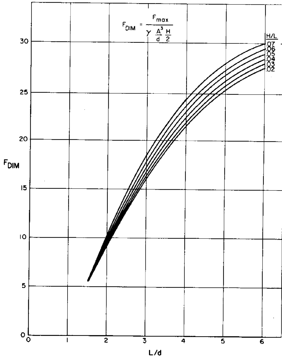
FIG.24-DIMENSIONLESS HORIZONTAL FORCE PLOT FOR HALF CYLINDER MODEL (SIDE FACING INCIDENT WAVE)
