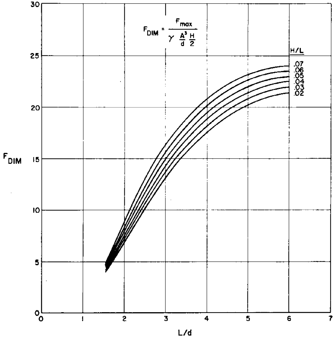
FIG. 20-DIMENSIONLESS HORIZONTAL FORCE FOR 8 INCH RECTANGULAR MODEL
