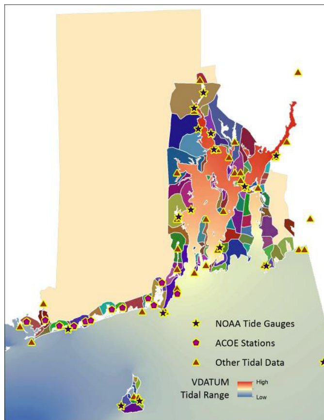
Figure 4. Map showing sub-sites and tidal stations for the RI SLAMM project
