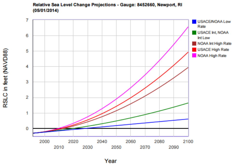
Figure 3. Projected sea level rise curves for Newport, RI
