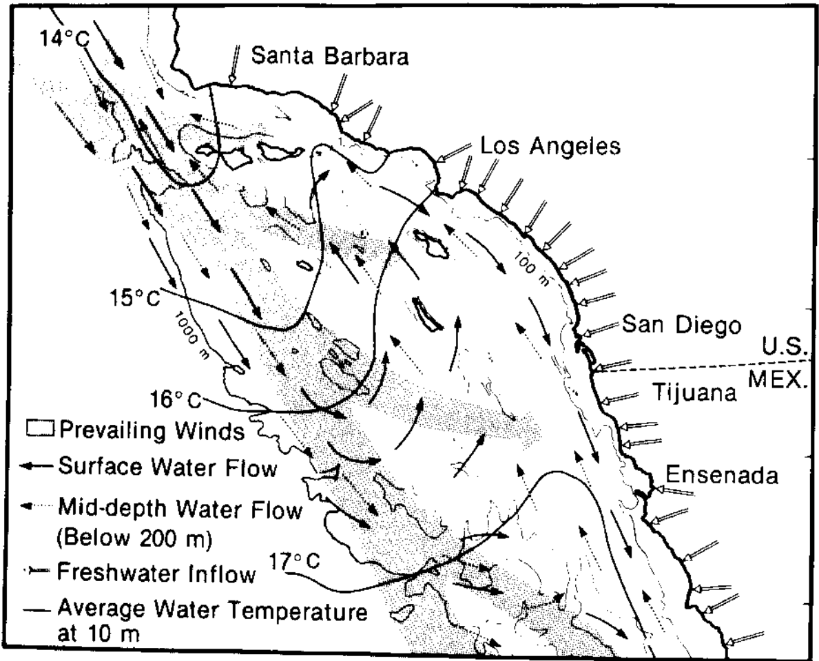
Figure 4. Nearshore patterns of bathymetry, wind, and ocean circulation (redrawn from Resources Partnership 1979).
