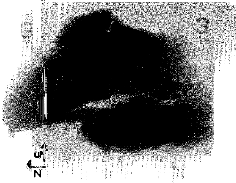
Figure 19 - Radiograph of 12.4 m deep sample, taken April 6, 1972. Original orientation marked.
