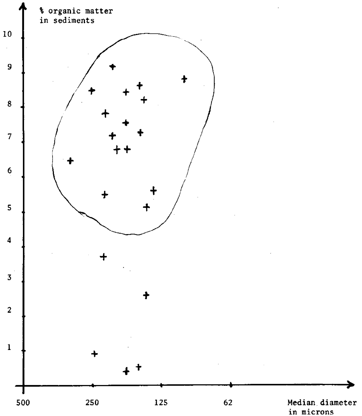
Figure 3. Comparison of grain-size and organic content for dredge spoil sediments.
