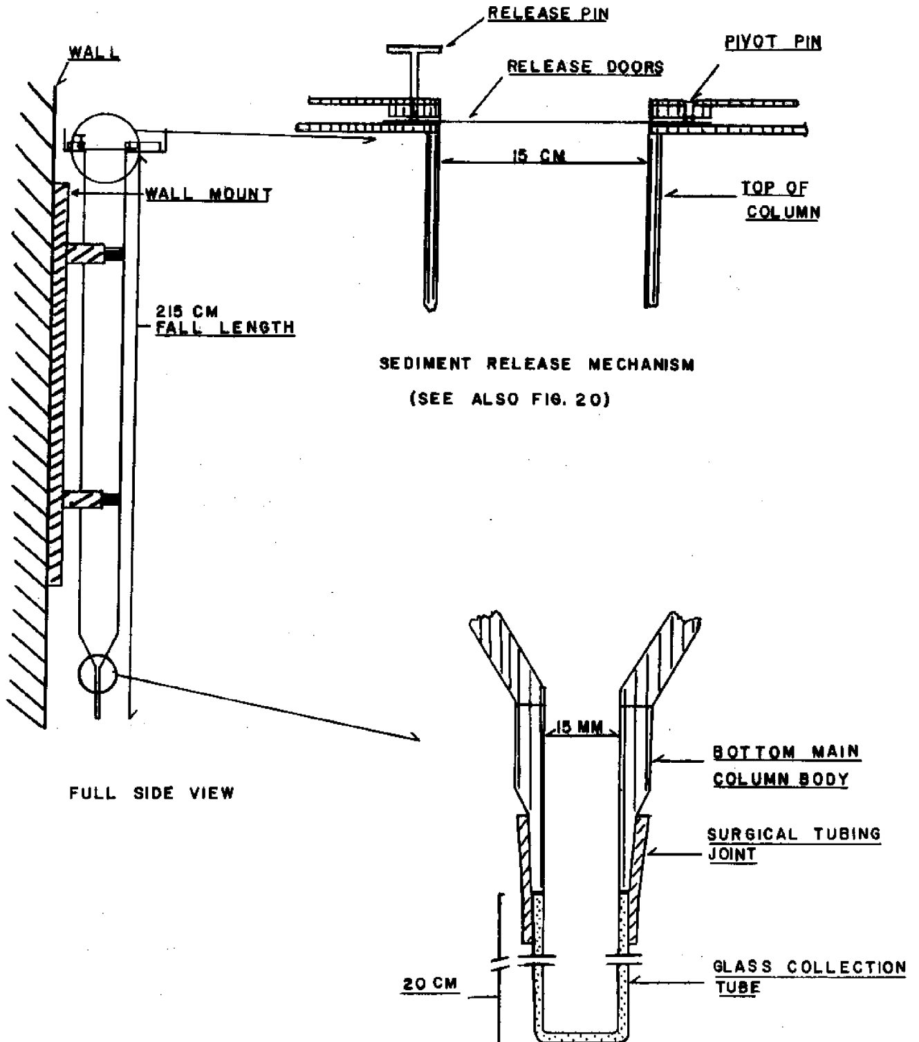
Figure 21 - Details of large settling tube used for hydraulic size analysis.
