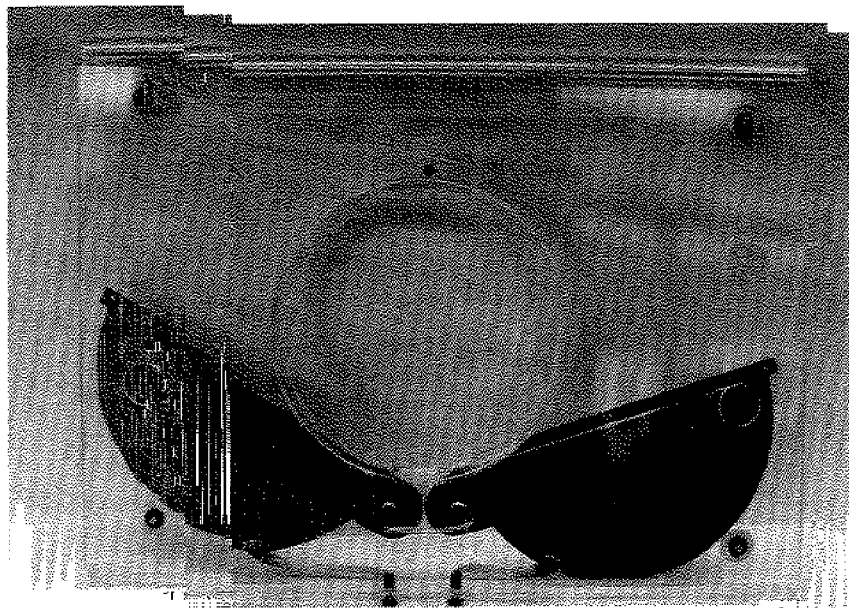
Figure 20 - Introduction doors of large settling tube, doors in open, uncocked position.
