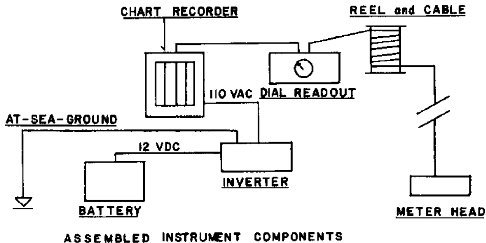
Figure 23 - Submersible current meter system shown as oriented and assembled.
