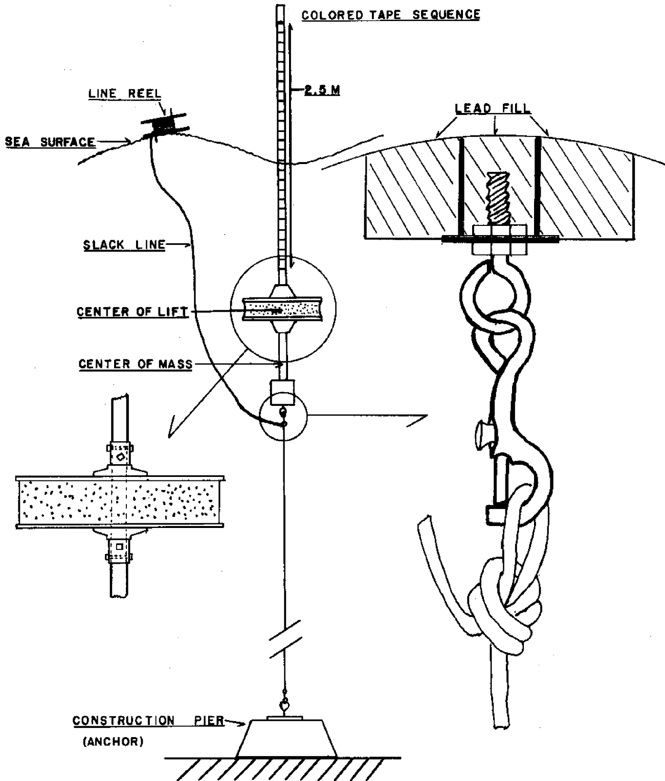
Figure 22 - Mobile wave staff system.
