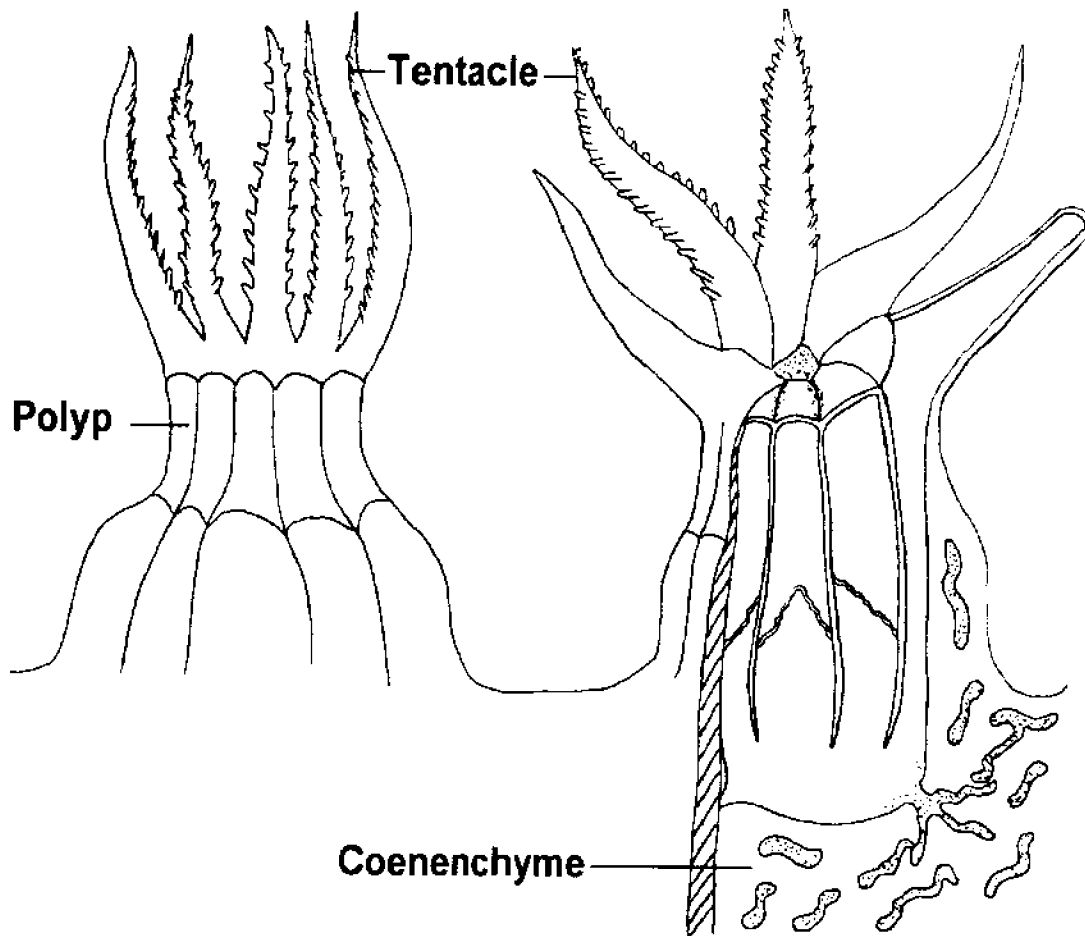
Figure 1. Schematic diagram of a soft coral polyp. (Adapted from Barnes, 1980)
