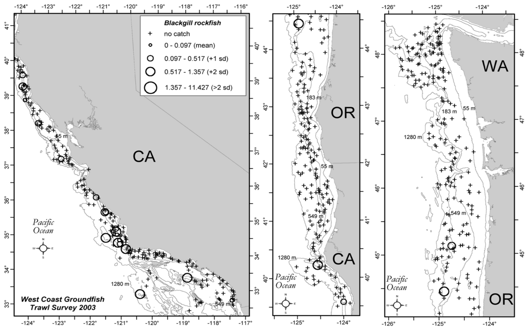
Figure 8. Blackgill rockfish distribution and relative abundance (kg/ha) from the 2003 West Coast groundfish trawl survey.
