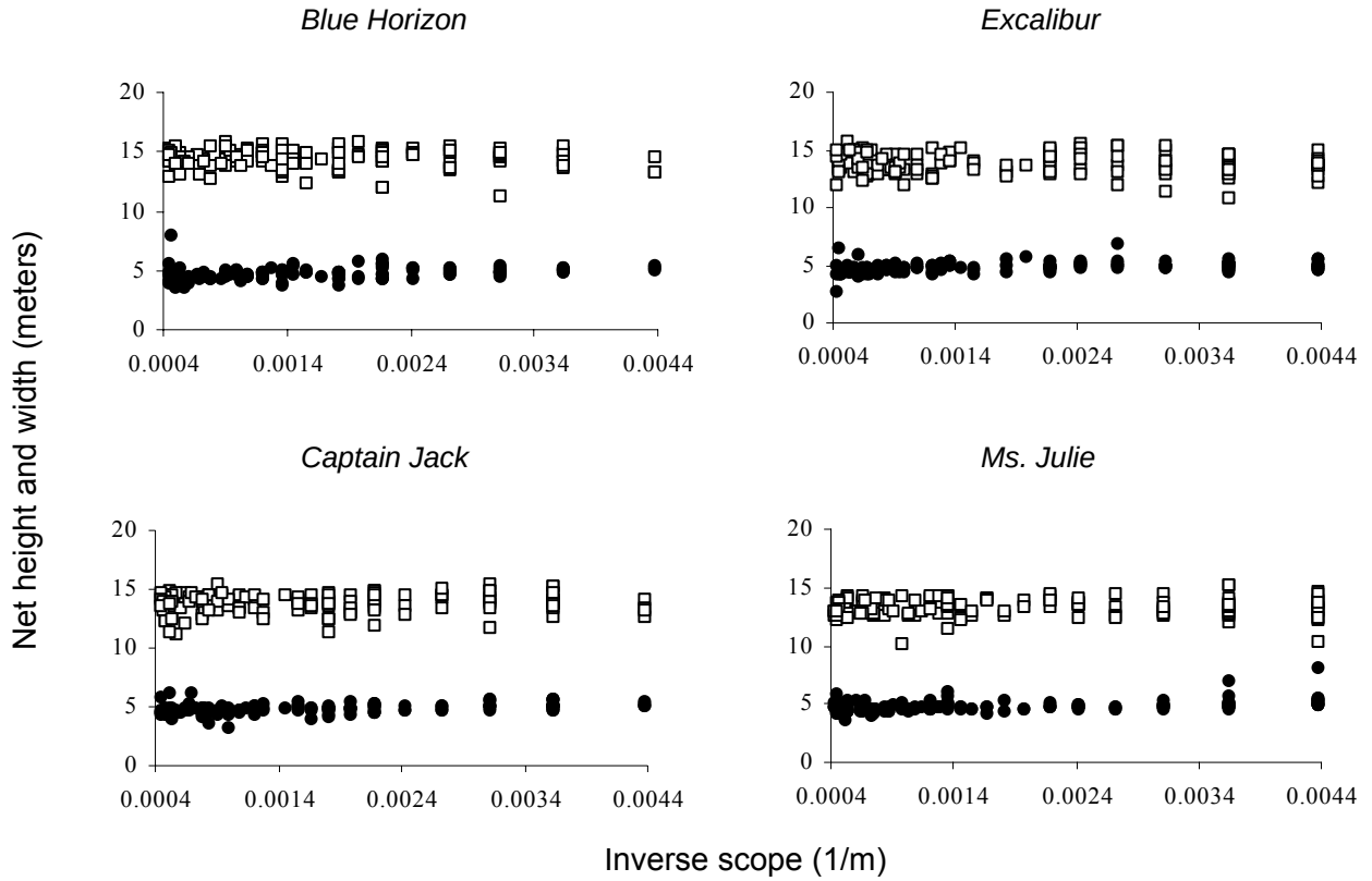
Figure 4. Mean net width (m) and height (m) for trawls conducted as part of the 2003 West Coast groundfish trawl survey. Estimates are grouped by vessel with net width ( \square ) and net height ( \bullet ) in meters plotted relative to inverse scope (1/meters). Multiple linear regressions of width versus net height and inverse scope (factored by vessel) were used to estimate net widths for tows lacking direct width observations. (FV Blue Horizon : Net width = 19.68 - 1.019 \times \text{net height} - 308.1 \times \text{inverse scope} ; FV Excalibur : Net width = 19.62 - 1.098 \times \text{net height} - 324.0 \times \text{inverse scope} ; FV Captain Jack : Net width = 18.24 - 0.781 \times \text{net height} - 335.5 \times \text{inverse scope} ; FV Ms. Julie : Net width = 17.30 - 0.727 \times \text{net height} - 274.1 \times \text{inverse scope} ).
