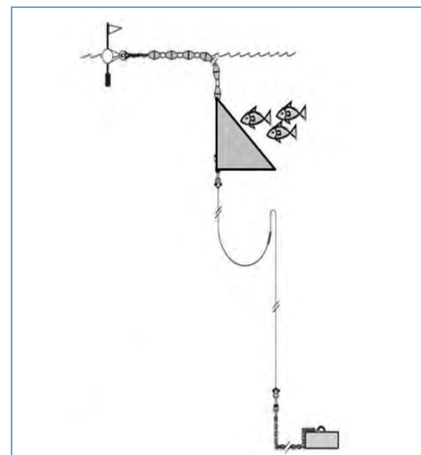
Figure 1. Fish Aggregating Device (FAD)
