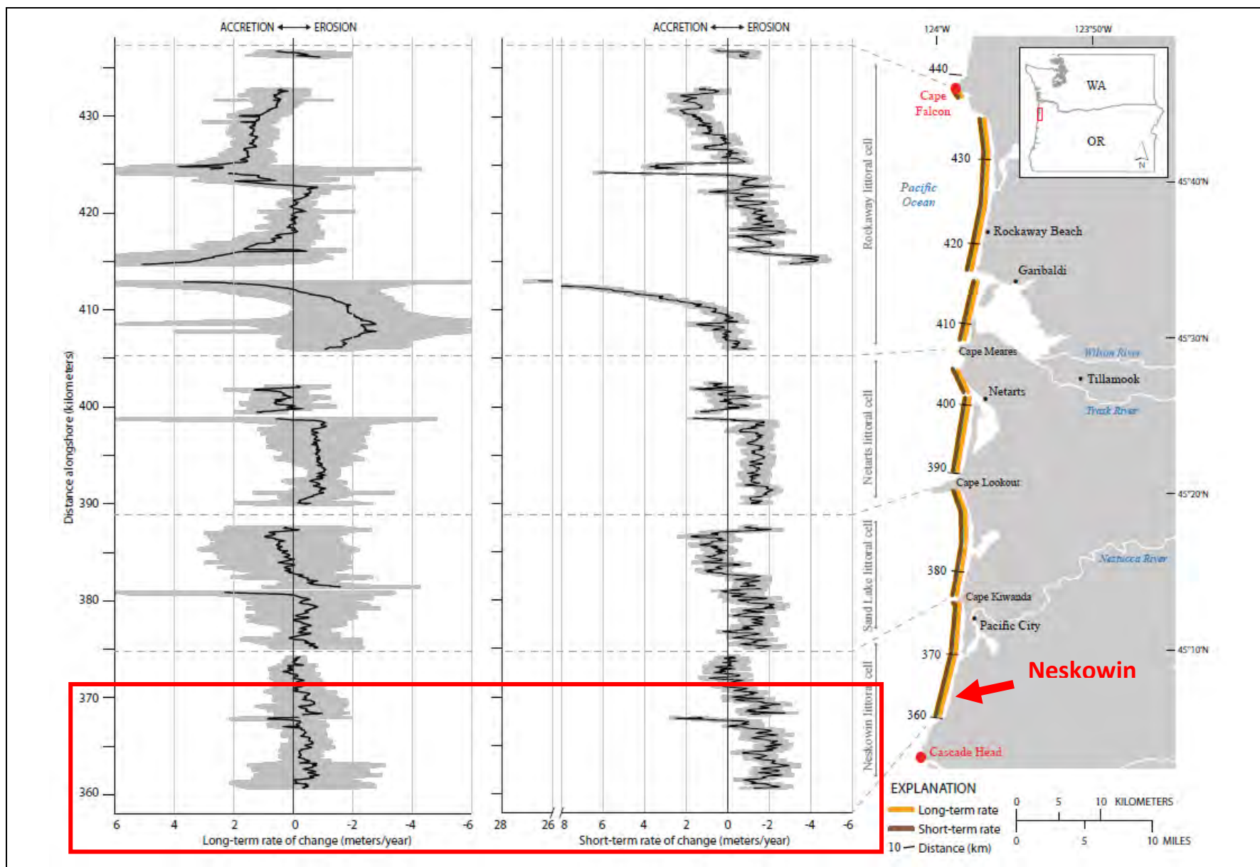
Figure 3 Shoreline Erosion Rates
