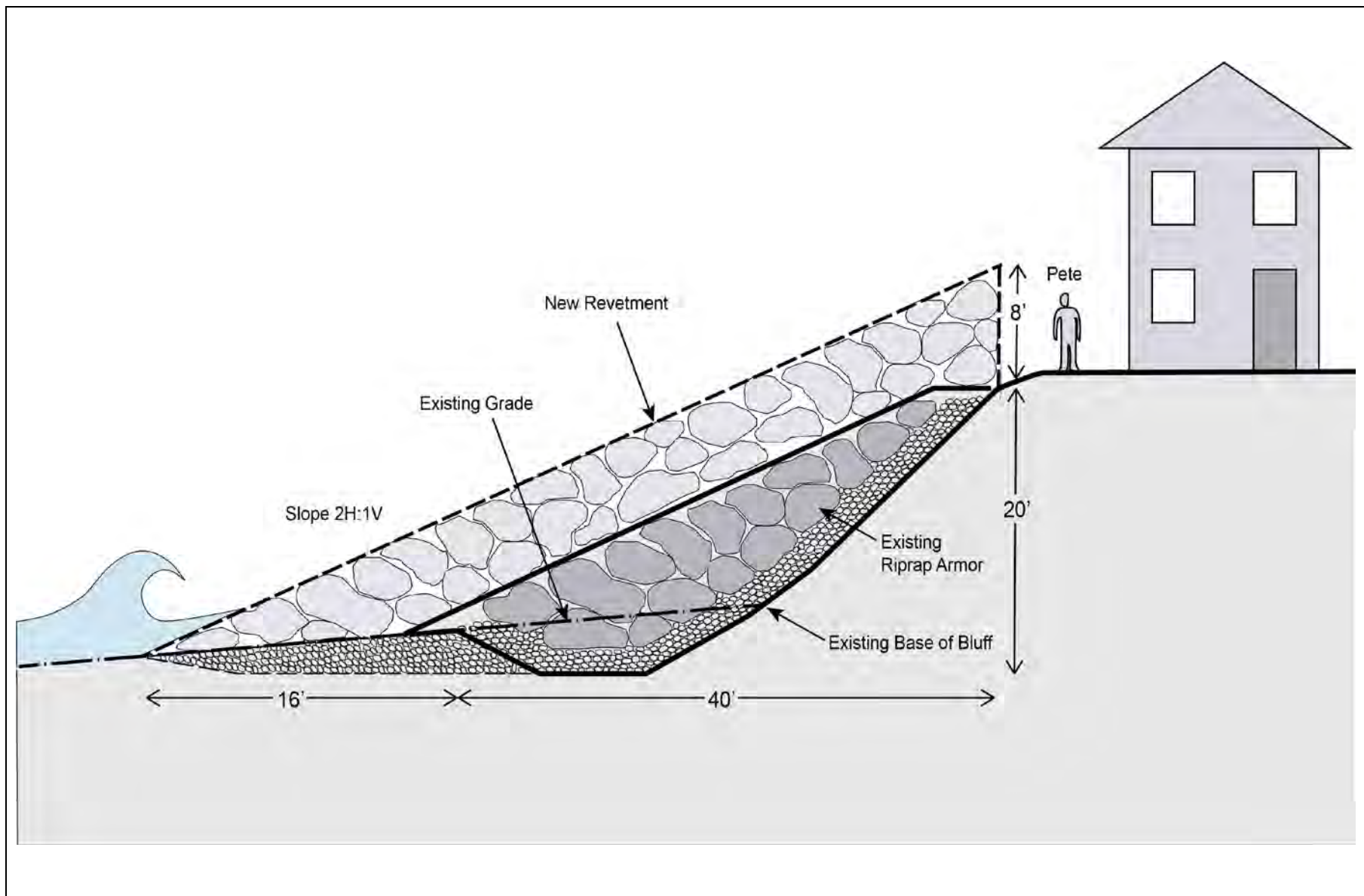
Figure 12 Conceptual Design for Expanded Revetment
