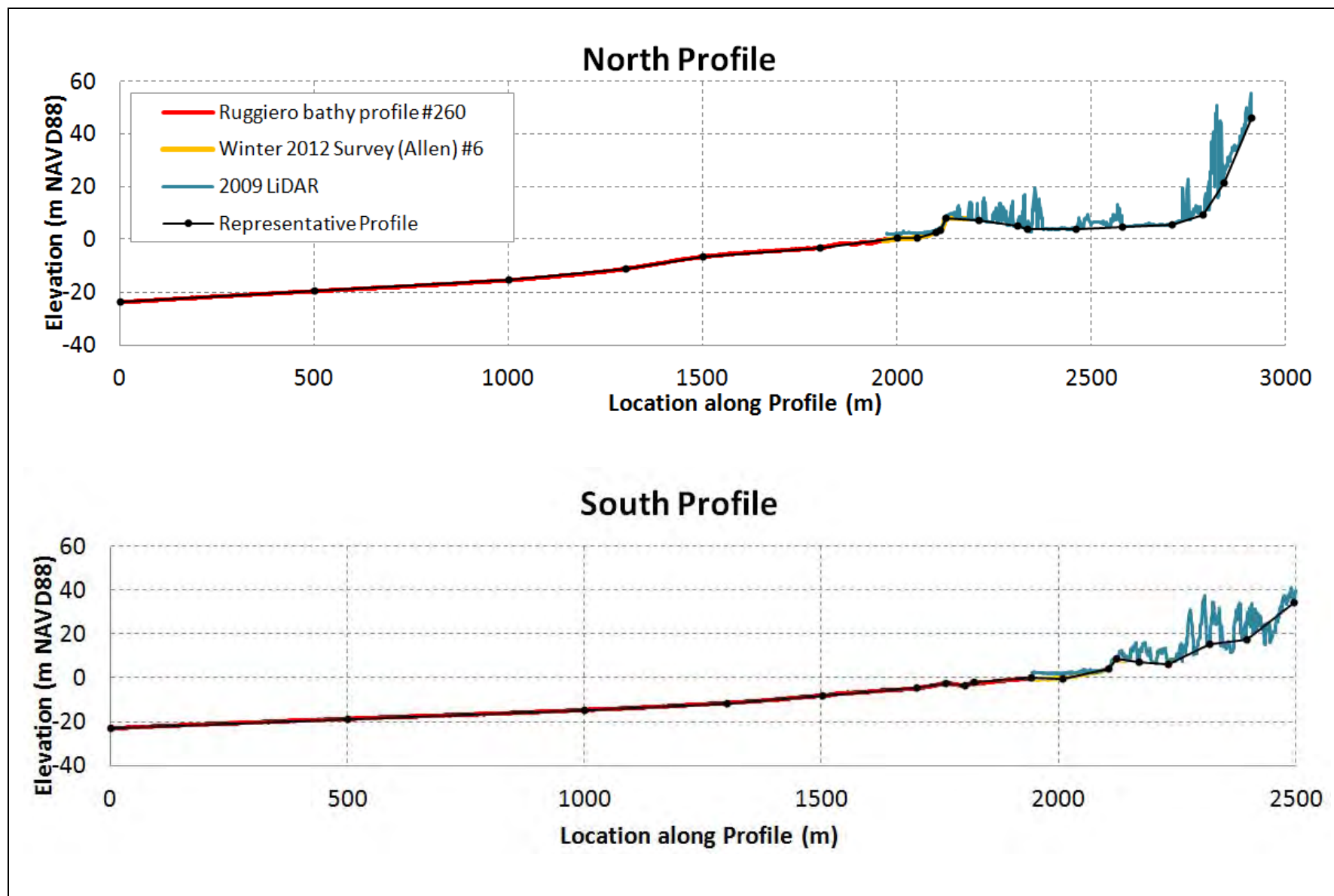
Figure 9 Representative Profiles for Composite Slope Analysis
