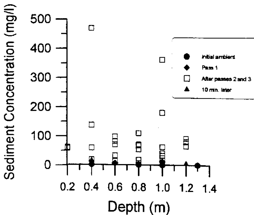
Figure 2. Change in suspended sediment concentration in the water column after up to three passes of a 200 hp dee-vee hull vessel. Water depth 1.5 m. 10 min after pass 3, sediment concentration approached pre-test levels.
