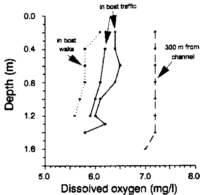
Figure 5. Depth profiles of dissolved oxygen concentration at several locations when numerous boats were being operated in Waquoit Bay. Concentrations were lowest in the navigation channel, particularly immediately after the passage of a boat (boat wake).
