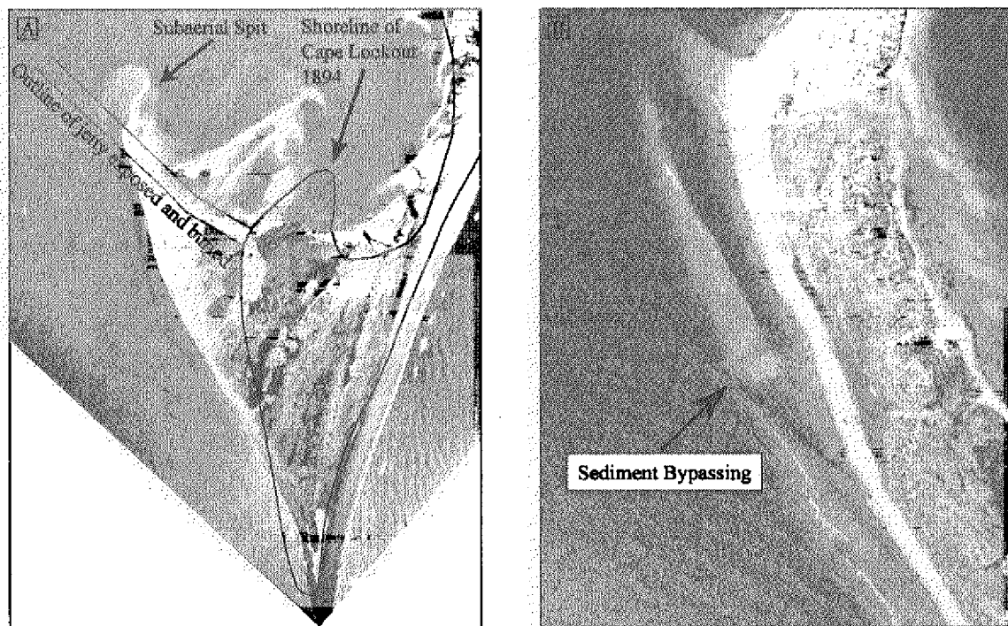
Figure 3. A: Aerial Photograph of Cape Lookout (1940) with 1894 shoreline and outline of exposed and buried portions of rock jetty. B: Aerial Photograph of the rock jetty at Cape Lookout (1996). Sediment readily bypasses jetty. At high tide jetty is awash, which was the intended design.
