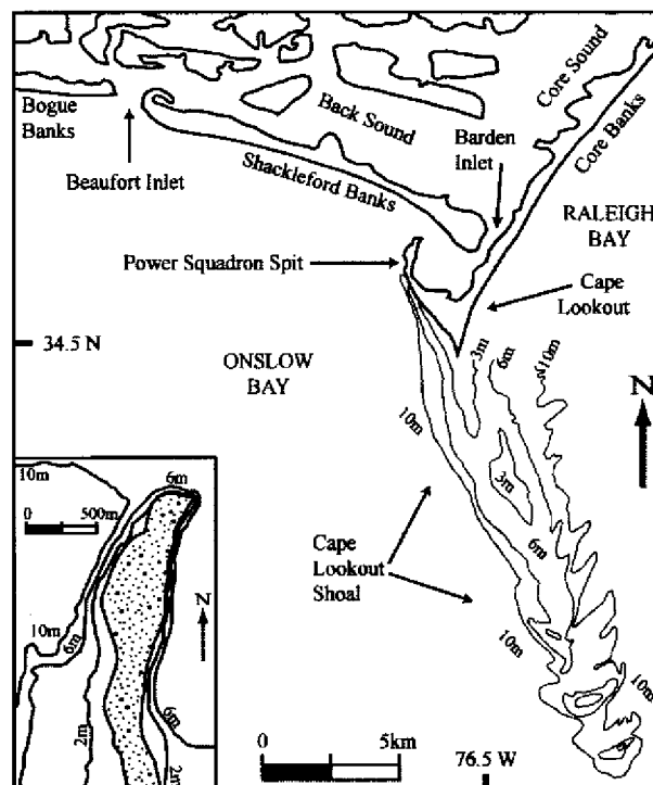
Figure 1. Cape Lookout, North Carolina and surrounding region, bathymetry of Cape Lookout Shoal after McNinch and Wells, (1999). Inset: shoreline and bathymetry of Power Squadron Spit.
