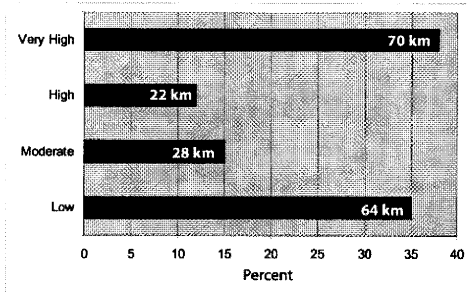
Figure 1. Histogram showing the percentage of each risk category within the Cape Cod National Seashore based on the CVI values of each shoreline segment. Shoreline lengths in each category are given in kilometers.
